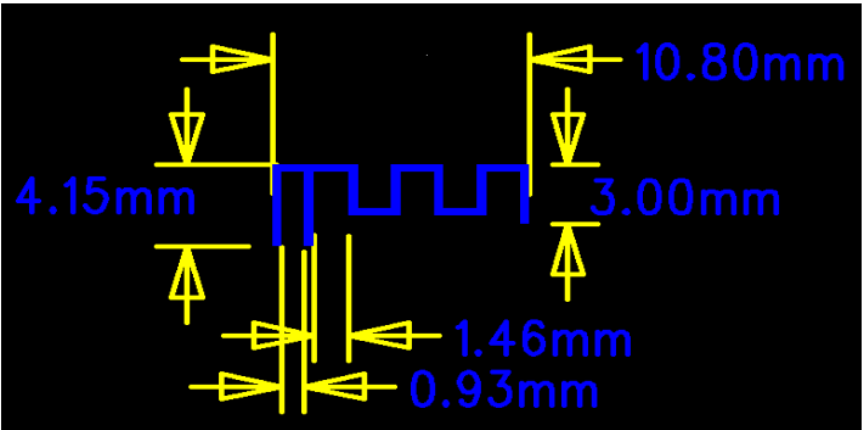
Antenna Photo & Length(mm)
