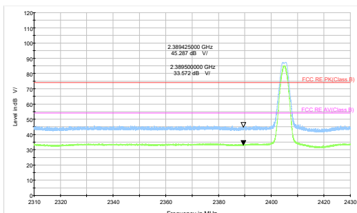
Zigbee Channel 11 Peak+ Average
