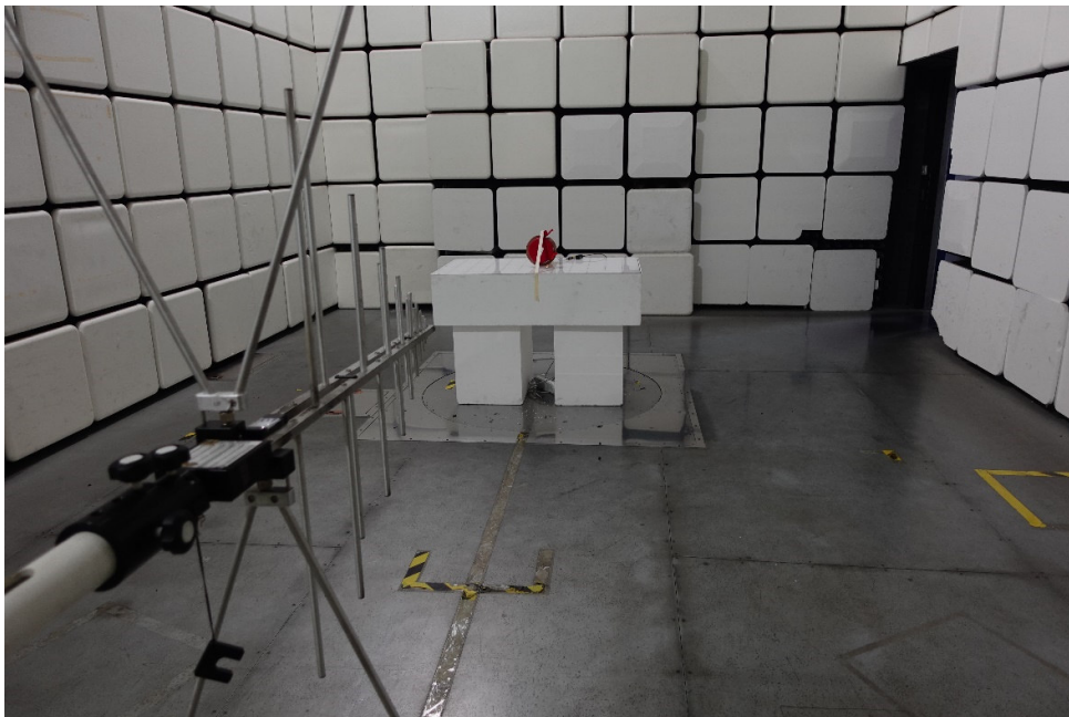
30MHz-1GHz
