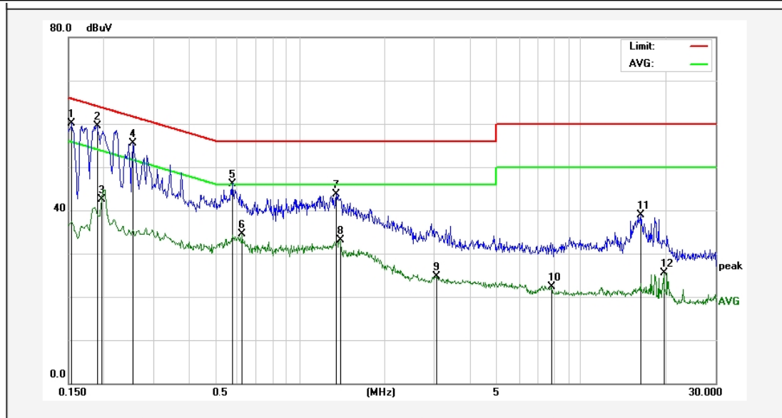
TM1 / Line: Neutral / Band: 2400-2483.5 MHz / BW: 1 / CH: H
