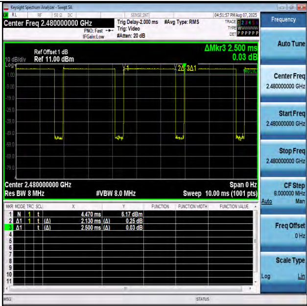
NTNV-BLE_1M-Ant1-2480
