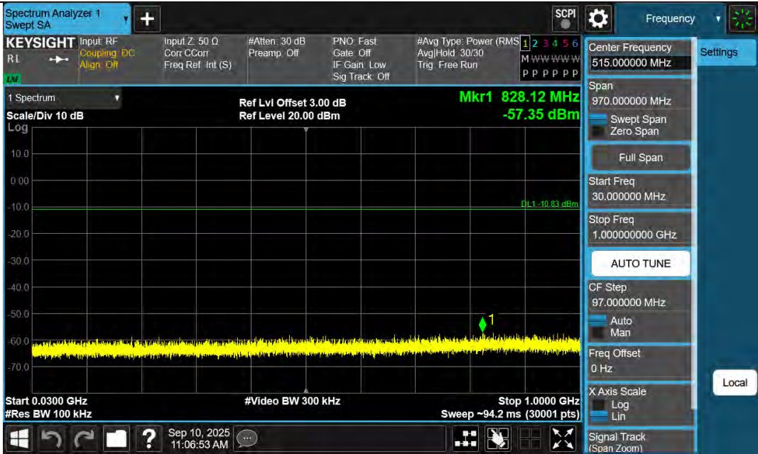
BLE_1M-Ant1-2480-30~1000-PASS
