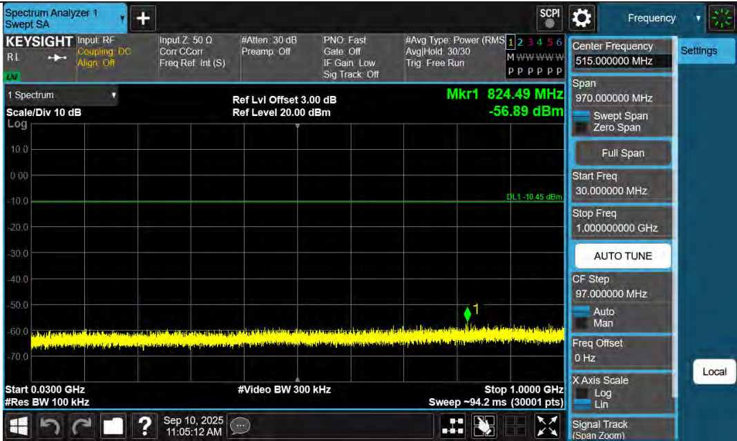
BLE_1M-Ant1-2440-30~1000-PASS
