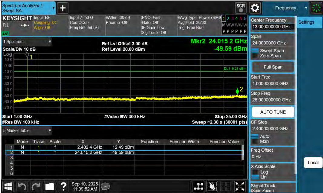
BLE_2M-Ant1-2402-1000~25000-PASS
