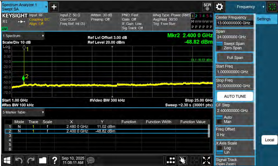
BLE_1M-Ant1-2480-1000~25000-PASS
