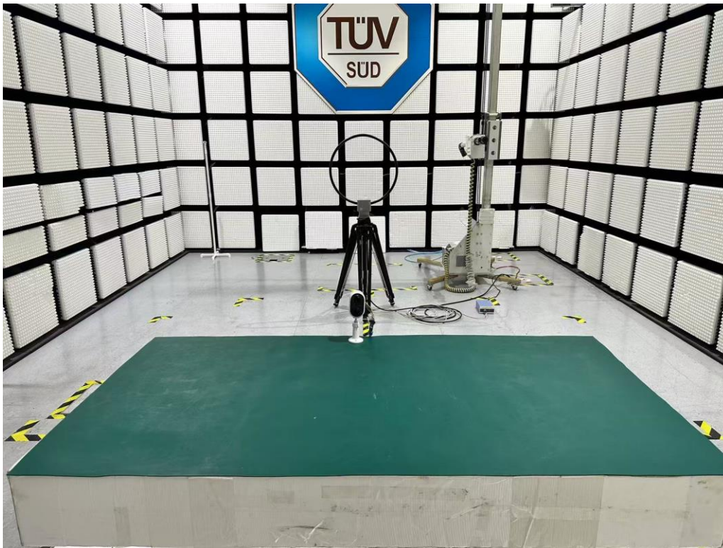
Radiated Emission Setup 9KHz-30MHz
