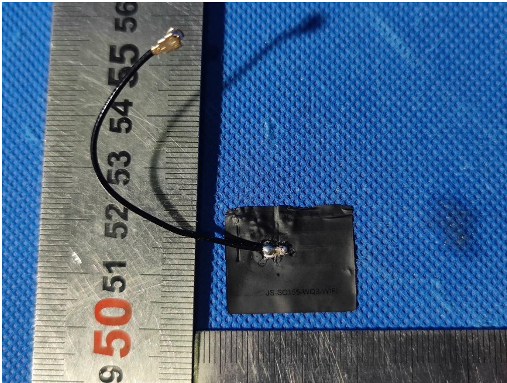
FPC Antenna
