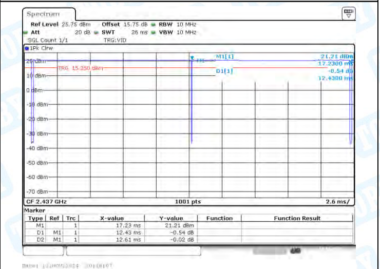
NTVN-11B-CDD-Ant2-2437
