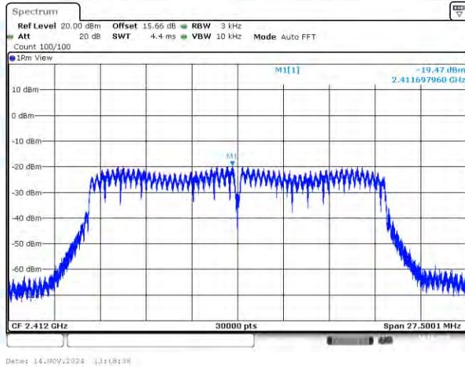
11N20MIMO-Ant1-2412-PASS
