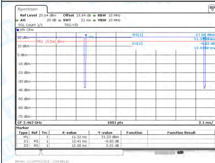
NTVN-11B-CDD-Ant1-2462
