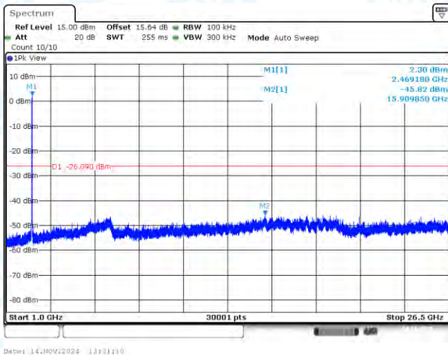
11N20MIMO-Ant1-2462-1000~26500-PASS
