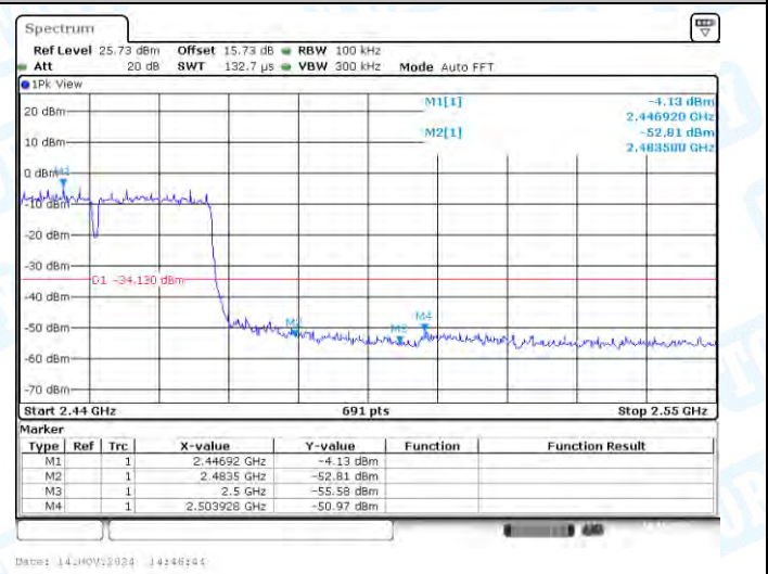
11N40MIMO-Ant2-2452-PASS
