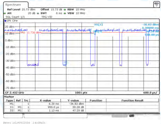
NTNV-11N40MIMO-Ant2-2452
