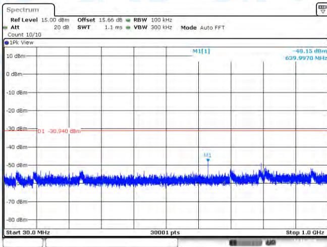
11N40MIMO-Ant1-2422-0~Reference-PASS
