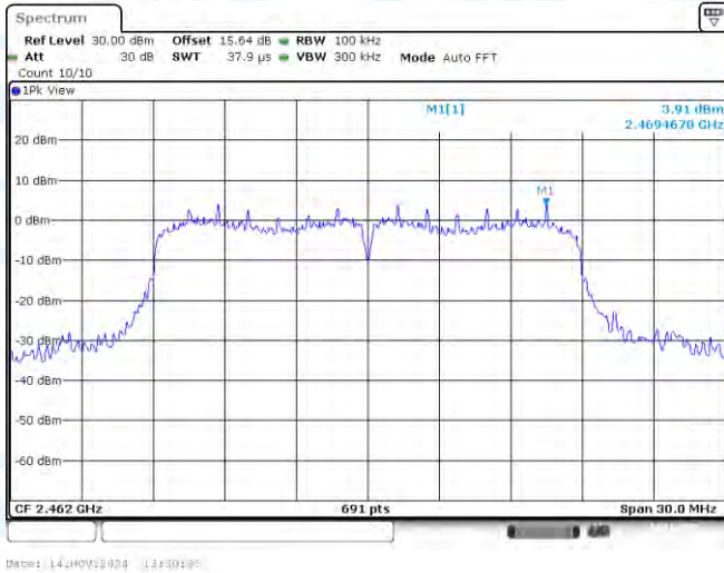
11N20MIMO-Ant1-2462-0~Reference-PASS
