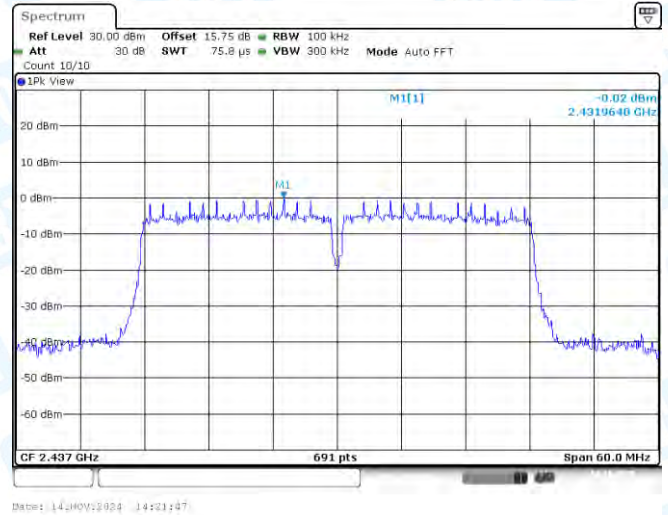
11N40MIMO-Ant2-2437-0~Reference-PASS
