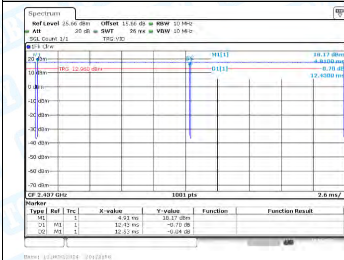
NTVN-11B-CDD-Ant1-2437
