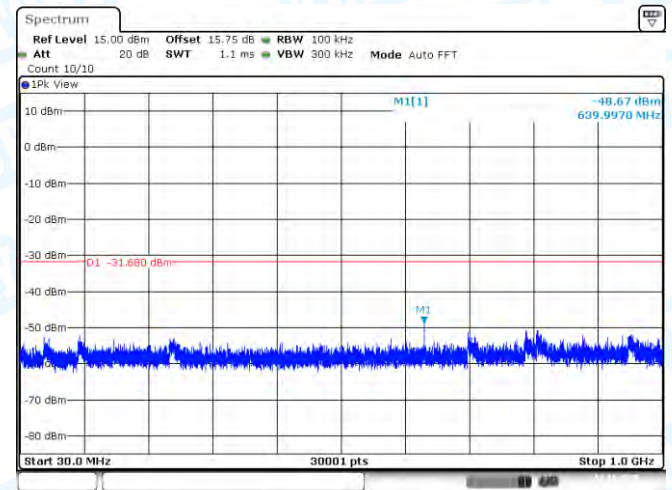
11N40MIMO-Ant2-2422-0~Reference-PASS
