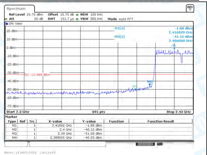
11N40MIMO-Ant2-2422-PASS
