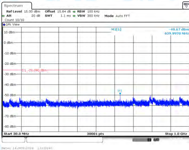
11N20MIMO-Ant1-2462-30~1000-PASS
