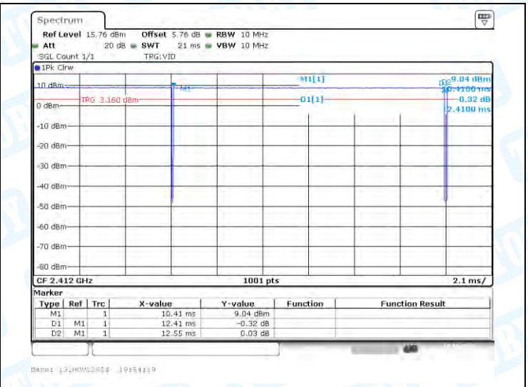
NTVN-11B-CDD-Ant2-2412
