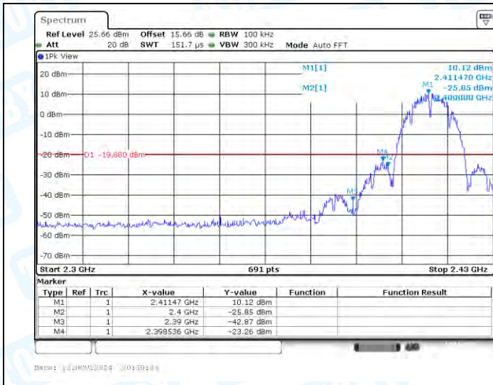
11B-CDD-Ant1-2412-PASS
