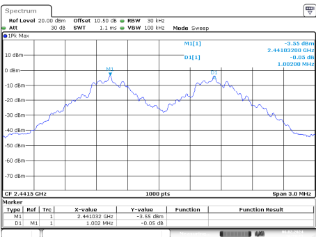
GFSK_Mid_DH1
