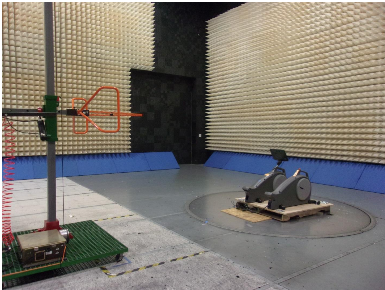
Unintentional radiated emissions and radiated spurious emissions, 30MHz – 1GHz
