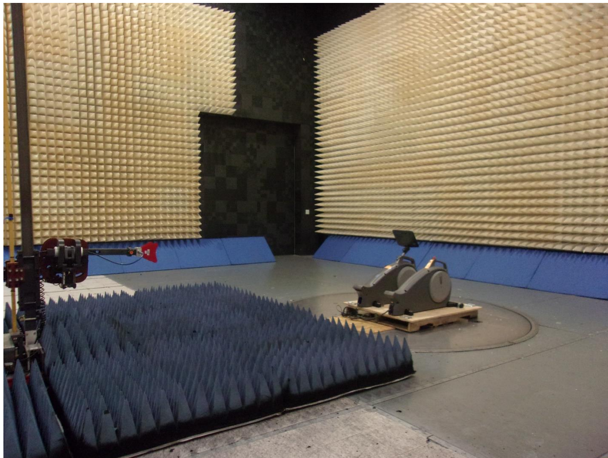
Unintentional emissions and radiated spurious emissions, 1GHz – 18GHz
