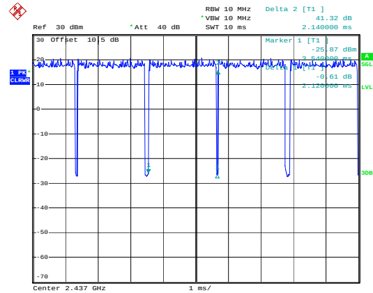
g_2437MHz_Chain 0
