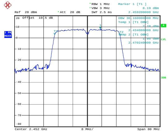
n40_2452MHz_Chain 0
