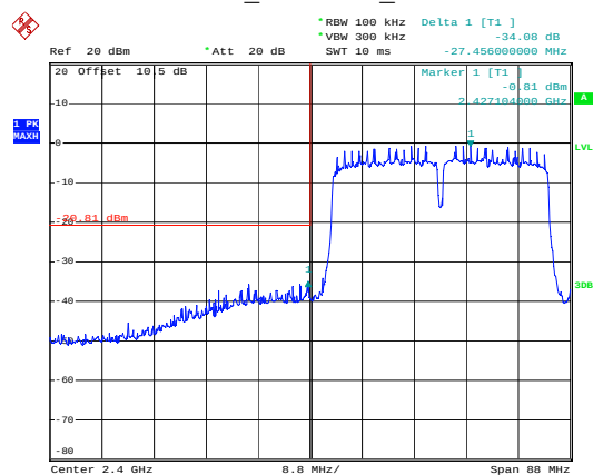
n40_2422MHz_Chain 0
