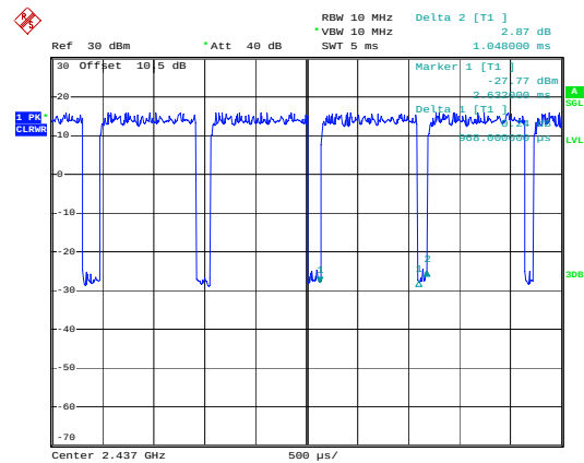
n40_2437MHz_Chain 0
