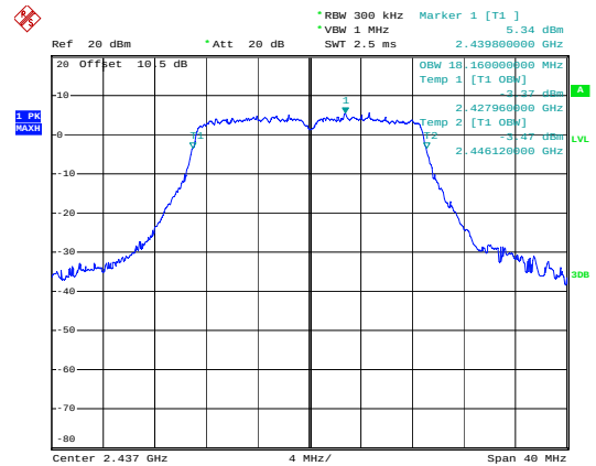
n20_2437MHz_Chain 0
