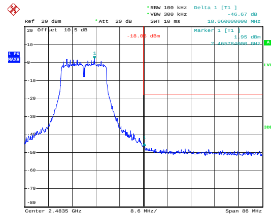
g_2462MHz_Chain 0
