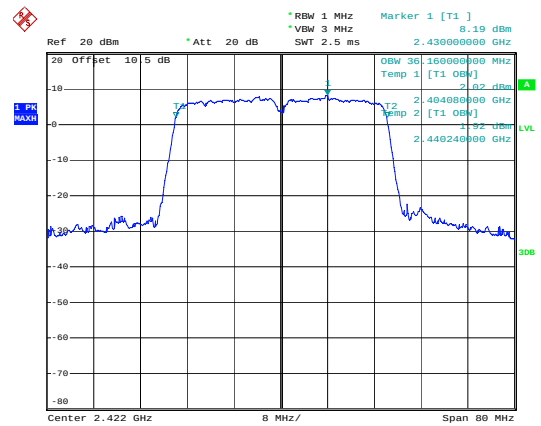
n40_2422MHz_Chain 0
