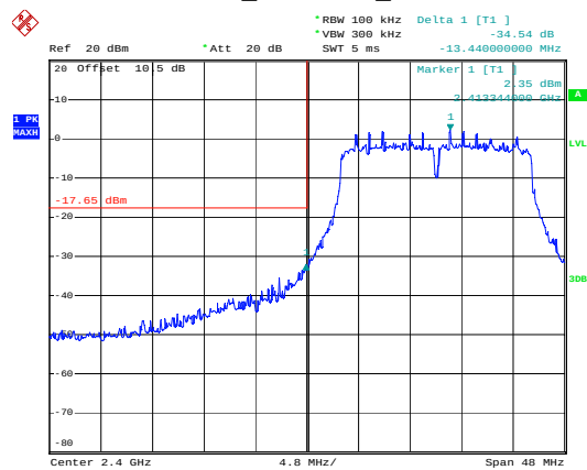
n20_2412MHz_Chain 0
