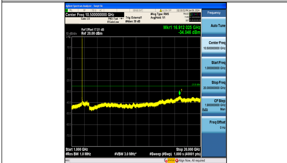
Band41_10MHz_QPSK_40290_50RB#0_1000~20000_1000~20000
