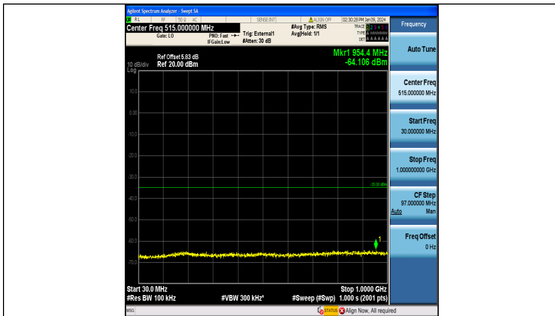
Band41_10MHz_QPSK_40290_50RB#0_30~1000_30~1000
