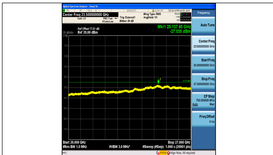
Band41_20MHz_QPSK_41140_100RB#0_20000~27000_20000~27000
