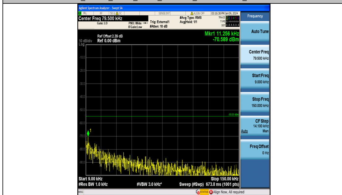
Band41_20MHz_16QAM_41140_100RB#0_0.009~0.15_0.009~0.15
