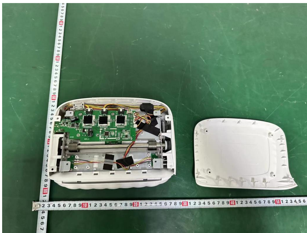
Internal photos M/N: SA501
