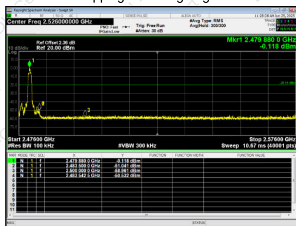
No-hopping Band edge-right side
