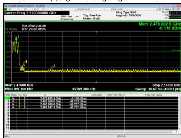
Hopping Band edge-right side
