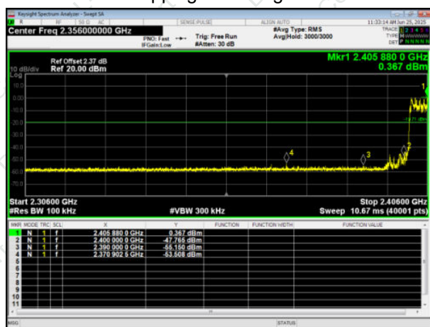
Hopping Band edge-left side
