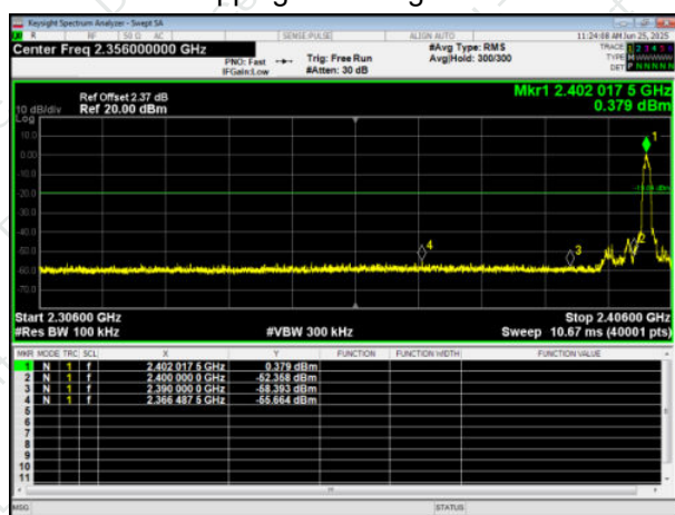
No-hopping Band edge-left side
