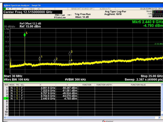
30.0 MHz - 25000.0 MHz π/4DQPSK 2-DH5 Channel 39
