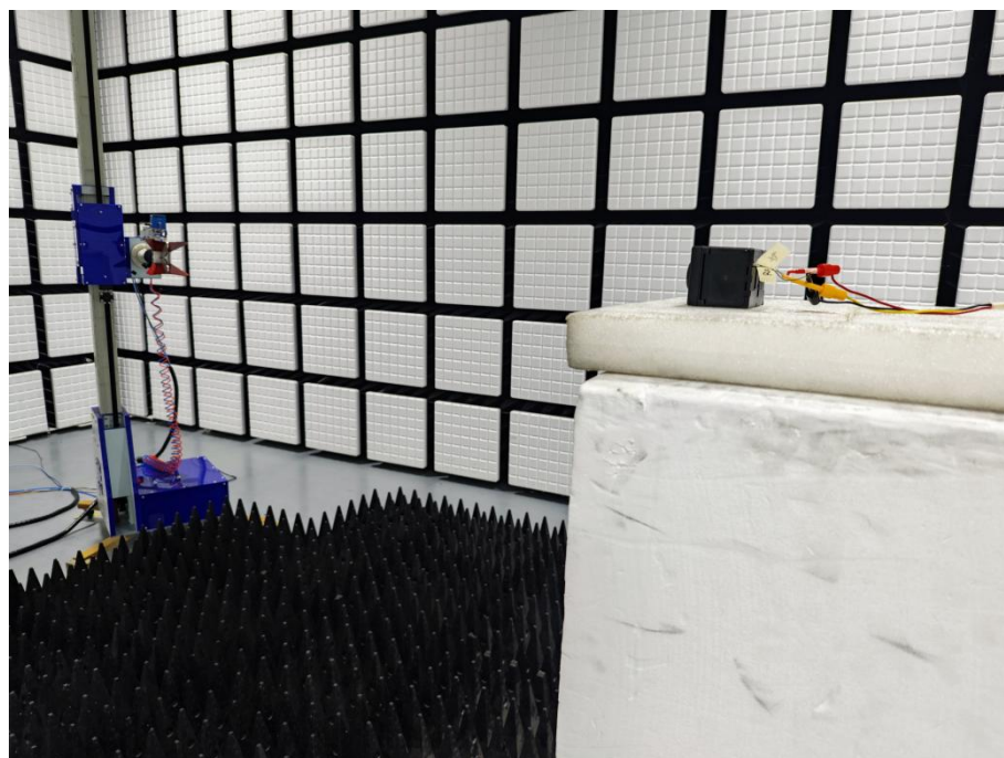
Description: Back view of Radiated Emission Test Setup (1GHz -18GHz) BLE Test
