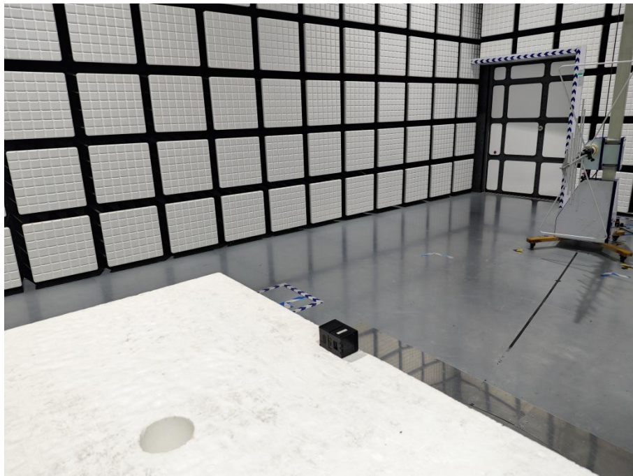
Description: Back view of Radiated Emission Test Setup (30MHz -1000MHz) WIFI Test
