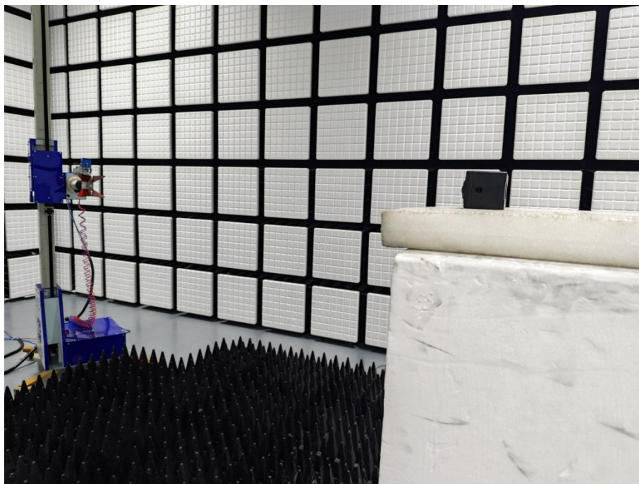
Description: Back view of Radiated Emission Test Setup (1GHz -18GHz) WIFI Test
