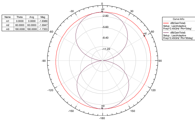
1-3 PIFA C Type antenna 2D gain chart
