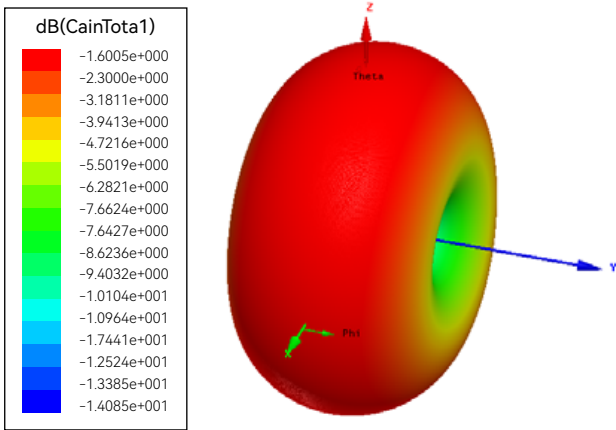
1-4 PIFA C Type antenna 3D gain chart
