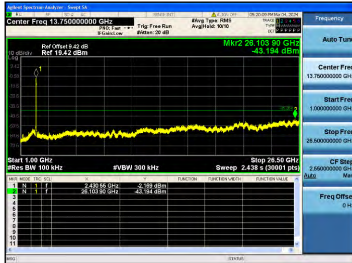
11AX40SISO_Ant1_2452_0~Reference
