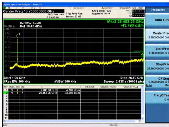
11AX40SISO_Ant1_2437_0~Reference
