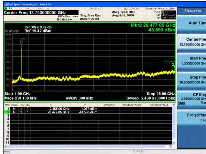
11AX40SISO_Ant1_2422_0~Reference
