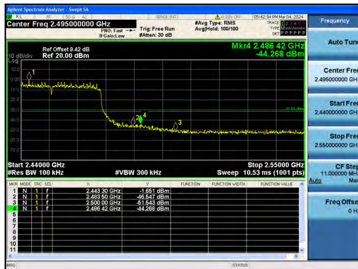
11AX40SISO_Ant1_High_2452
