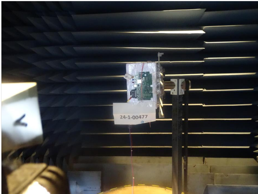
Photograph 7: EUT test setup in the fully anechoic chamber 2, overview_EUT elevation 90°
