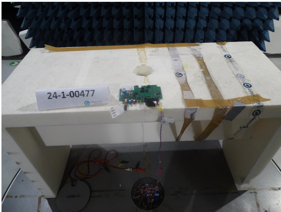
Photograph 8: EUT test setup in the semi anechoic chamber, close up view_EUT elevation 0°
