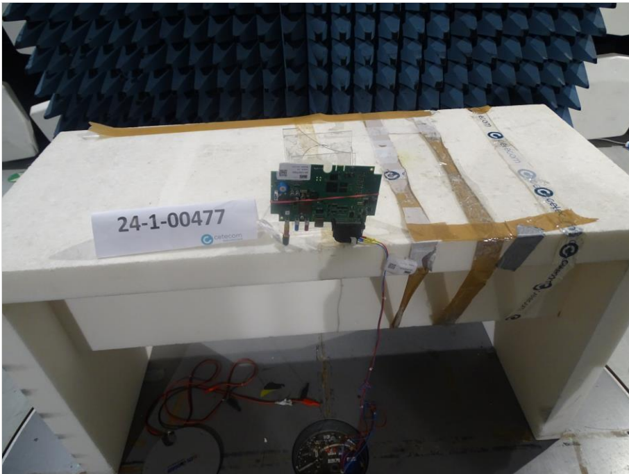
Photograph 10: EUT test setup in the semi anechoic chamber, close up view_EUT elevation 90°
