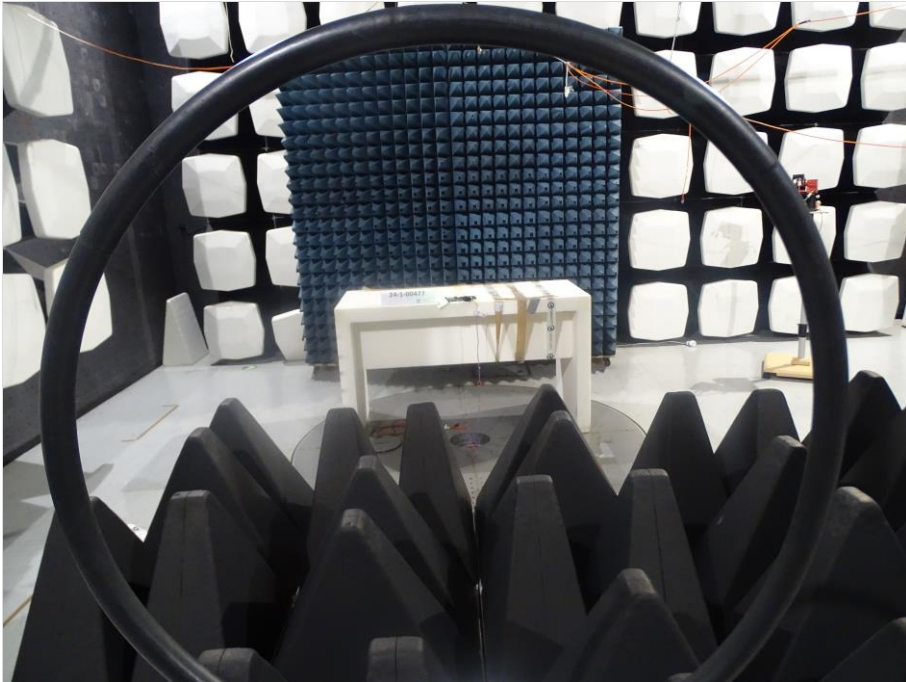
Photograph 9: EUT test setup in the semi anechoic chamber, overview_EUT elevation 0°
