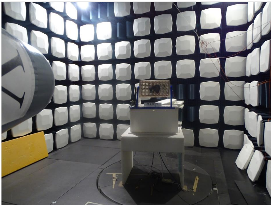
Photograph 6: EUT test setup in the fully anechoic chamber, overview_EUT elevation 90°
