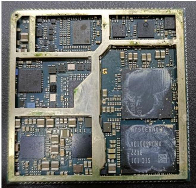
Main Board Photo Rear – Shield removed
