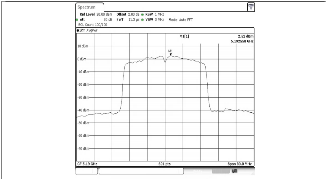
11AC40SISO-Ant1-5190-PASS
