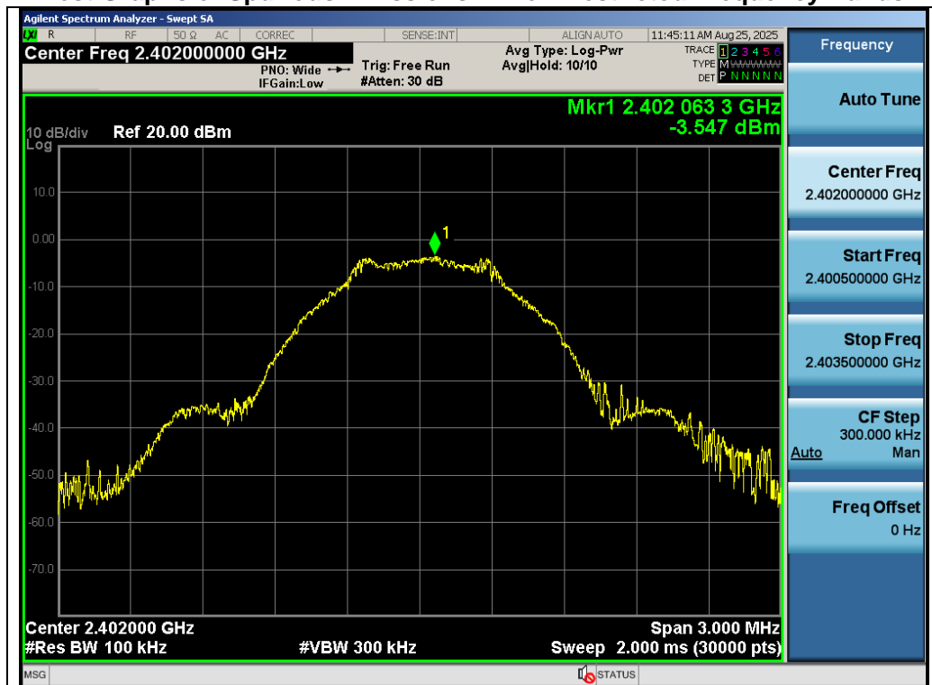
Test_Graph_SRD_ANT1_2402_2.4G_Reference Level
