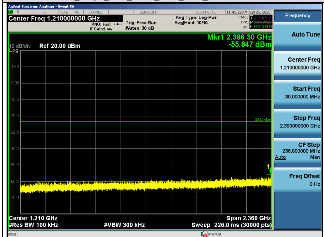
Test_Graph_SRD_ANT1_2402_2.4G_Lower Band Emissions
