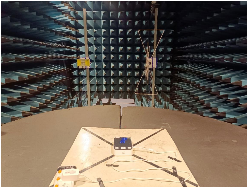
Radiated Emission 1 GHz -18GHz -Front
