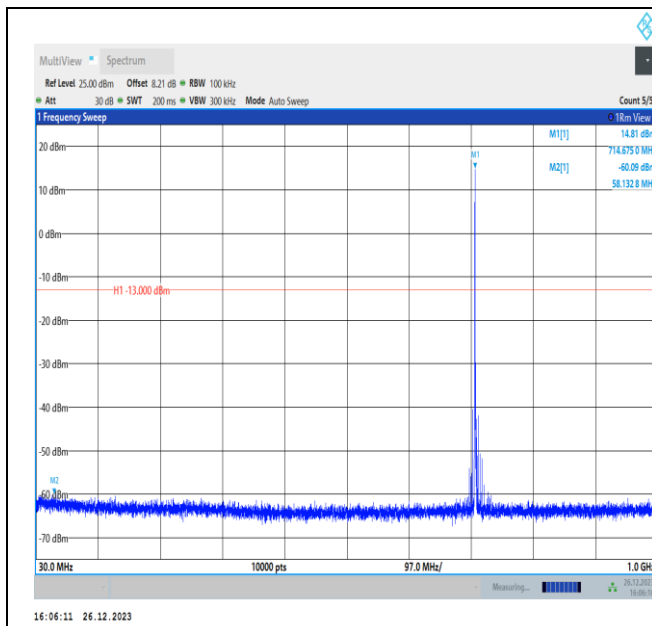
Band12-5MHz-QPSK-23155-PASS
