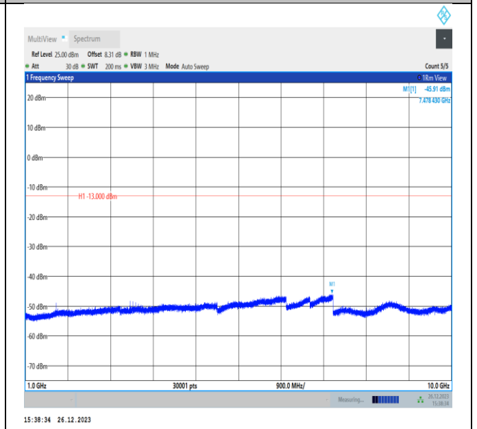
Band5-10MHz-QPSK-20450-PASS
