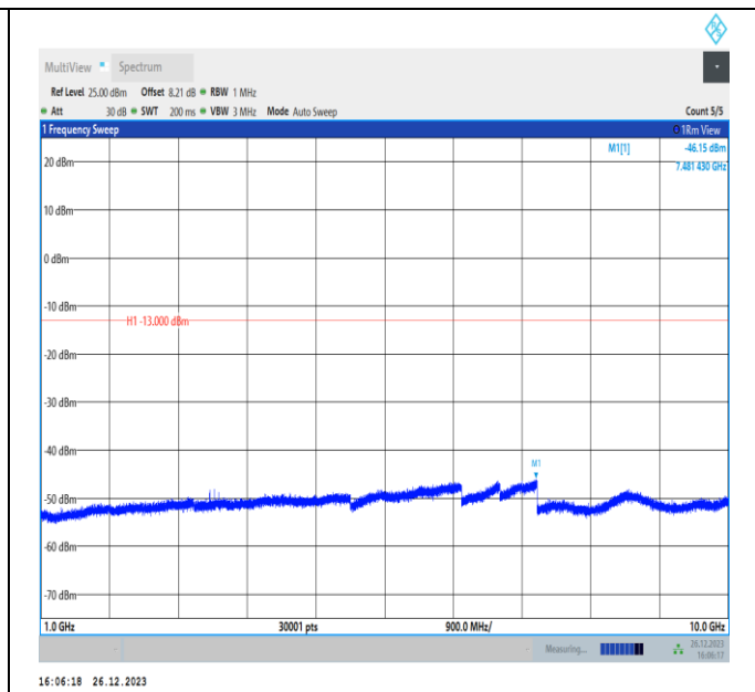
Band12-5MHz-QPSK-23155-PASS
