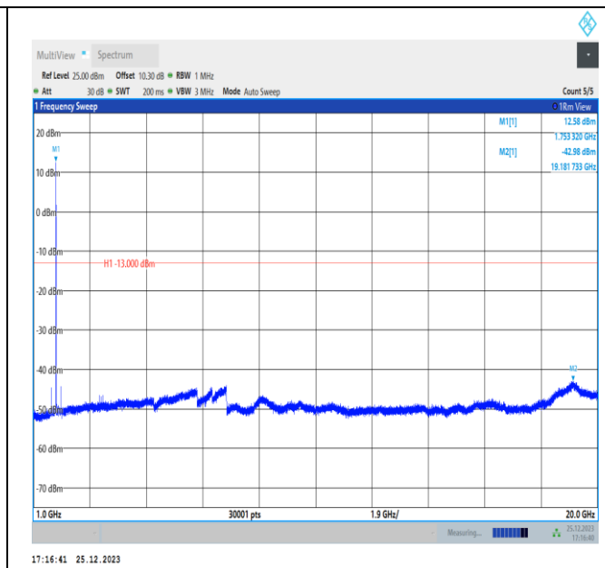
Band4-15MHz-QPSK-20325-PASS
