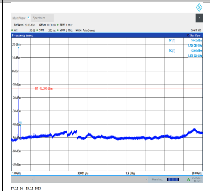
Band4-15MHz-QPSK-20175-PASS
