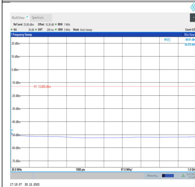
Band4-15MHz-QPSK-20175-PASS
