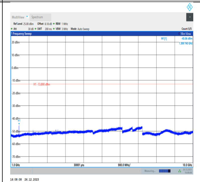
Band12-10MHz-QPSK-23060-PASS
