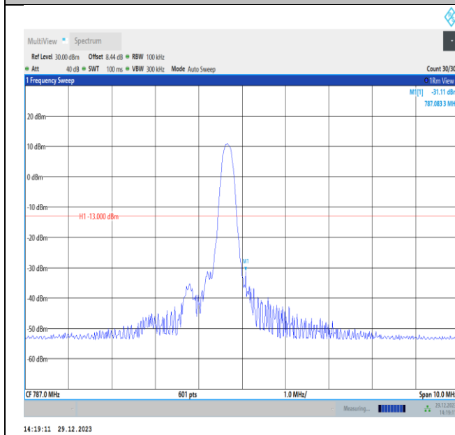
Band13-5MHz-16QAM-23255-PASS
