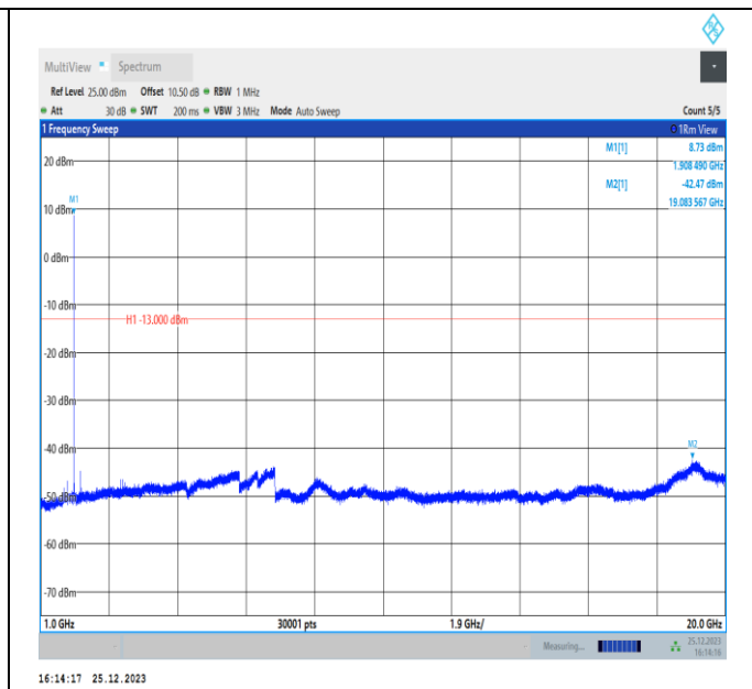
Band2-1.4MHz-QPSK-19193-PASS
