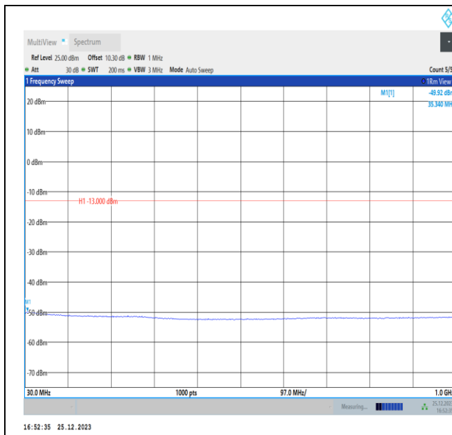
Band4-3MHz-QPSK-20175-PASS
