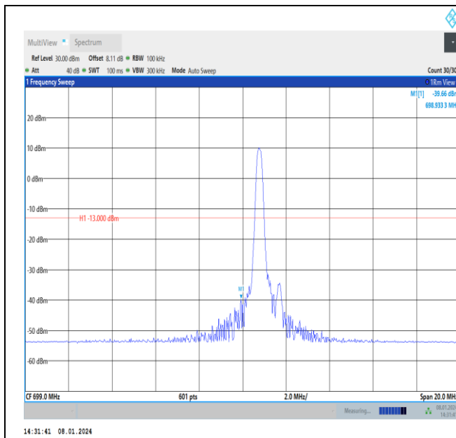
Band12-10MHz-16QAM-23060-PASS
