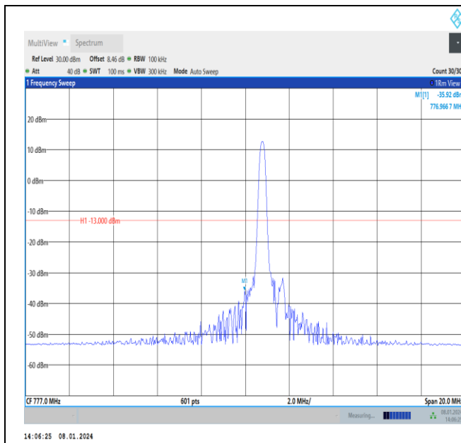
Band13-10MHz-QPSK-23230-PASS
