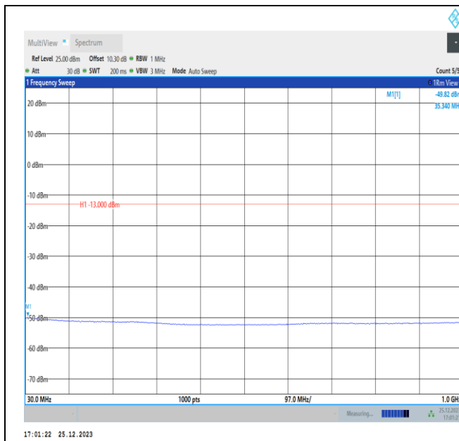
Band4-5MHz-QPSK-20375-PASS
