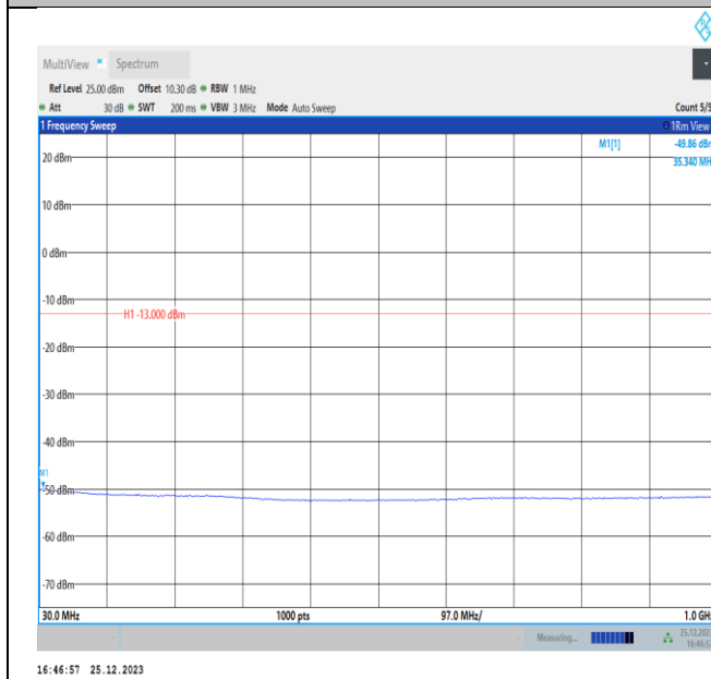
Band4-1.4MHz-QPSK-20175-PASS
