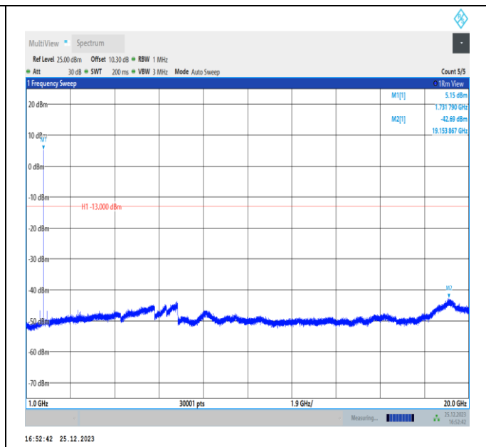
Band4-3MHz-QPSK-20175-PASS
