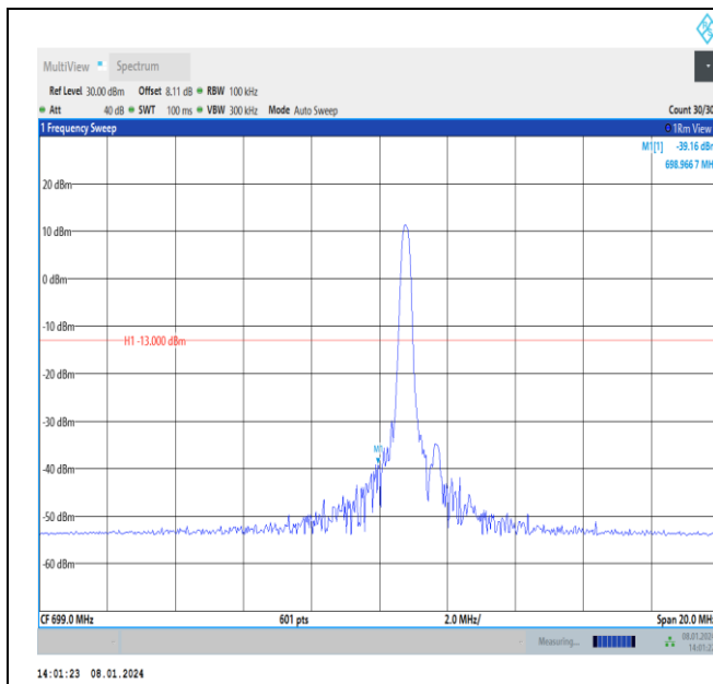
Band12-10MHz-QPSK-23060-PASS
