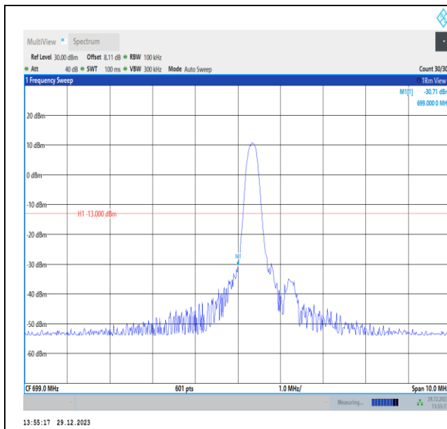
Band12-5MHz-16QAM-23035-PASS
