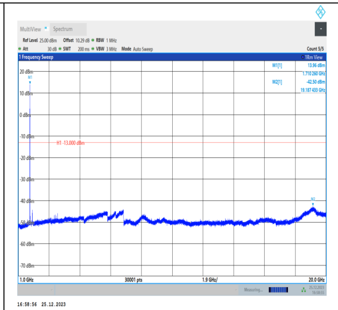
Band4-5MHz-QPSK-19975-PASS
