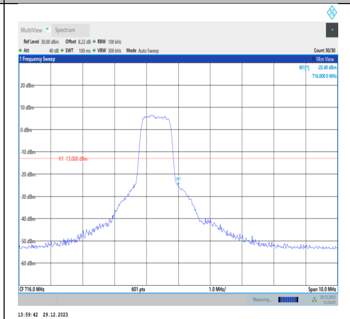
Band12-5MHz-16QAM-23155-PASS
