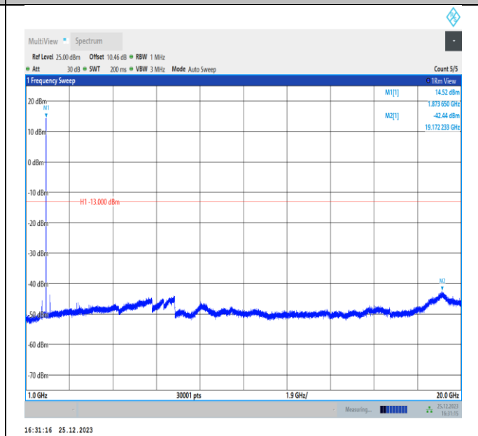
Band2-15MHz-QPSK-18900-PASS
