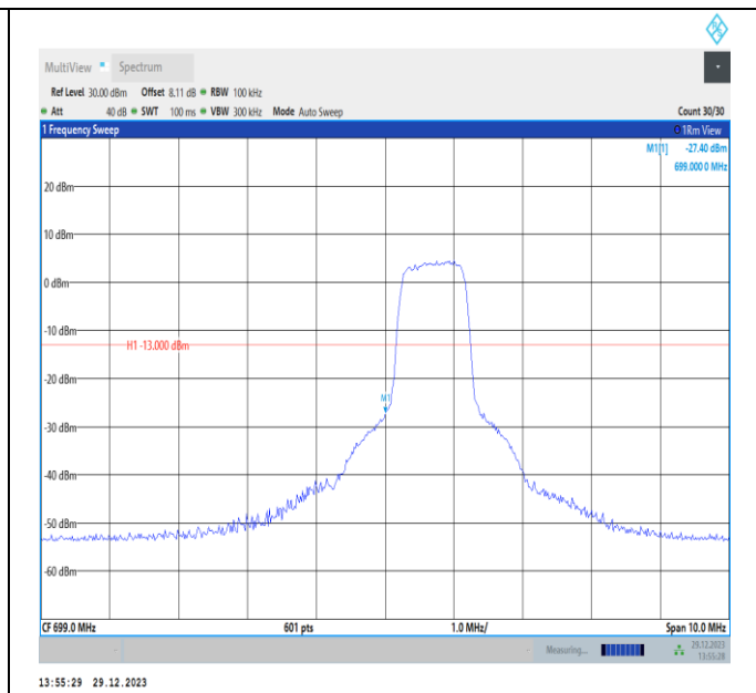
Band12-5MHz-16QAM-23035-PASS
