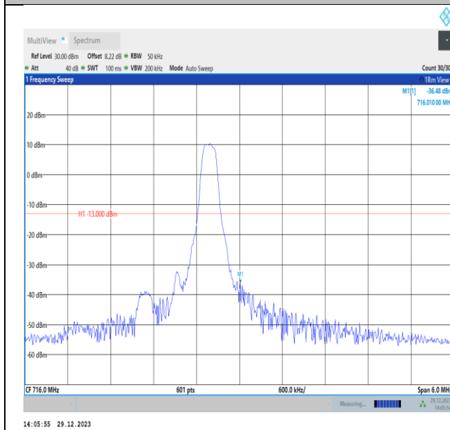
Band12-3MHz-16QAM-23165-PASS
