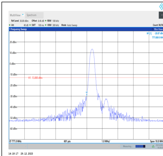
Band13-5MHz-16QAM-23205-PASS
