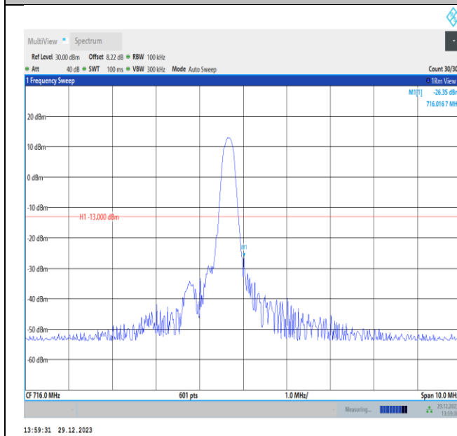
Band12-5MHz-16QAM-23155-PASS
