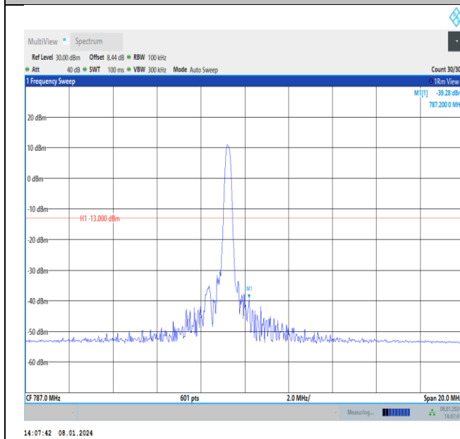
Band13-10MHz-QPSK-23230-PASS
