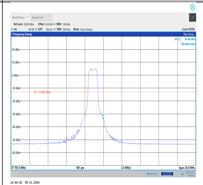
Band13-10MHz-16QAM-23230-PASS
