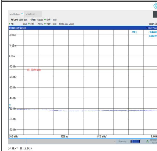
Band4-3MHz-QPSK-20385-PASS
