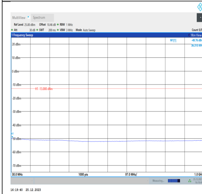
Band2-5MHz-QPSK-18900-PASS
