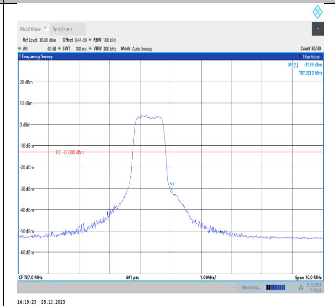
Band13-5MHz-16QAM-23255-PASS
