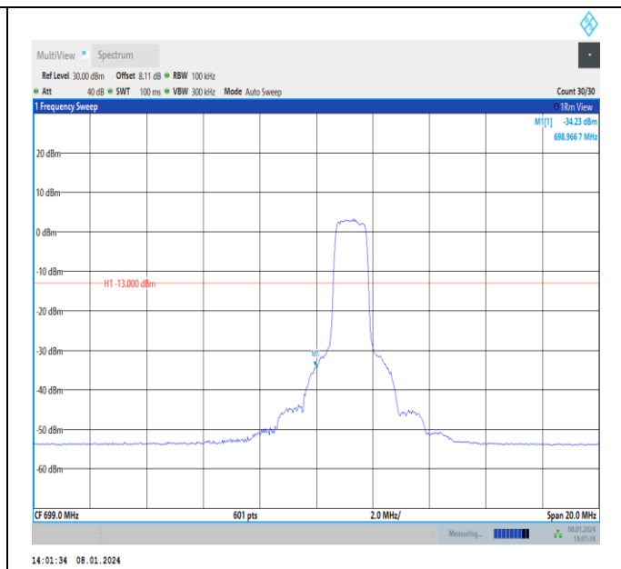
Band12-10MHz-QPSK-23060-PASS
