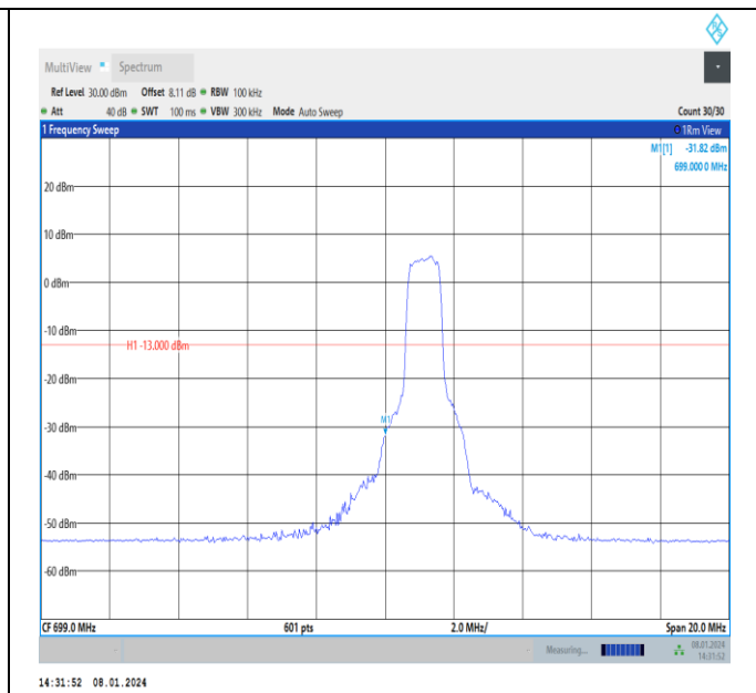
Band12-10MHz-16QAM-23060-PASS
