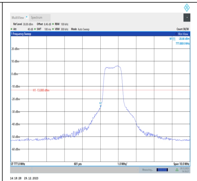
Band13-5MHz-16QAM-23205-PASS
