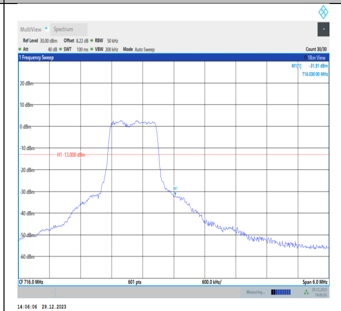
Band12-3MHz-16QAM-23165-PASS
