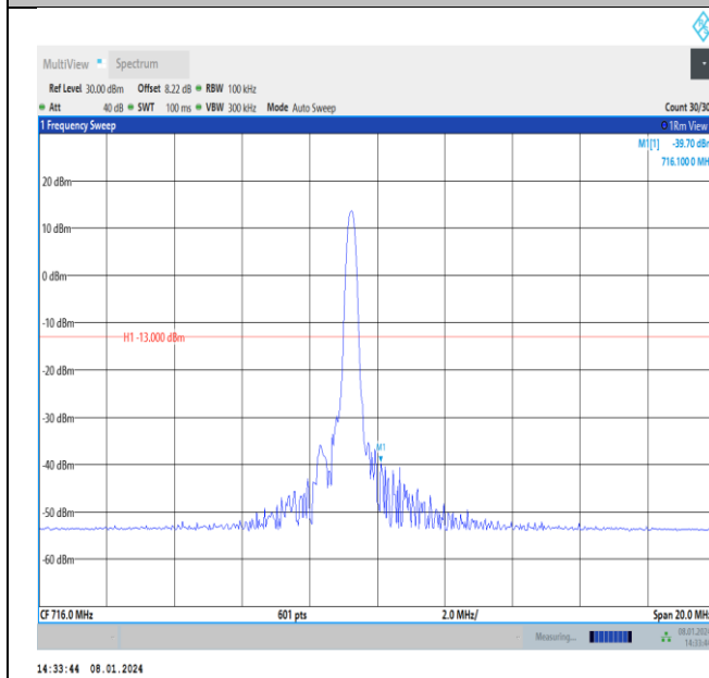
Band12-10MHz-16QAM-23130-PASS
