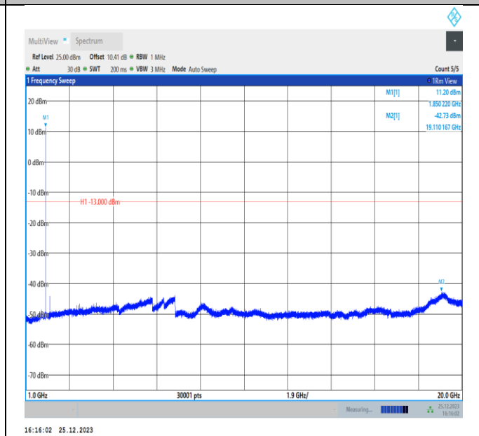
Band2-3MHz-QPSK-18615-PASS
