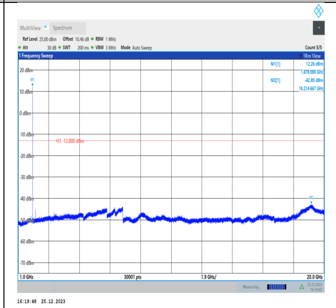
Band2-5MHz-QPSK-18900-PASS
