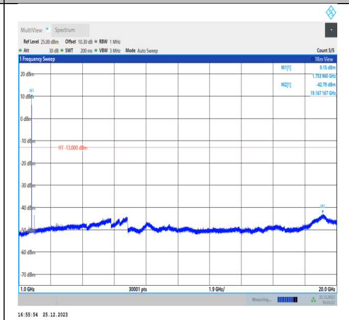
Band4-3MHz-QPSK-20385-PASS
