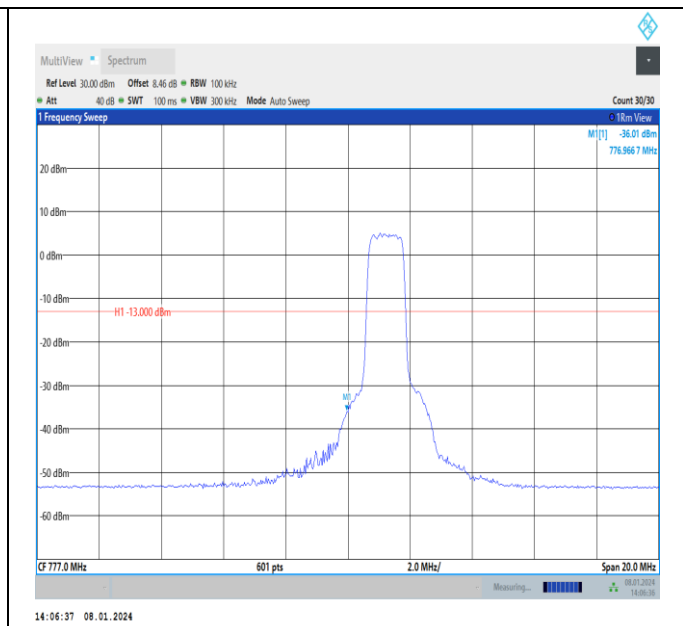
Band13-10MHz-QPSK-23230-PASS
