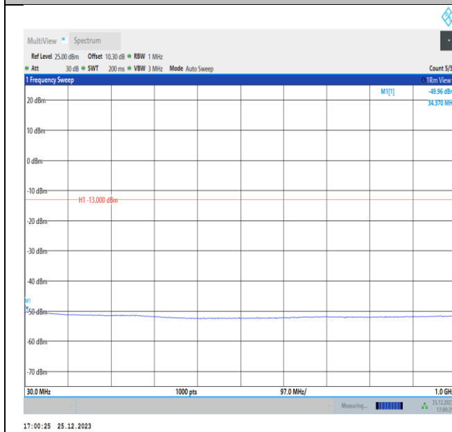
Band4-5MHz-QPSK-20175-PASS
