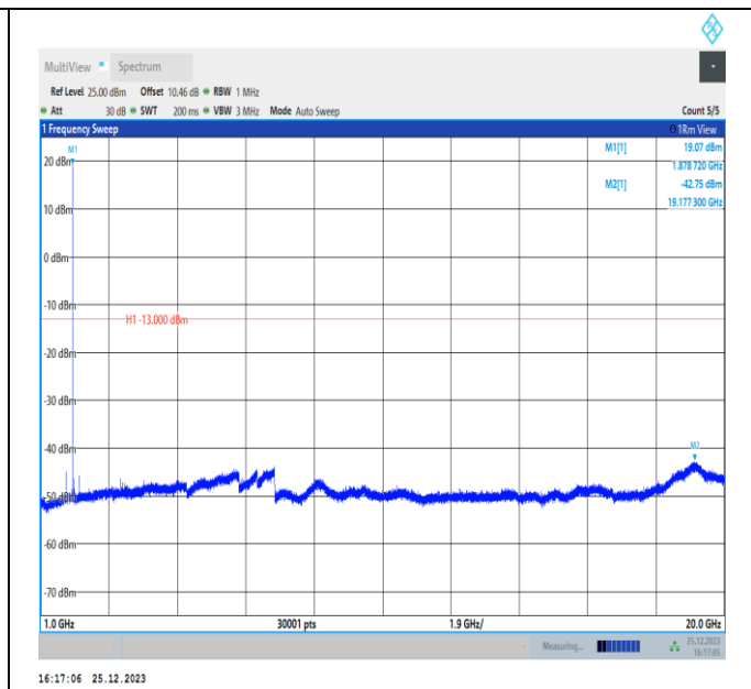
Band2-3MHz-QPSK-18900-PASS
