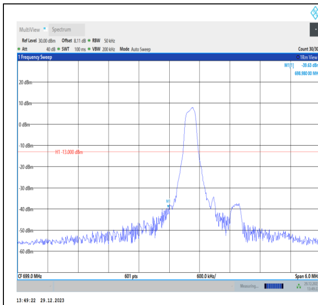
Band12-3MHz-16QAM-23025-PASS
