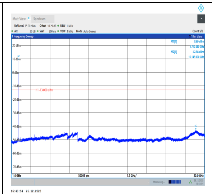
Band4-1.4MHz-QPSK-19957-PASS
