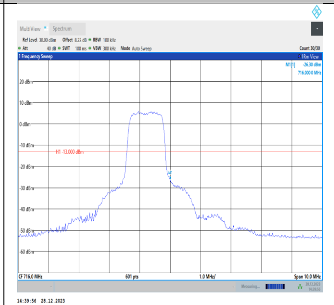
Band12-5MHz-QPSK-23155-PASS
