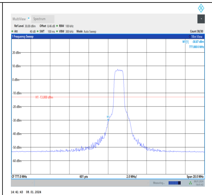
Band13-10MHz-16QAM-23230-PASS
