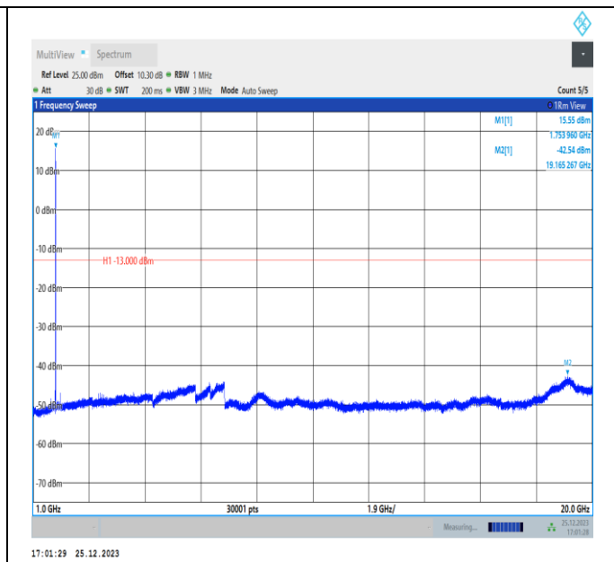
Band4-5MHz-QPSK-20375-PASS
