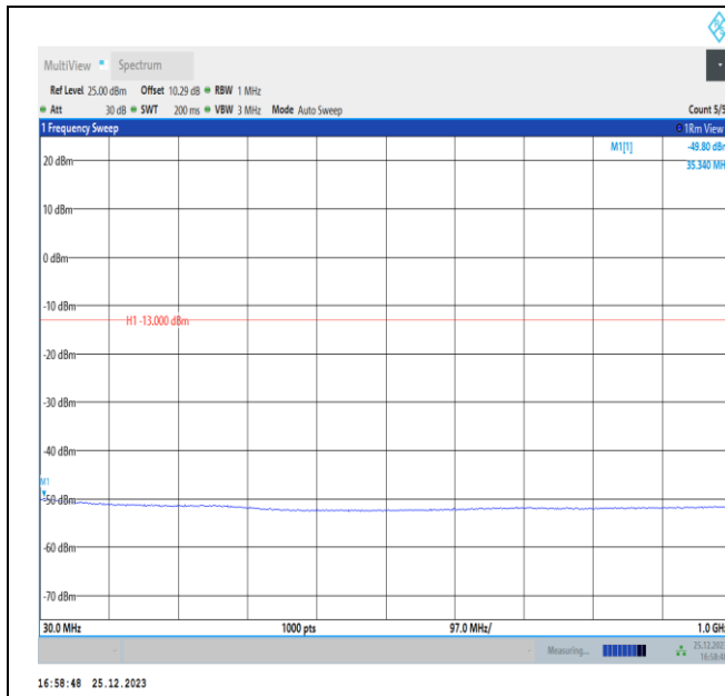
Band4-5MHz-QPSK-19975-PASS
