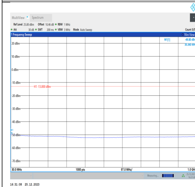
Band2-15MHz-QPSK-18900-PASS
