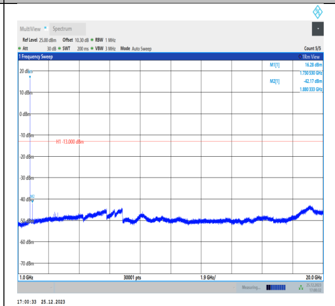
Band4-5MHz-QPSK-20175-PASS
