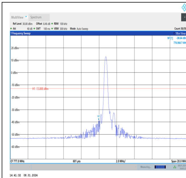
Band13-10MHz-16QAM-23230-PASS
