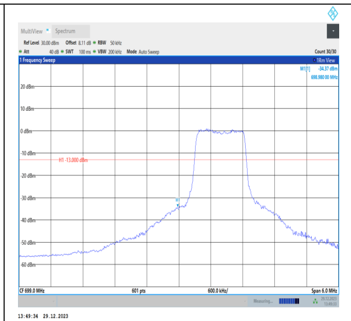
Band12-3MHz-16QAM-23025-PASS
