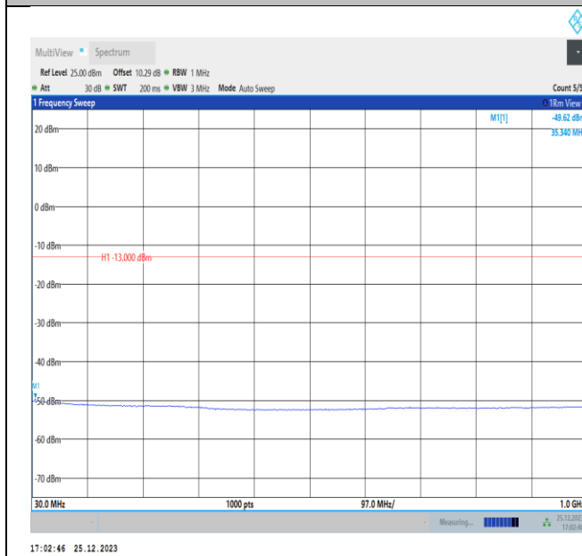
Band4-10MHz-QPSK-20000-PASS
