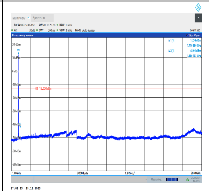
Band4-10MHz-QPSK-20000-PASS
