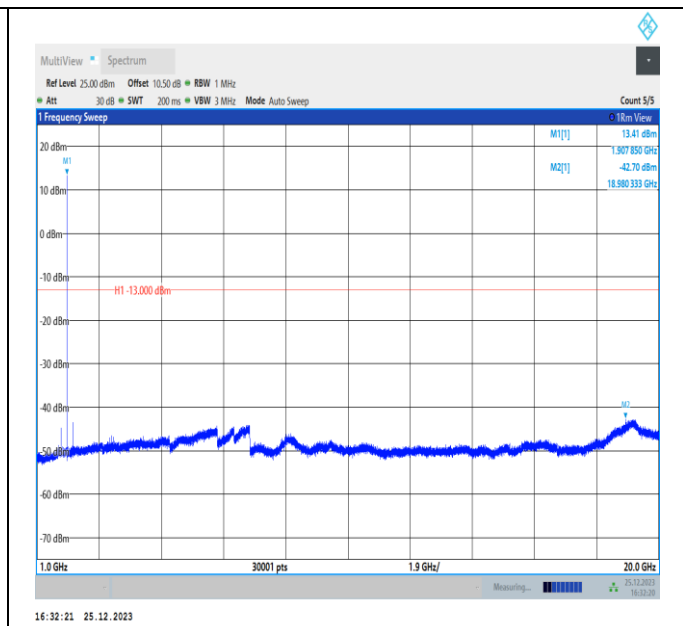
Band2-15MHz-QPSK-19125-PASS
