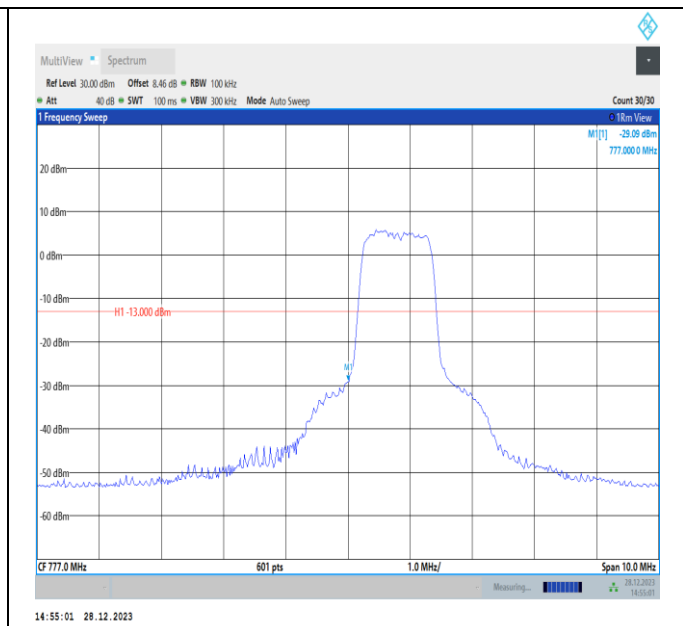
Band13-5MHz-QPSK-23205-PASS
