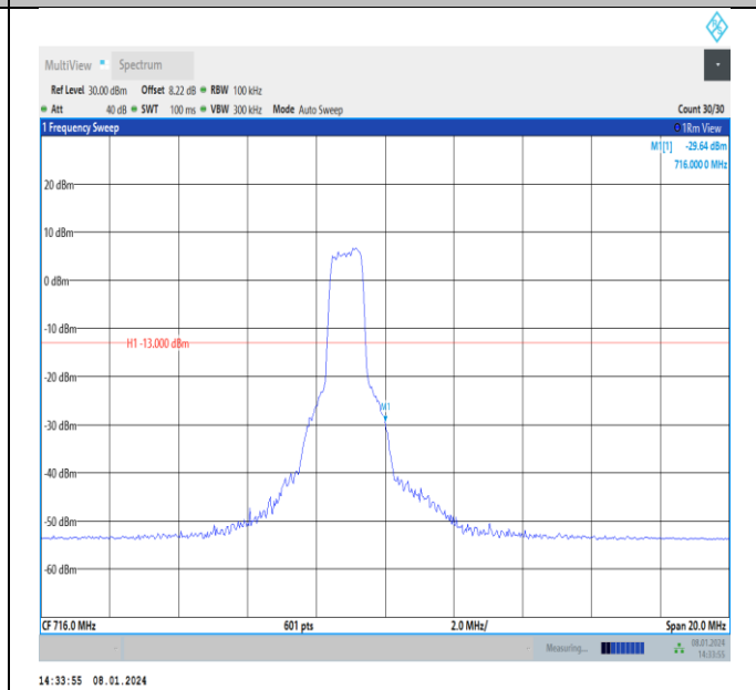
Band12-10MHz-16QAM-23130-PASS
