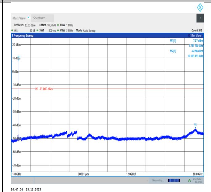
Band4-1.4MHz-QPSK-20175-PASS
