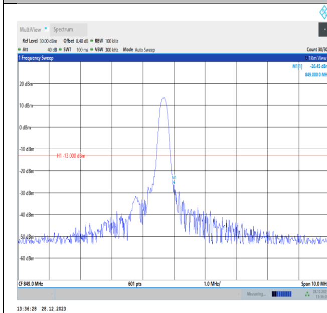
Band5-5MHz-QPSK-20625-PASS
