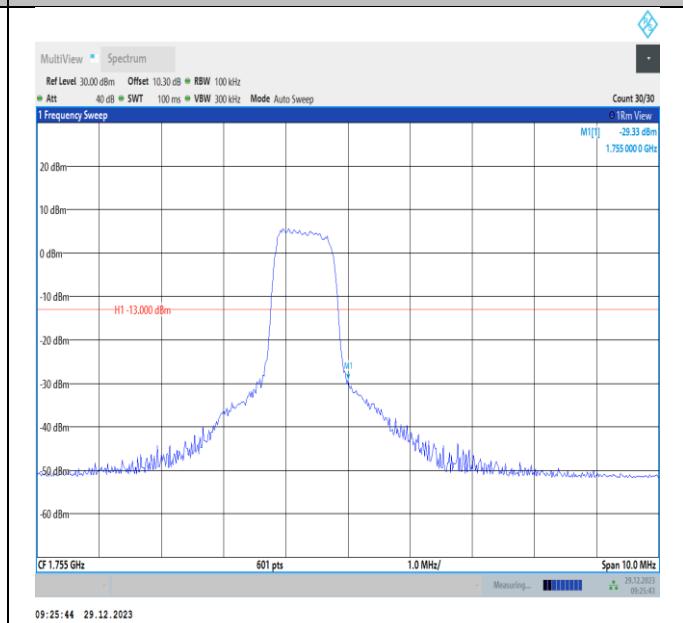
Band4-5MHz-16QAM-20375-PASS
