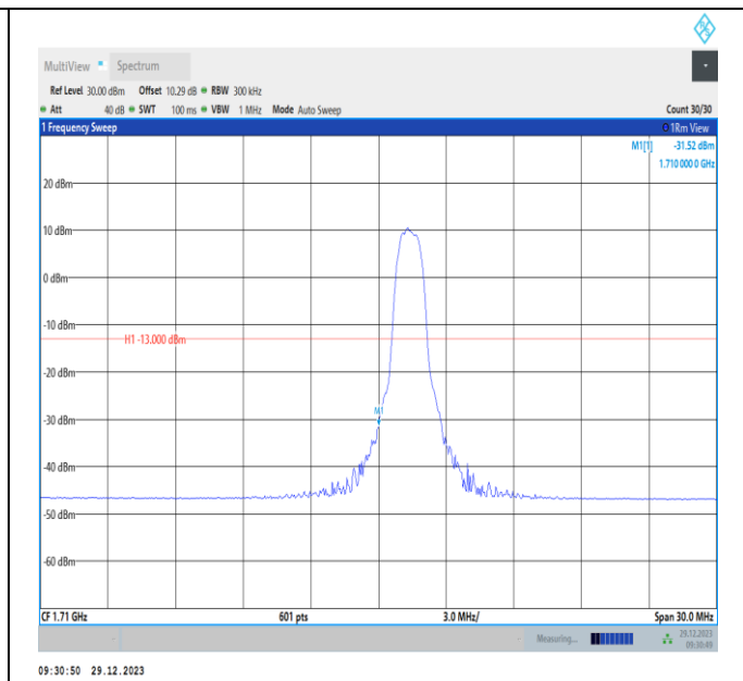
Band4-15MHz-16QAM-20025-PASS
