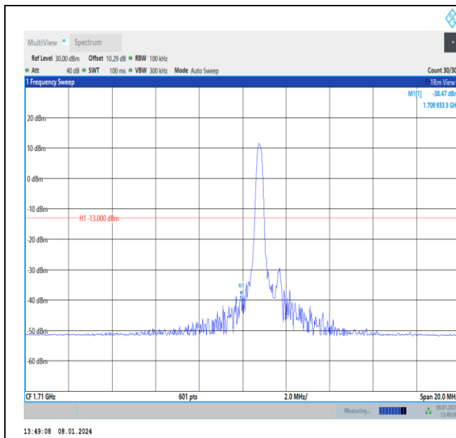
Band4-10MHz-QPSK-20000-PASS
