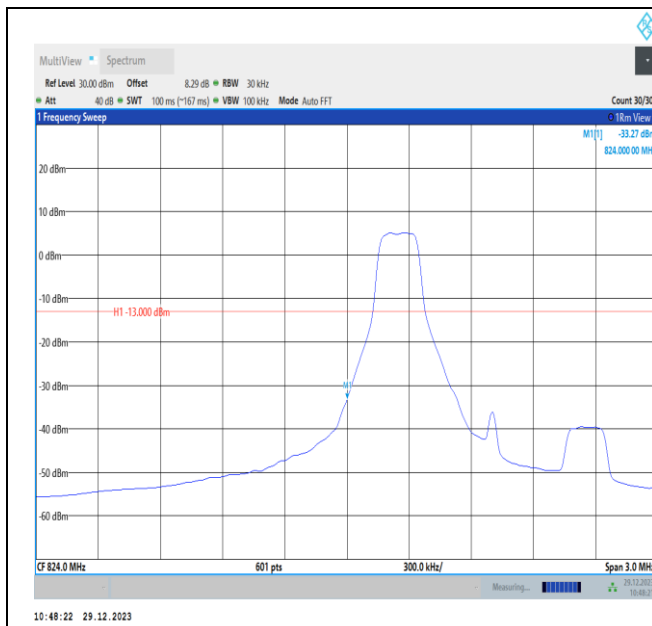
Band5-1.4MHz-16QAM-20407-PASS
