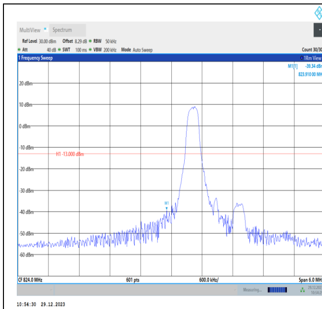
Band5-3MHz-16QAM-20415-PASS
