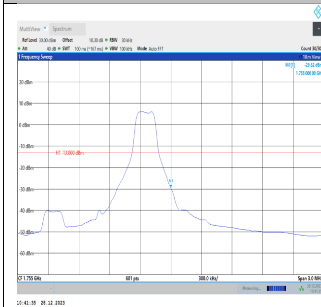
Band4-1.4MHz-QPSK-20393-PASS
