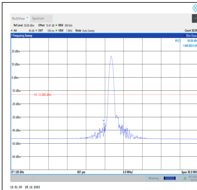
Band2-15MHz-16QAM-18675-PASS
