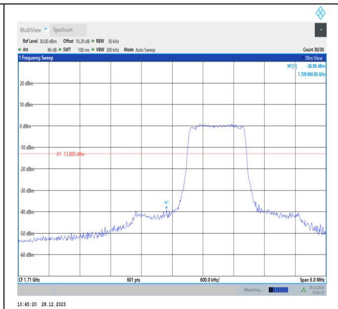
Band4-3MHz-QPSK-19965-PASS
