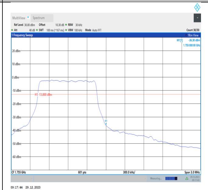
Band4-1.4MHz-16QAM-20393-PASS
