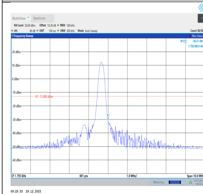
Band4-5MHz-16QAM-20375-PASS
