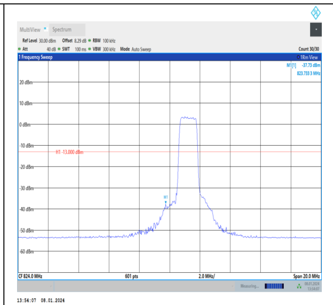
Band5-10MHz-QPSK-20450-PASS
