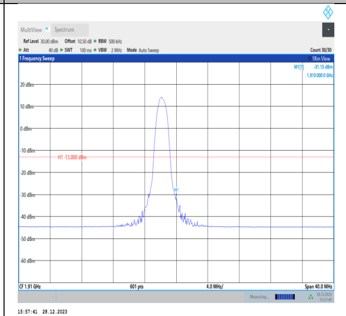
Band2-20MHz-16QAM-19100-PASS
