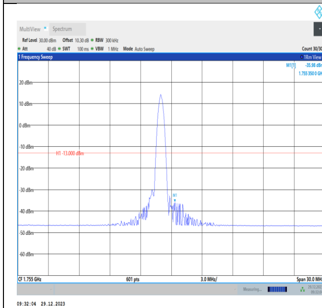
Band4-15MHz-16QAM-20325-PASS
