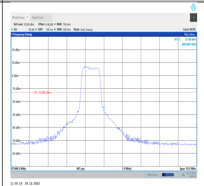
Band5-5MHz-16QAM-20625-PASS
