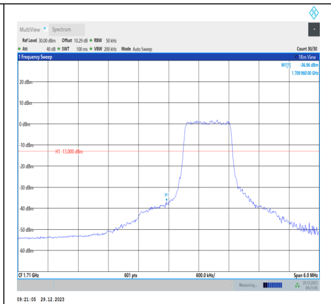
Band4-3MHz-16QAM-19965-PASS
