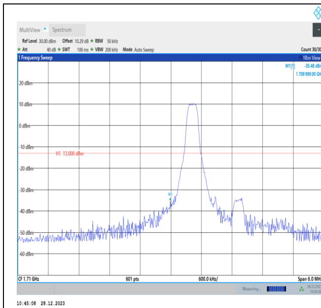
Band4-3MHz-QPSK-19965-PASS
