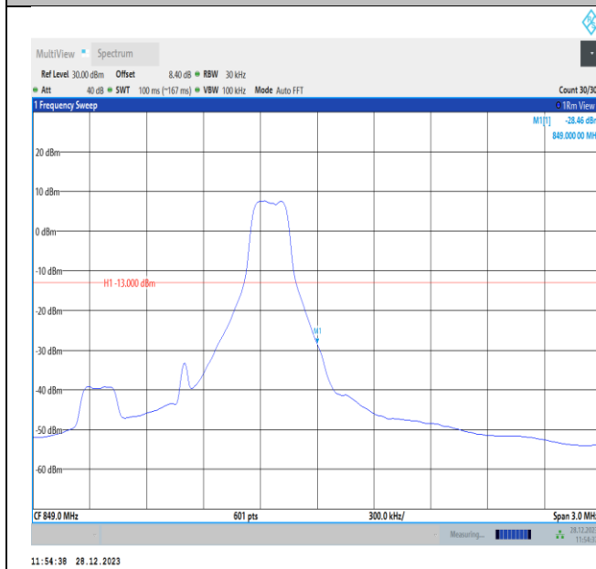
Band5-1.4MHz-QPSK-20643-PASS
