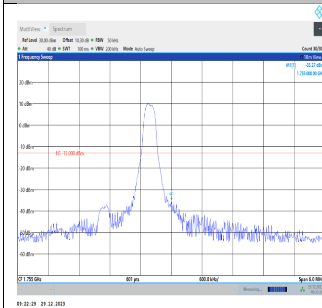
Band4-3MHz-16QAM-20385-PASS
