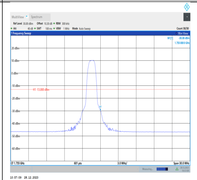
Band4-15MHz-QPSK-20325-PASS
