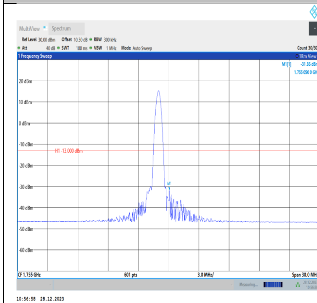
Band4-15MHz-QPSK-20325-PASS
