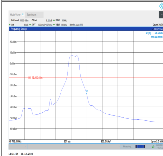
Band12-1.4MHz-QPSK-23173-PASS
