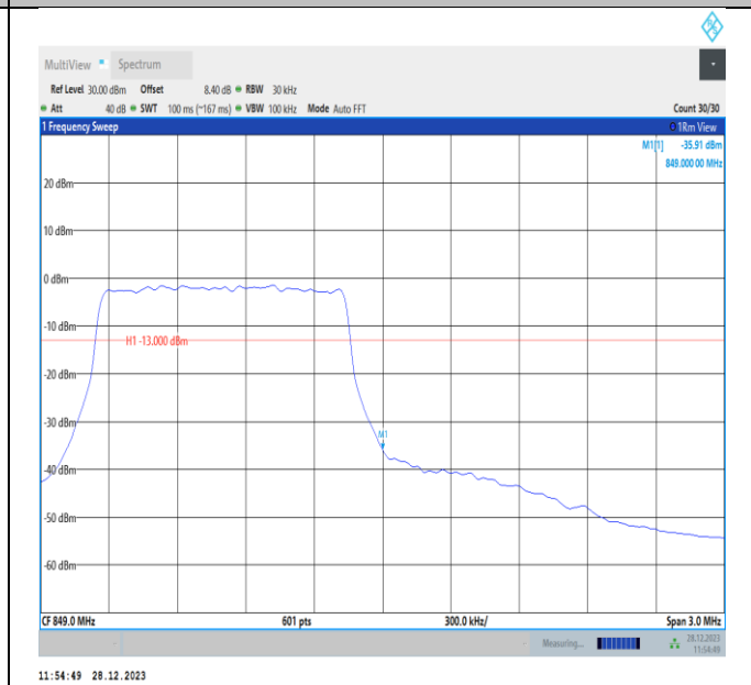
Band5-1.4MHz-QPSK-20643-PASS
