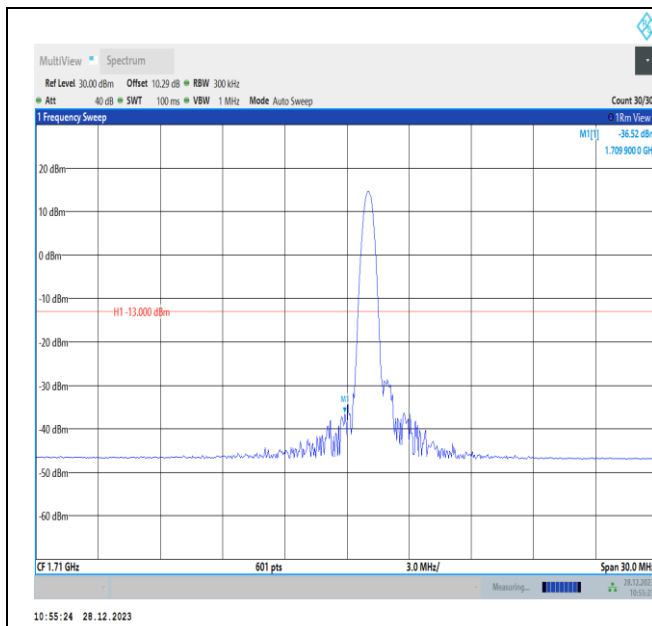
Band4-15MHz-QPSK-20025-PASS
