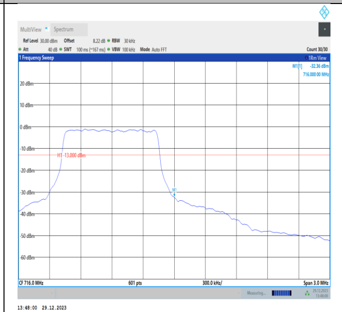
Band12-1.4MHz-16QAM-23173-PASS
