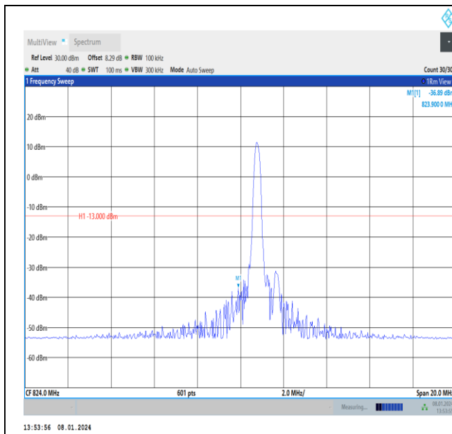
Band5-10MHz-QPSK-20450-PASS
