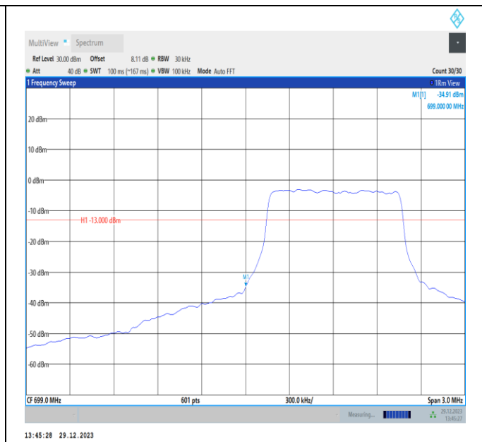
Band12-1.4MHz-16QAM-23017-PASS
