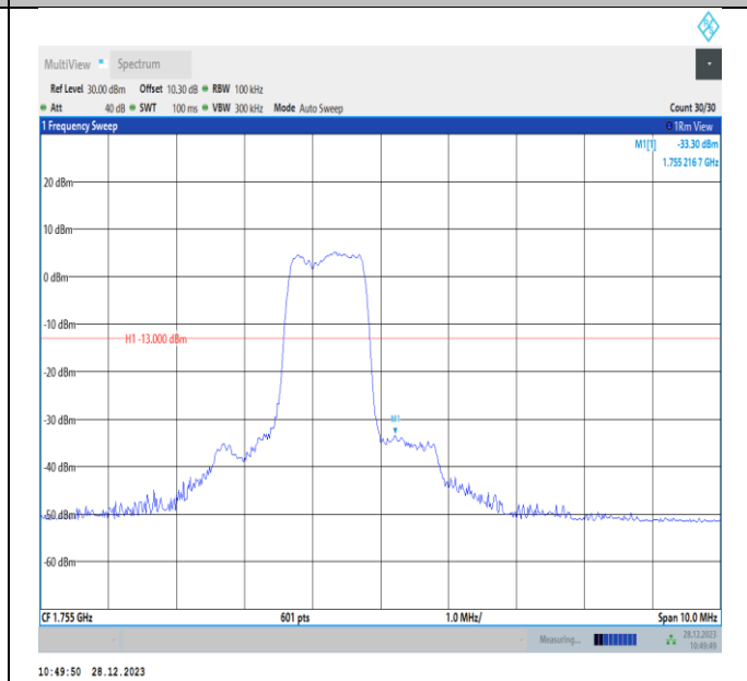
Band4-5MHz-QPSK-20375-PASS
