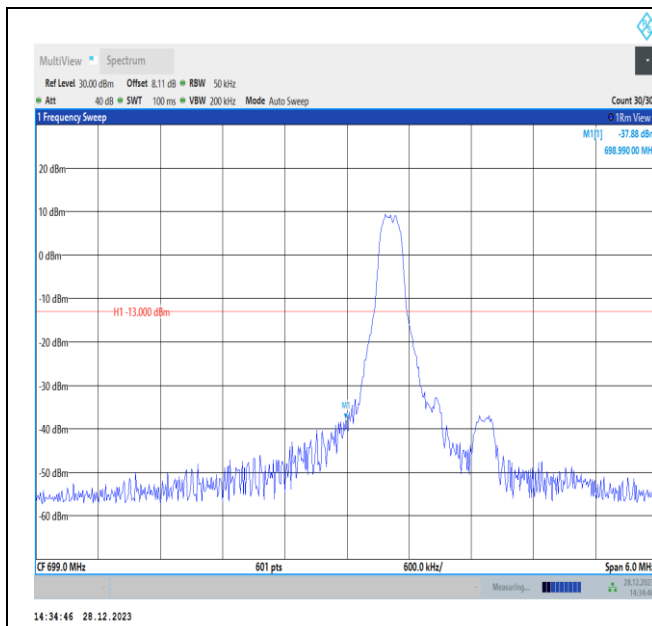
Band12-3MHz-QPSK-23025-PASS
