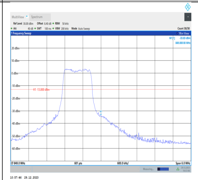
Band5-3MHz-16QAM-20635-PASS
