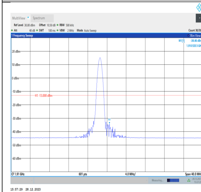
Band2-20MHz-16QAM-19100-PASS
