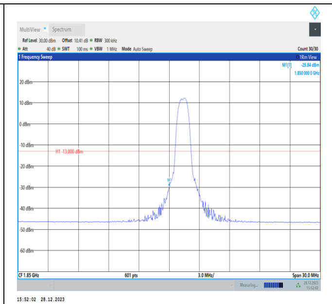
Band2-15MHz-16QAM-18675-PASS
