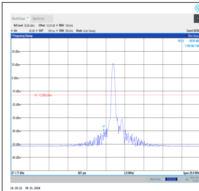
Band4-10MHz-16QAM-20000-PASS
