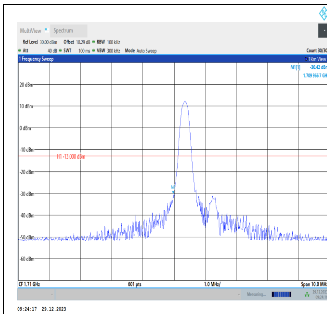
Band4-5MHz-16QAM-19975-PASS
