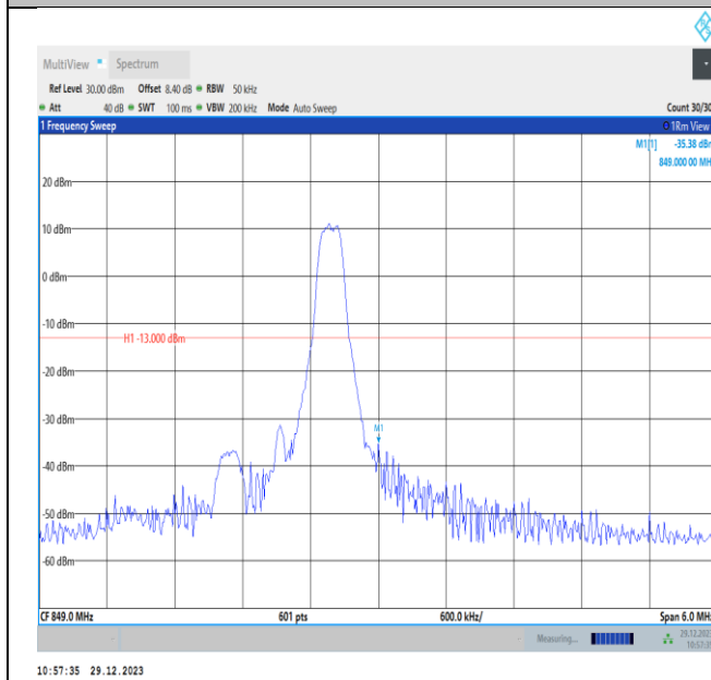
Band5-3MHz-16QAM-20635-PASS
