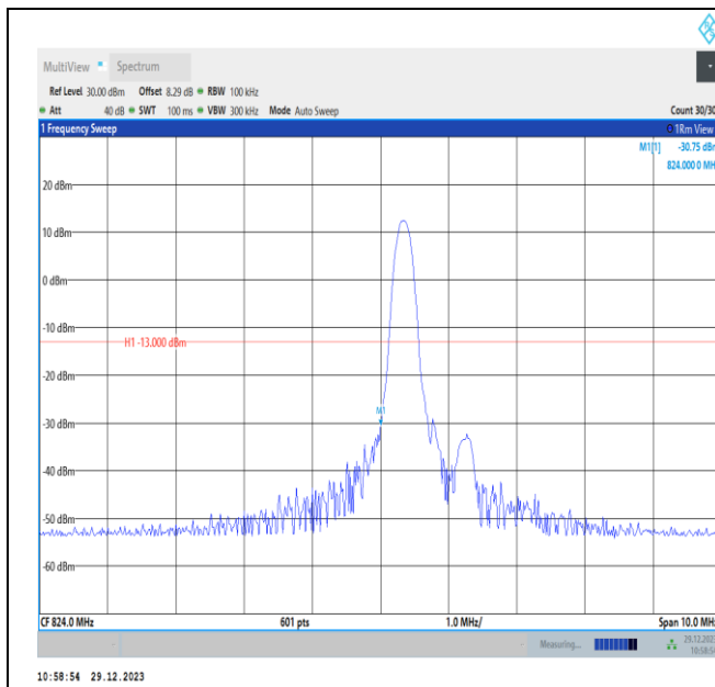
Band5-5MHz-16QAM-20425-PASS
