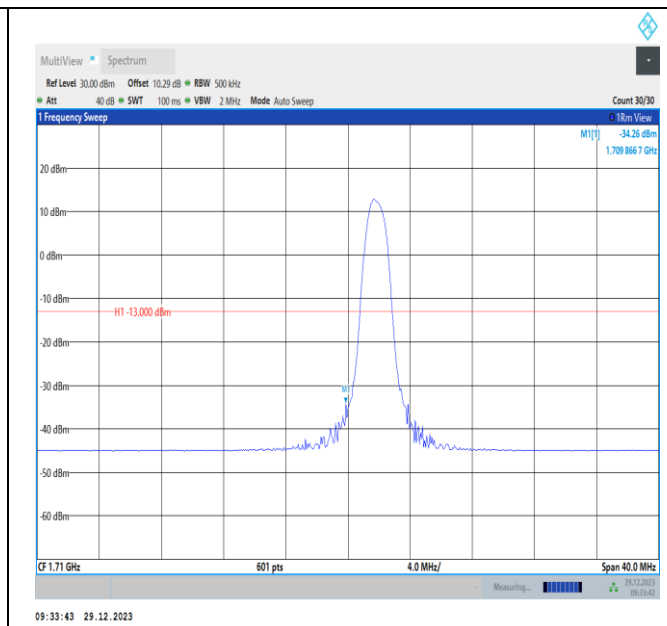
Band4-20MHz-16QAM-20050-PASS
