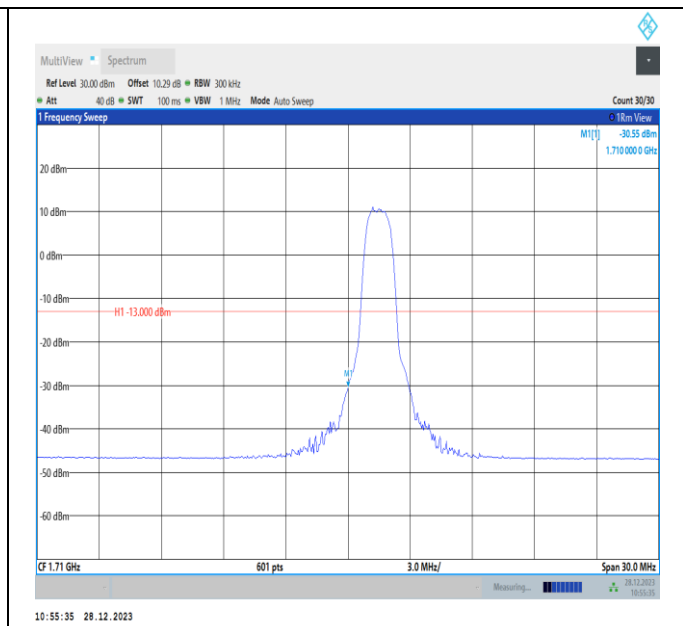
Band4-15MHz-QPSK-20025-PASS
