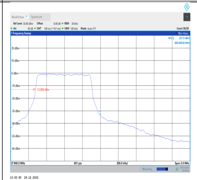
Band5-1.4MHz-16QAM-20643-PASS
