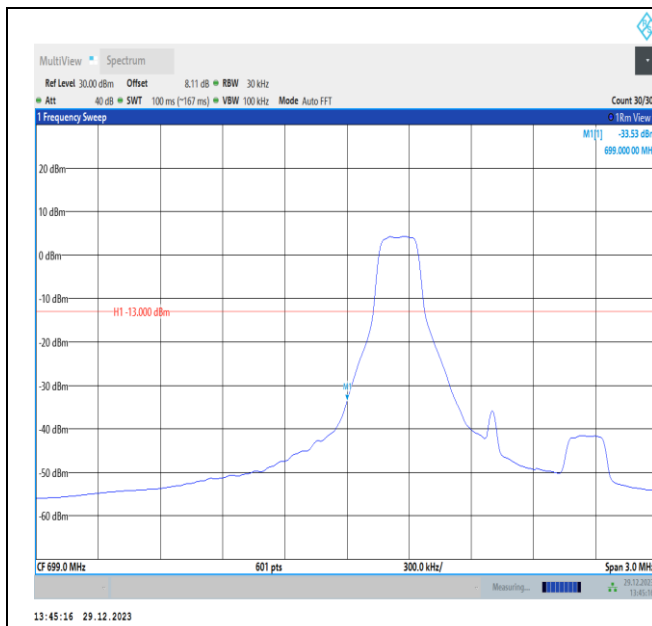
Band12-1.4MHz-16QAM-23017-PASS
