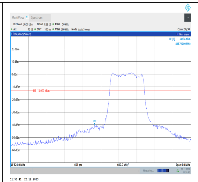
Band5-3MHz-QPSK-20415-PASS
