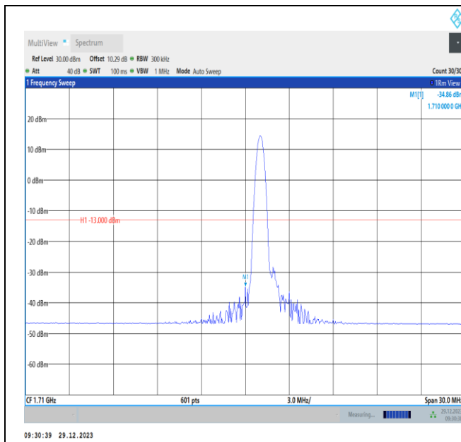
Band4-15MHz-16QAM-20025-PASS
