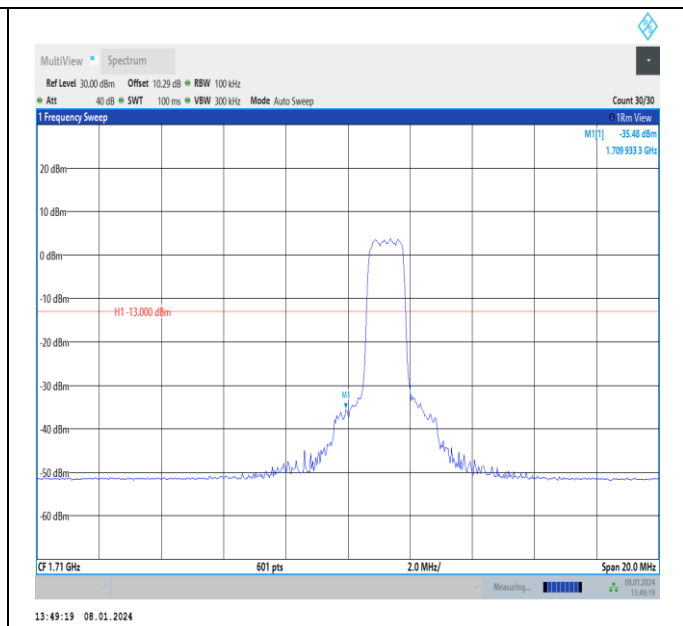
Band4-10MHz-QPSK-20000-PASS
