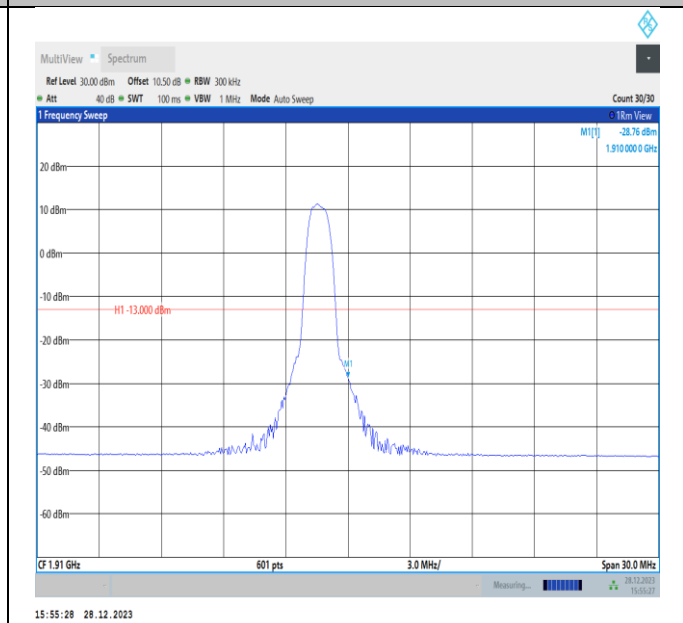
Band2-15MHz-16QAM-19125-PASS
