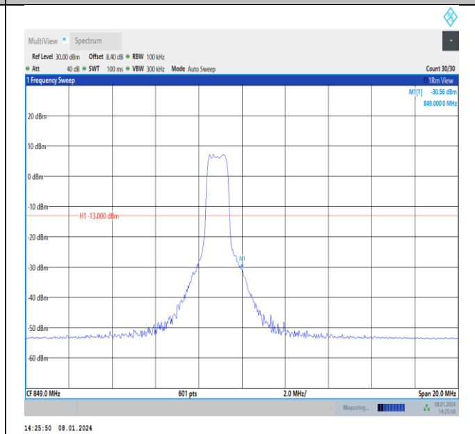
Band5-10MHz-16QAM-20600-PASS
