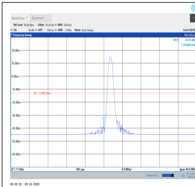
Band4-20MHz-16QAM-20050-PASS
