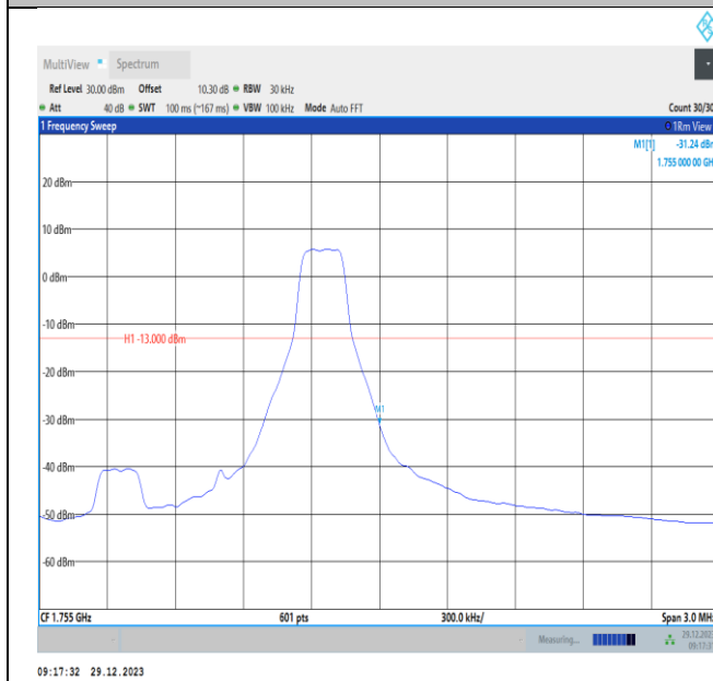
Band4-1.4MHz-16QAM-20393-PASS
