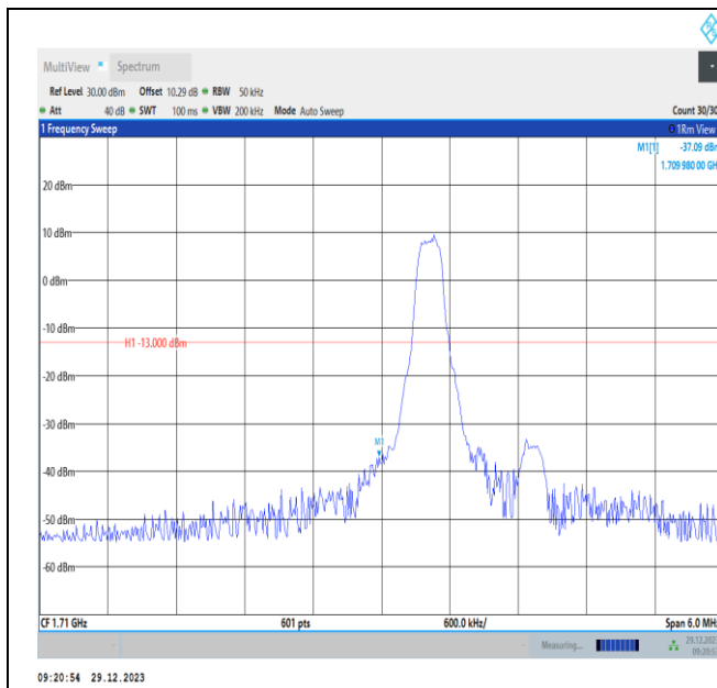
Band4-3MHz-16QAM-19965-PASS
