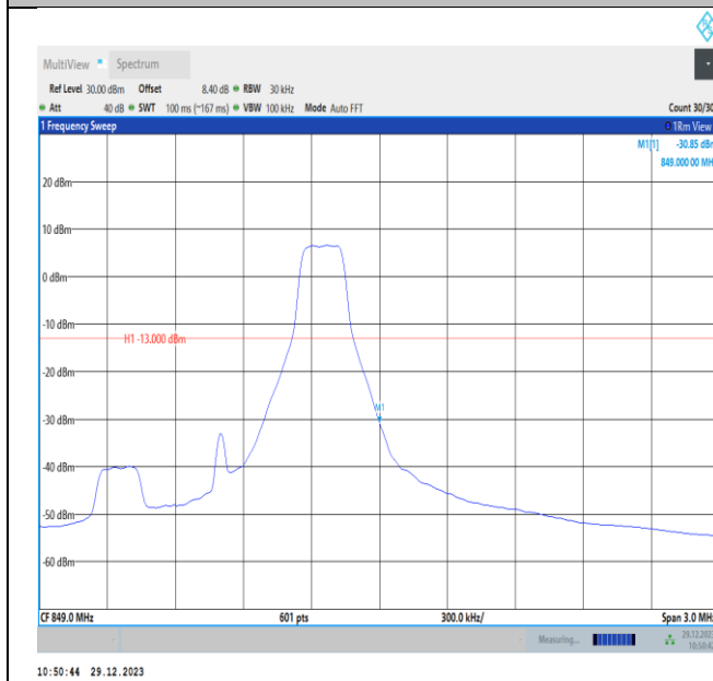
Band5-1.4MHz-16QAM-20643-PASS
