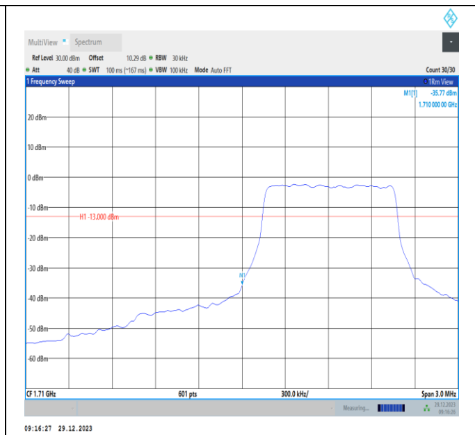
Band4-1.4MHz-16QAM-19957-PASS
