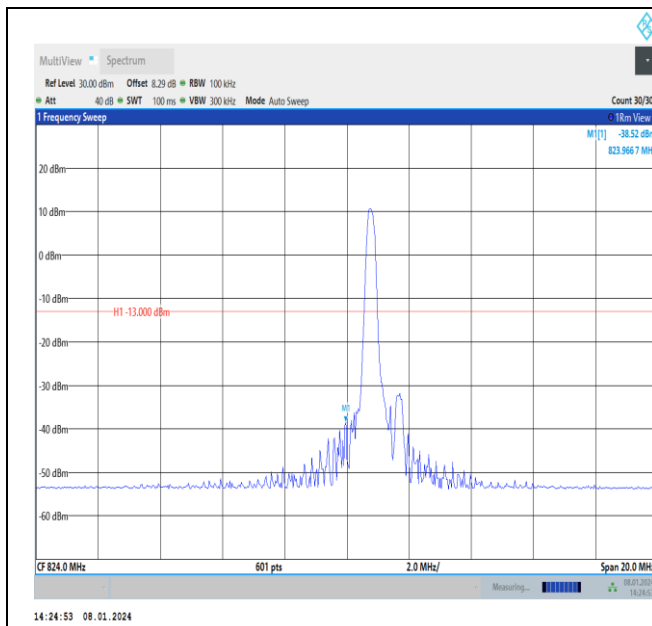
Band5-10MHz-16QAM-20450-PASS
