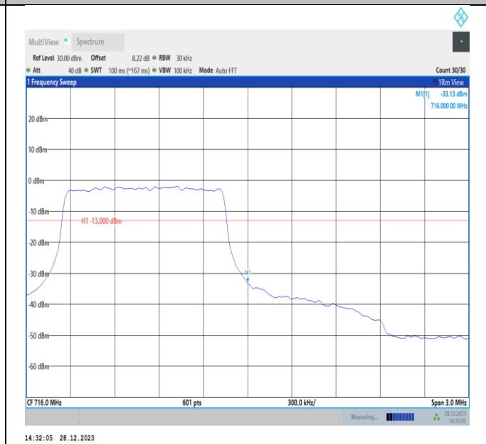
Band12-1.4MHz-QPSK-23173-PASS
