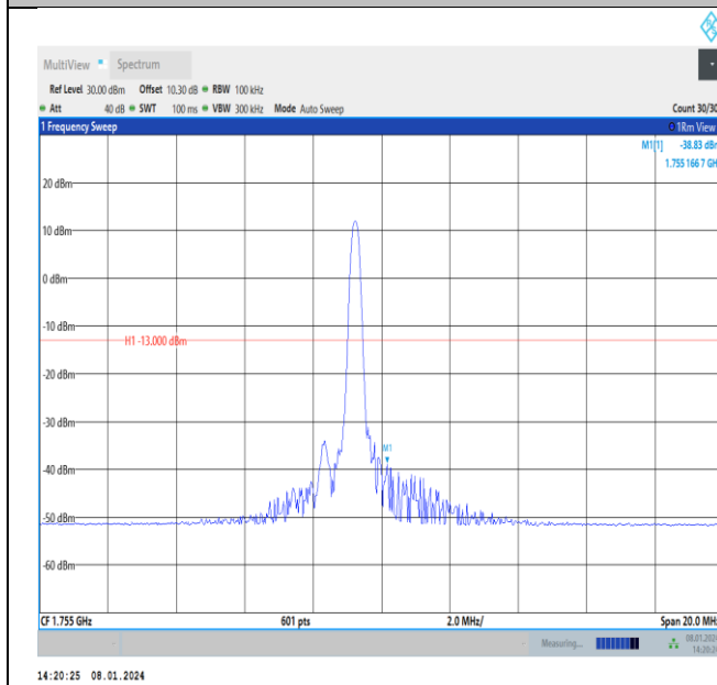
Band4-10MHz-16QAM-20350-PASS
