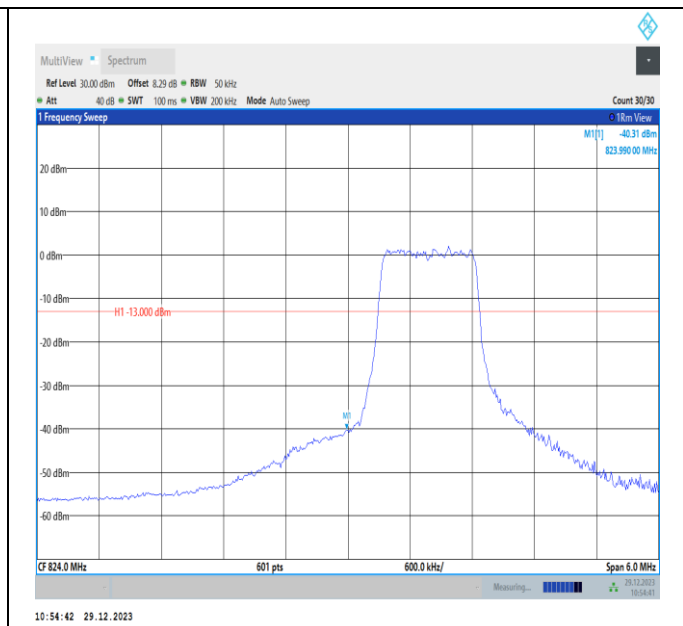
Band5-3MHz-16QAM-20415-PASS
