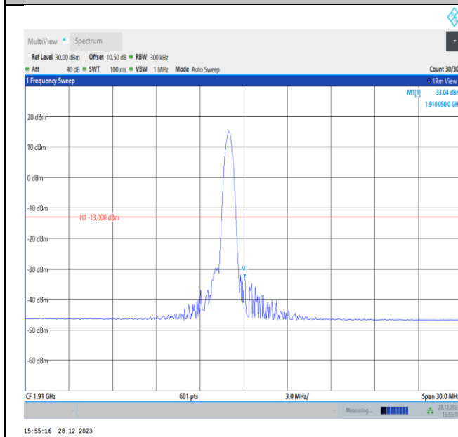
Band2-15MHz-16QAM-19125-PASS
