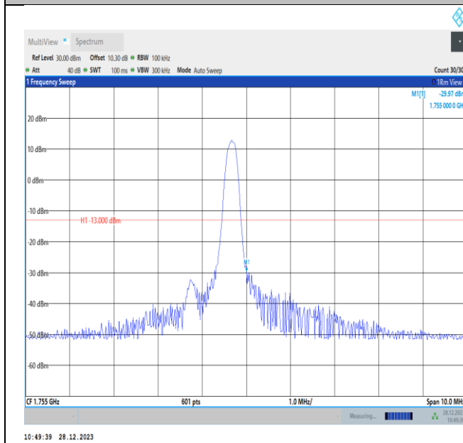
Band4-5MHz-QPSK-20375-PASS
