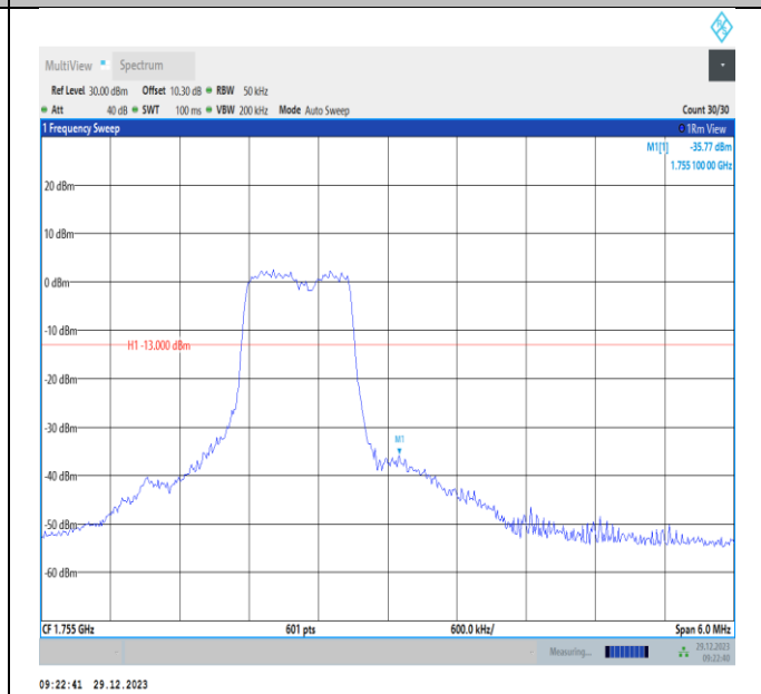
Band4-3MHz-16QAM-20385-PASS
