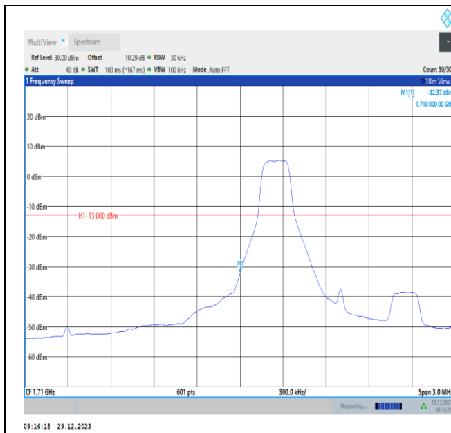
Band4-1.4MHz-16QAM-19957-PASS
