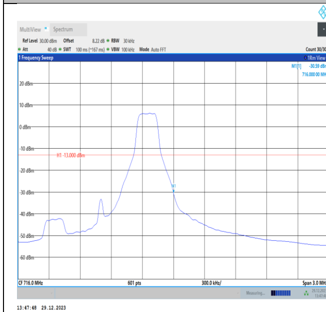
Band12-1.4MHz-16QAM-23173-PASS
