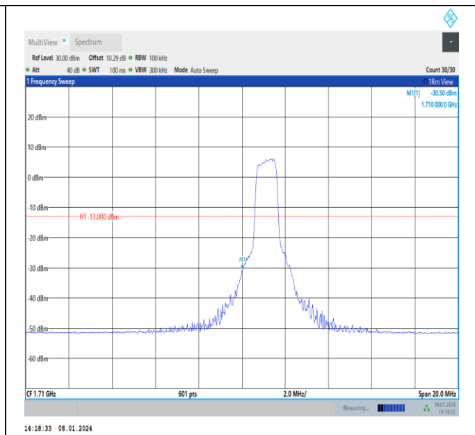
Band4-10MHz-16QAM-20000-PASS
