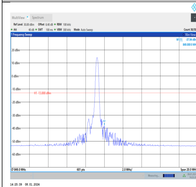
Band5-10MHz-16QAM-20600-PASS
