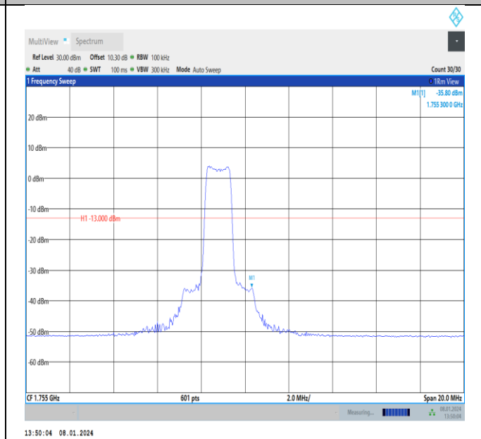
Band4-10MHz-QPSK-20350-PASS
