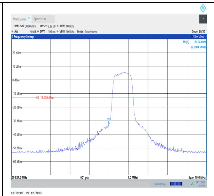
Band5-5MHz-16QAM-20425-PASS
