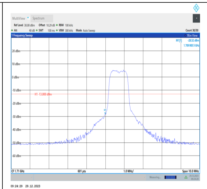
Band4-5MHz-16QAM-19975-PASS
