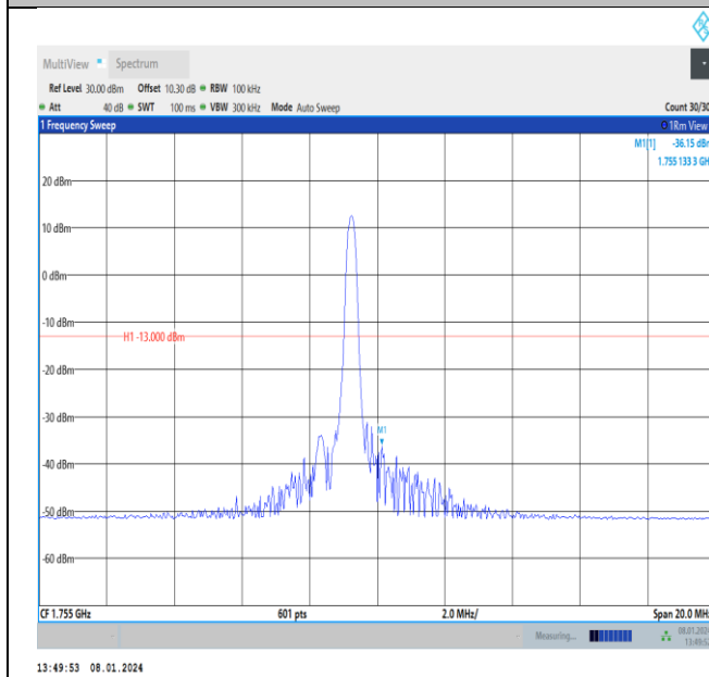
Band4-10MHz-QPSK-20350-PASS
