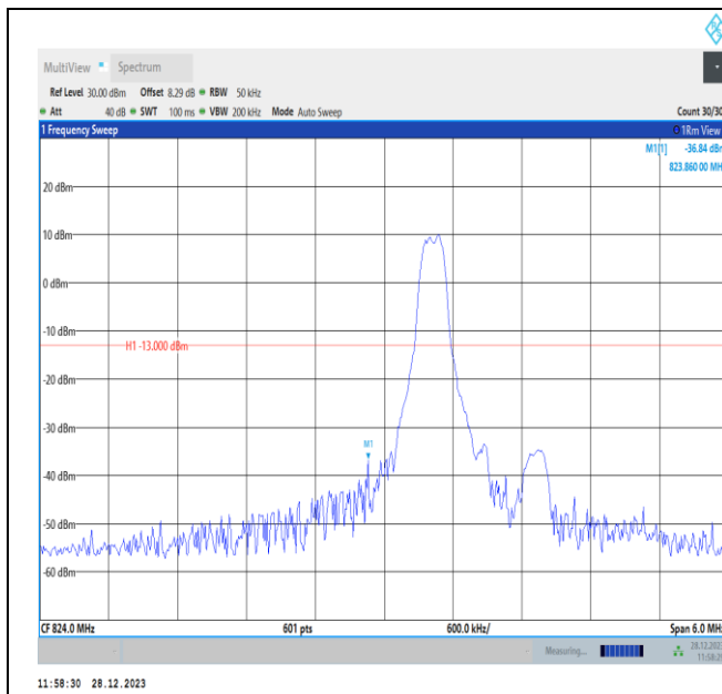
Band5-3MHz-QPSK-20415-PASS
