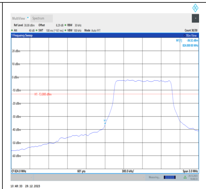
Band5-1.4MHz-16QAM-20407-PASS
