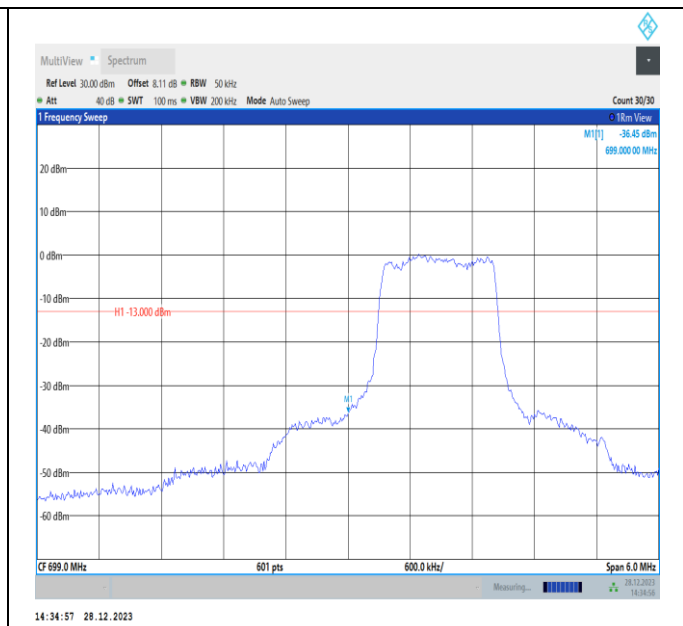
Band12-3MHz-QPSK-23025-PASS
