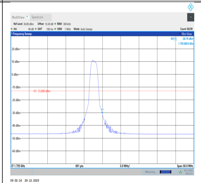
Band4-15MHz-16QAM-20325-PASS
