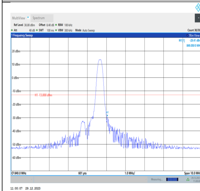
Band5-5MHz-16QAM-20625-PASS
