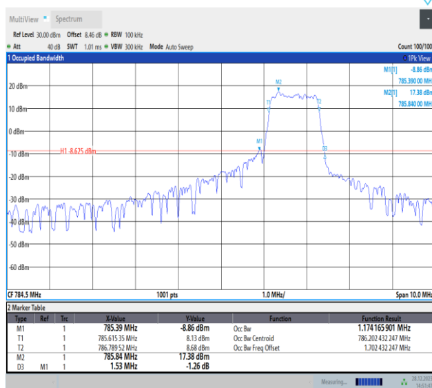
Band13-5MHz-QPSK-23255-PASS
