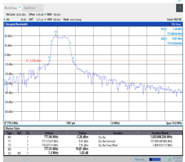
Band13-5MHz-16QAM-23205-PASS
