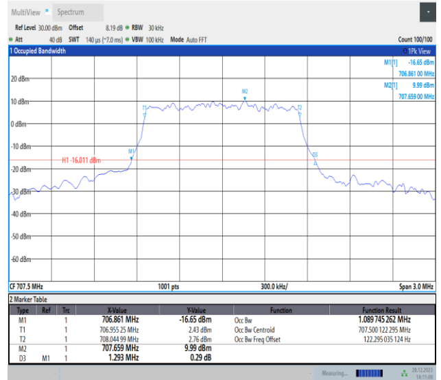
Band12-1.4MHz-QPSK-23095-PASS
