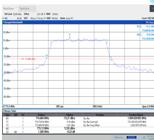
Band12-1.4MHz-QPSK-23173-PASS
