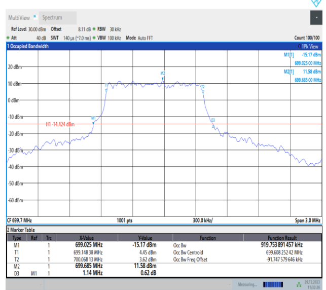
Band12-1.4MHz-16QAM-23017-PASS
