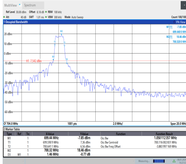
Band12-10MHz-16QAM-23060-PASS
