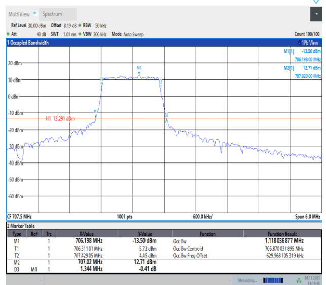
Band12-3MHz-QPSK-23095-PASS
