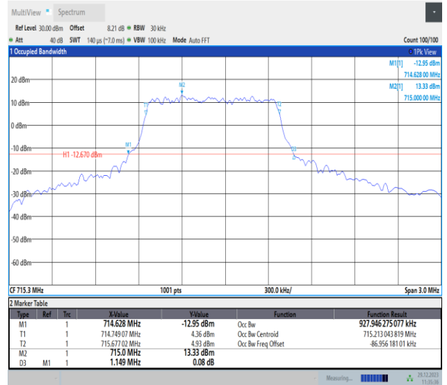
Band12-1.4MHz-16QAM-23173-PASS
