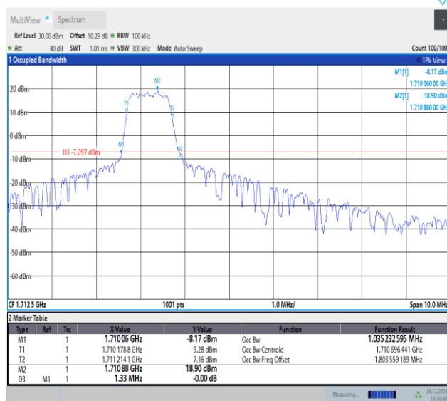
Band4-5MHz-16QAM-19975-PASS
