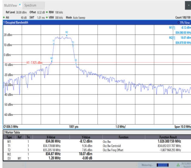
Band5-5MHz-16QAM-20525-PASS
