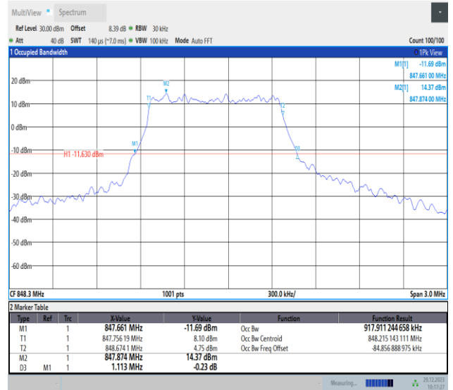
Band5-1.4MHz-16QAM-20643-PASS
