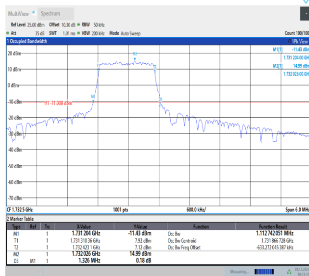
Band4-3MHz-QPSK-20175-PASS
