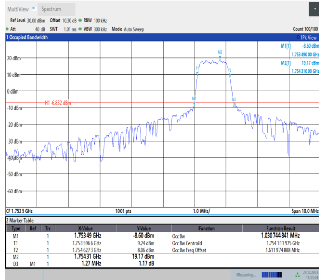
Band4-5MHz-16QAM-20375-PASS
