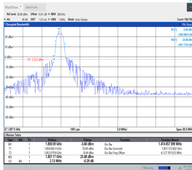
Band2-15MHz-16QAM-18675-PASS
