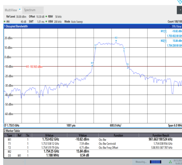
Band4-3MHz-16QAM-20385-PASS
