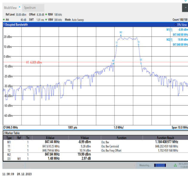
Band5-5MHz-QPSK-20625-PASS
