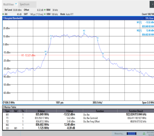
Band5-1.4MHz-16QAM-20525-PASS
