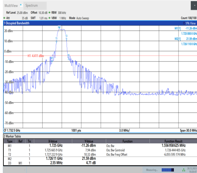
Band4-15MHz-QPSK-20175-PASS
