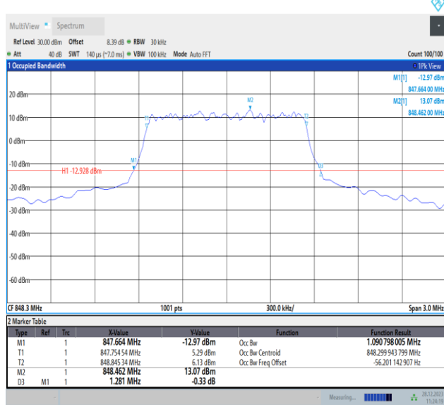
Band5-1.4MHz-QPSK-20643-PASS
