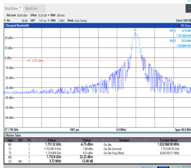
Band4-20MHz-16QAM-20300-PASS
