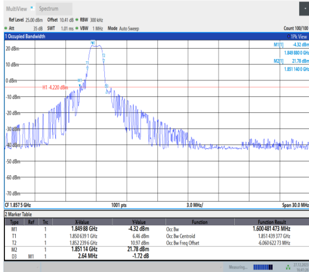
Band2-15MHz-QPSK-18675-PASS
