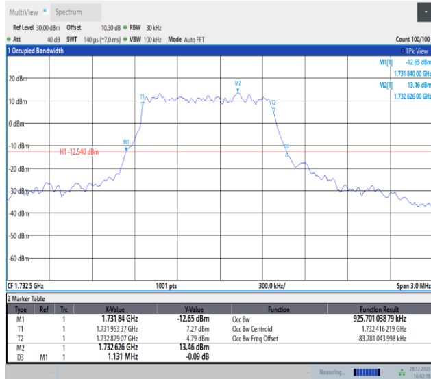
Band4-1.4MHz-16QAM-20175-PASS
