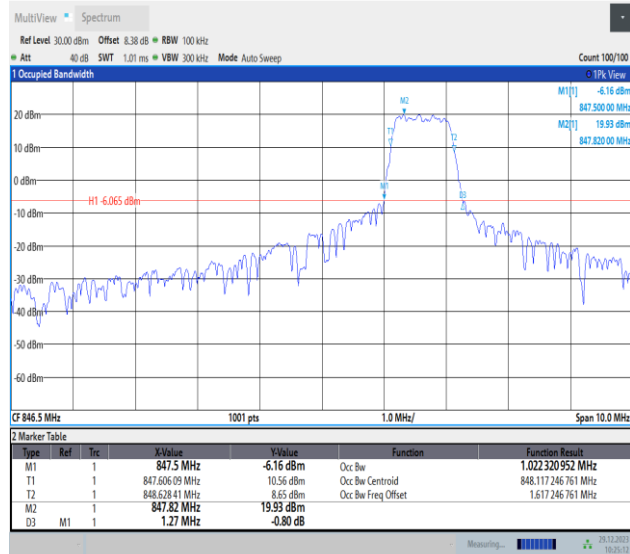
Band5-5MHz-16QAM-20625-PASS
