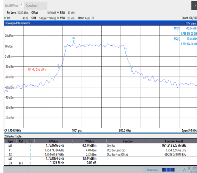
Band4-1.4MHz-16QAM-20393-PASS
