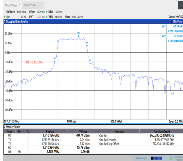
Band4-3MHz-16QAM-19965-PASS
