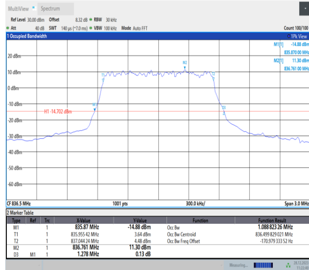
Band5-1.4MHz-QPSK-20525-PASS
