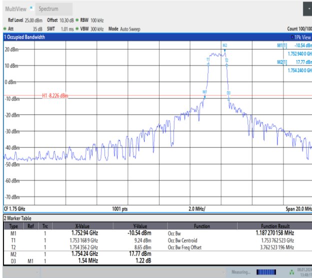
Band4-10MHz-QPSK-20350-PASS
