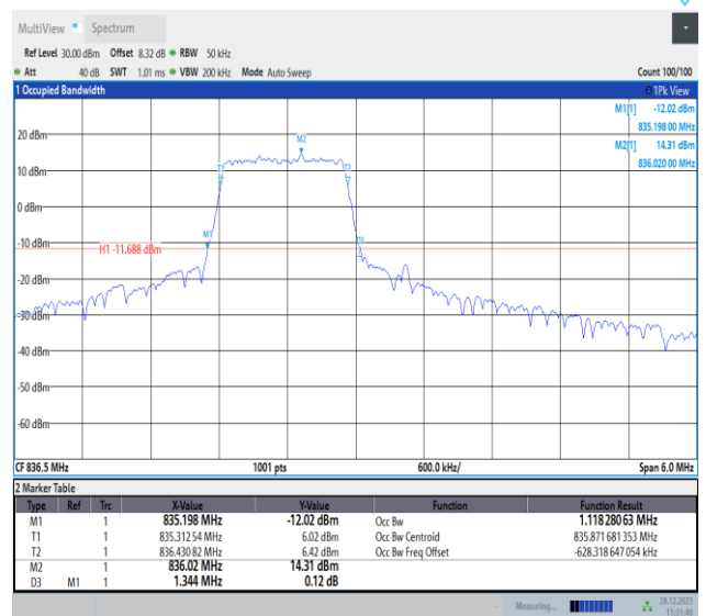
Band5-3MHz-QPSK-20525-PASS
