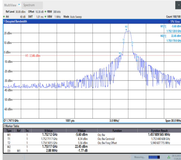
Band4-15MHz-16QAM-20325-PASS
