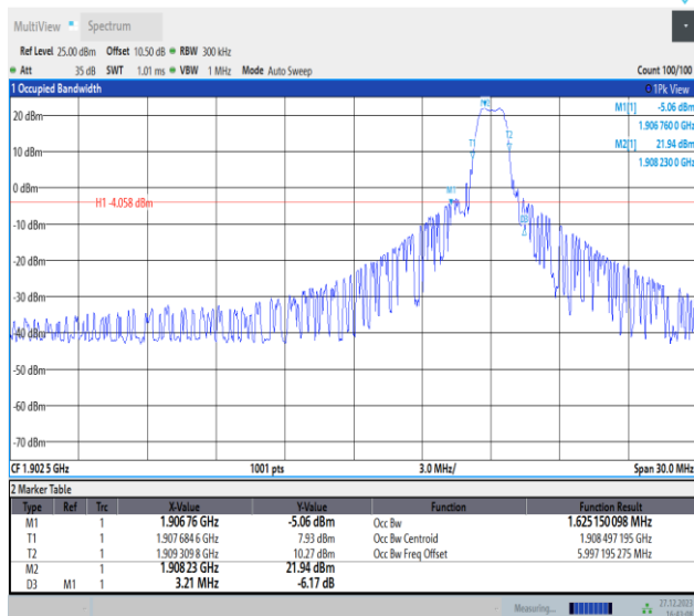
Band2-15MHz-QPSK-19125-PASS
