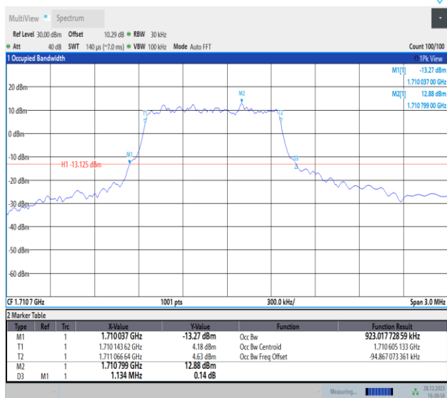
Band4-1.4MHz-16QAM-19957-PASS
