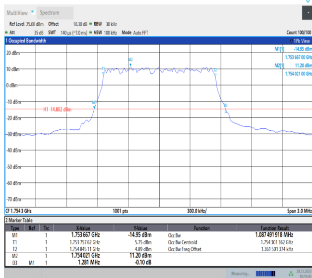
Band4-1.4MHz-QPSK-20393-PASS
