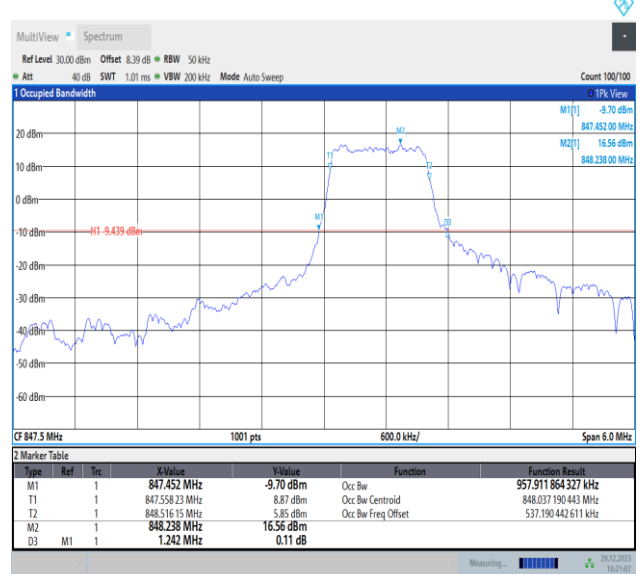
Band5-3MHz-16QAM-20635-PASS
