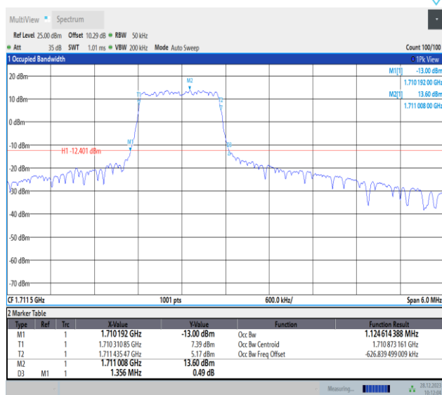
Band4-3MHz-QPSK-19965-PASS
