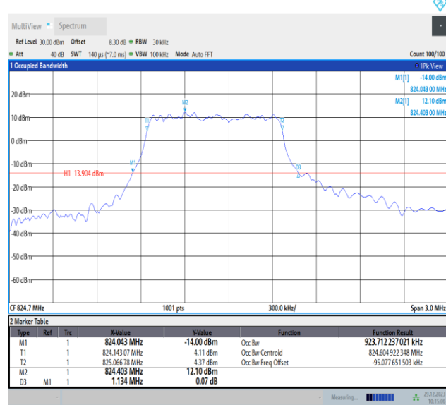
Band5-1.4MHz-16QAM-20407-PASS
