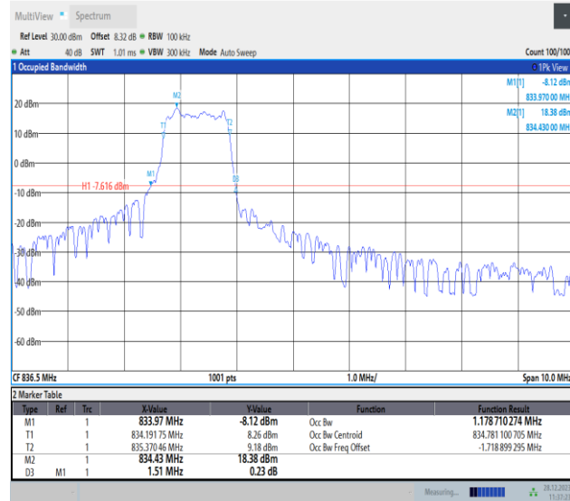
Band5-5MHz-QPSK-20525-PASS
