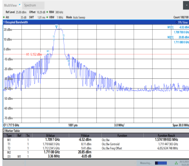
Band4-15MHz-QPSK-20025-PASS
