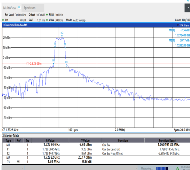
Band4-10MHz-16QAM-20175-PASS
