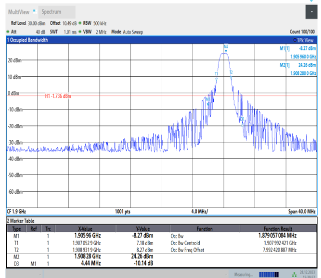
Band2-20MHz-16QAM-19100-PASS
