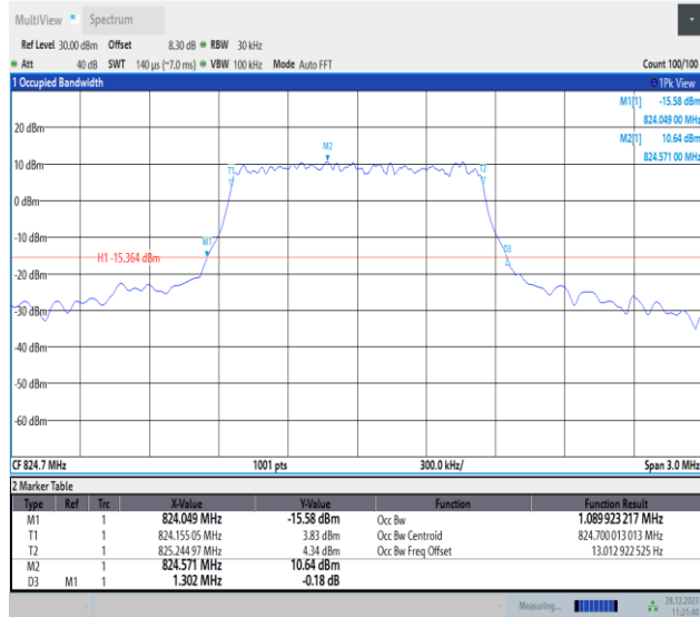
Band5-1.4MHz-QPSK-20407-PASS
