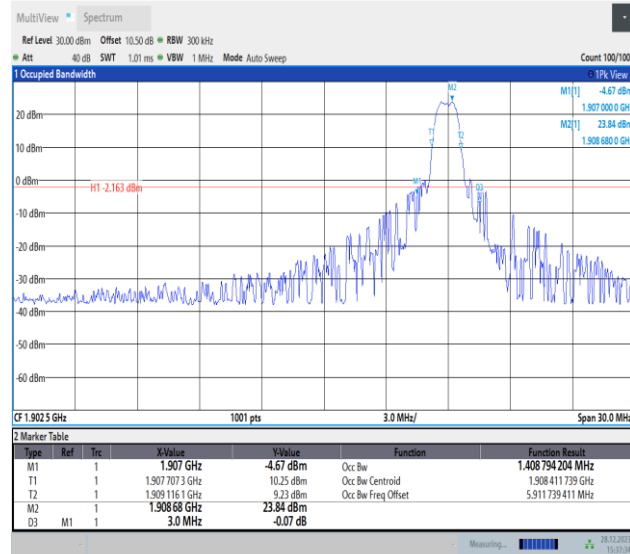
Band2-15MHz-16QAM-19125-PASS
