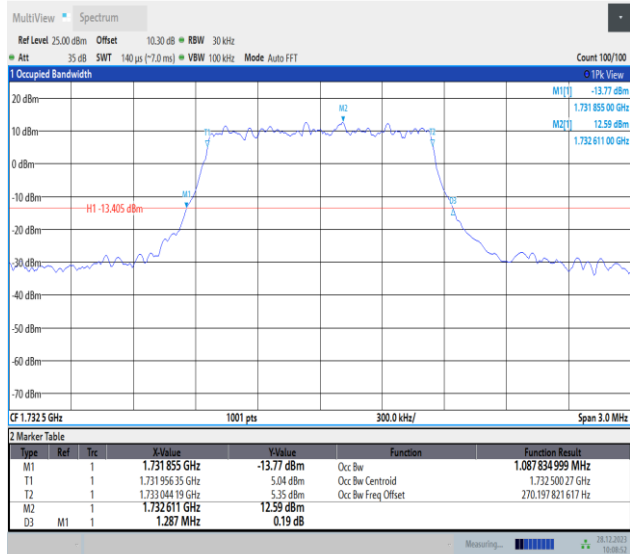
Band4-1.4MHz-QPSK-20175-PASS
