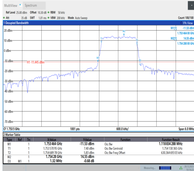
Band4-3MHz-QPSK-20385-PASS
