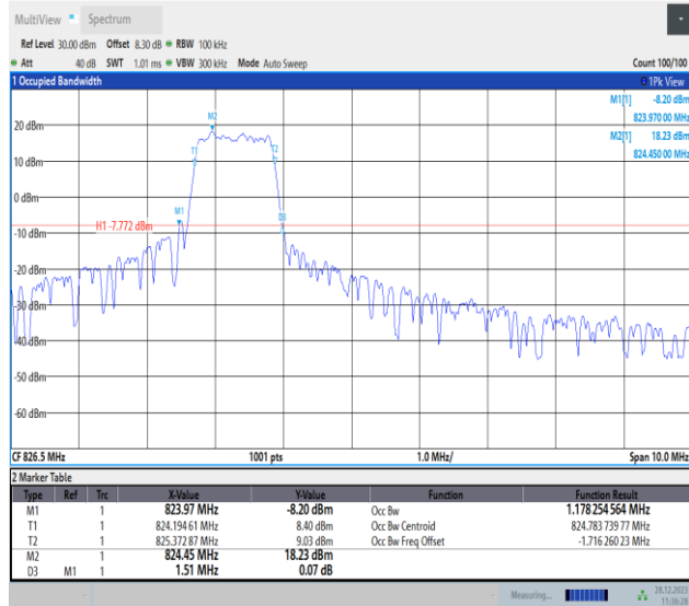
Band5-5MHz-QPSK-20425-PASS
