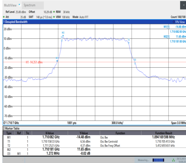
Band4-1.4MHz-QPSK-19957-PASS
