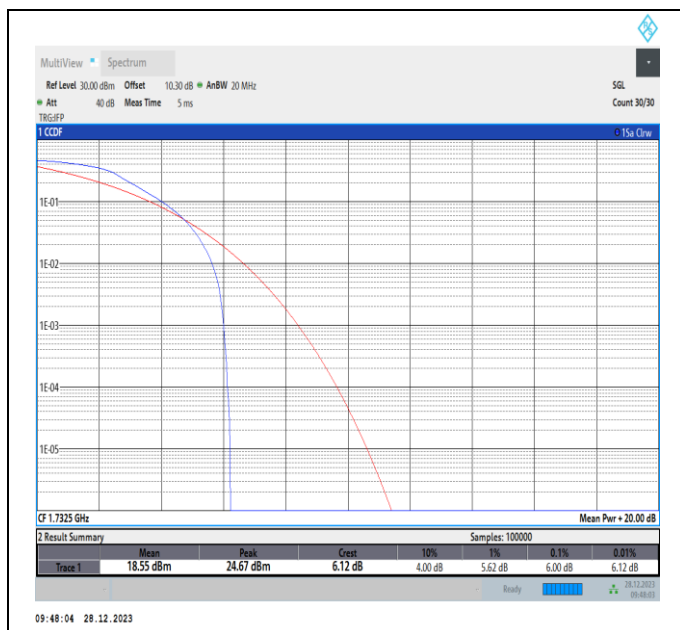
Band4-20MHz-QPSK-20175-PASS
