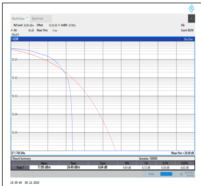
Band4-20MHz-16QAM-20300-PASS
