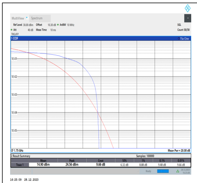
Band4-10MHz-16QAM-20350-PASS
