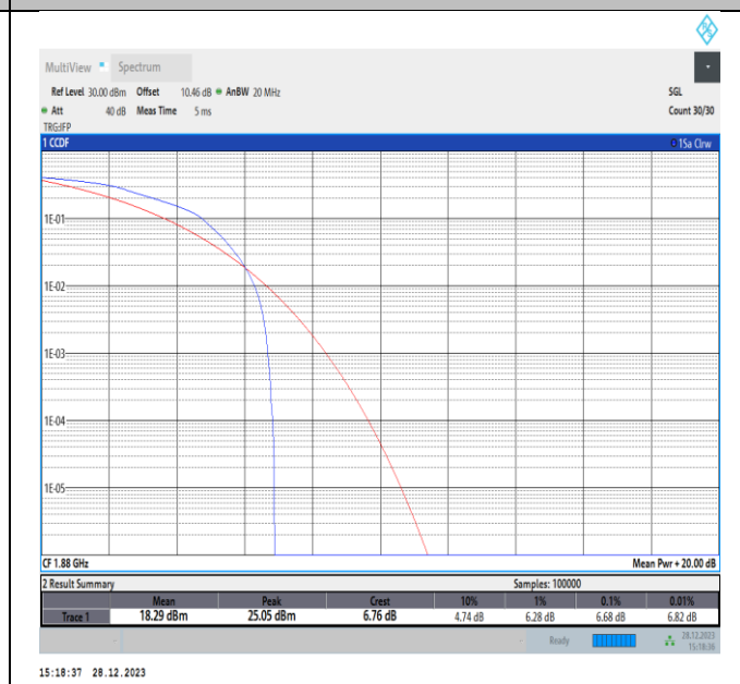
Band2-20MHz-16QAM-18900-PASS
