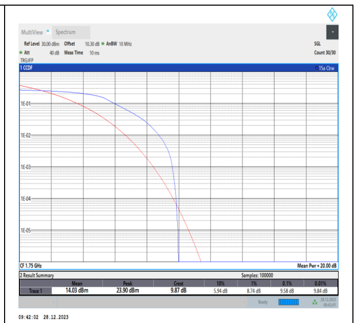
Band4-10MHz-QPSK-20350-PASS
