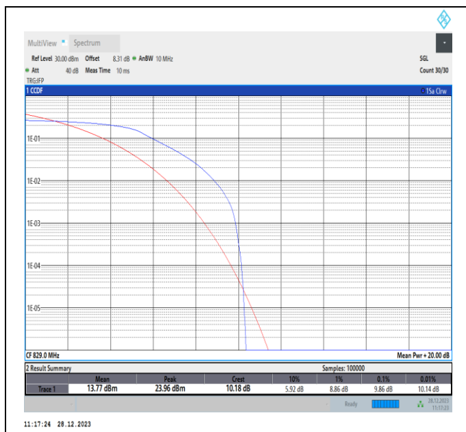
Band5-10MHz-QPSK-20450-PASS
