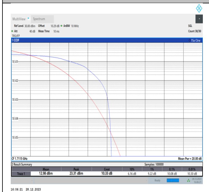
Band4-3MHz-16QAM-19965-PASS
