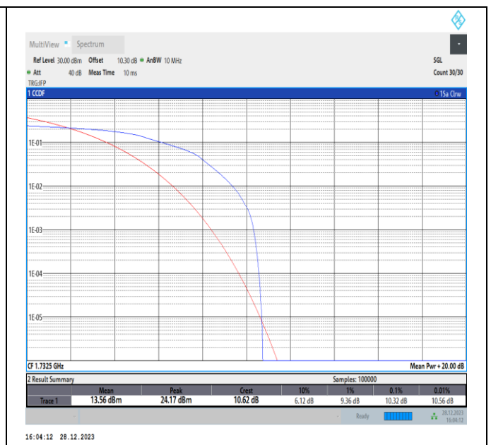
Band4-1.4MHz-16QAM-20175-PASS
