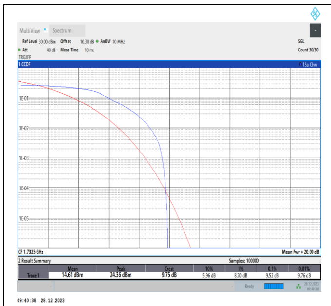
Band4-10MHz-QPSK-20175-PASS
