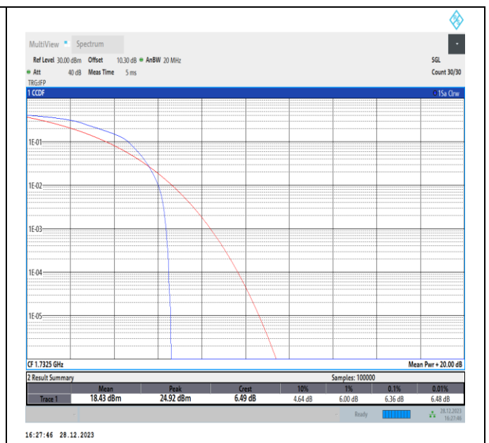
Band4-15MHz-16QAM-20175-PASS
