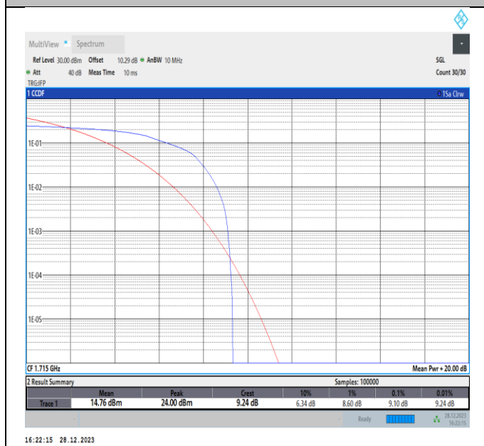
Band4-10MHz-16QAM-20000-PASS
