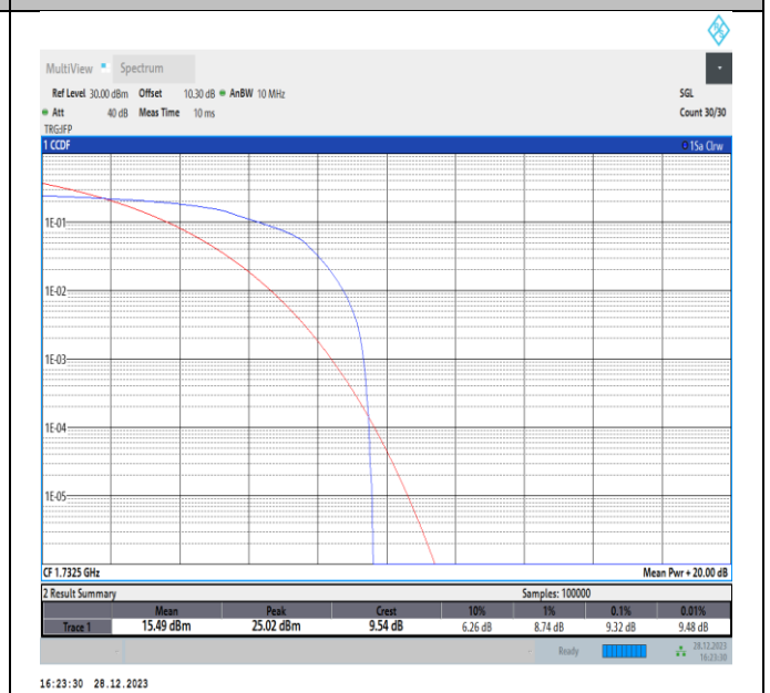
Band4-10MHz-16QAM-20175-PASS
