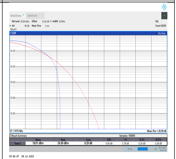
Band4-15MHz-QPSK-20325-PASS
