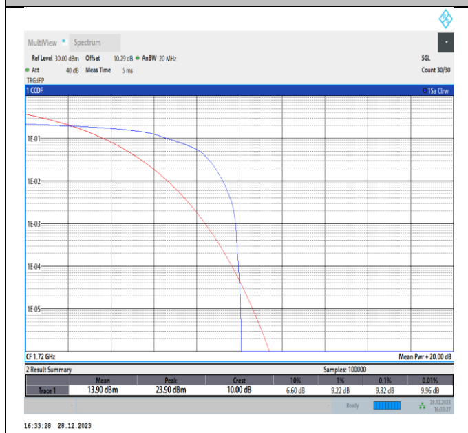
Band4-20MHz-16QAM-20050-PASS
