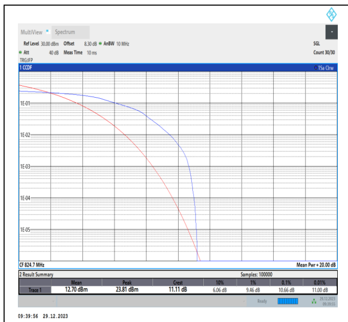
Band5-1.4MHz-16QAM-20407-PASS
