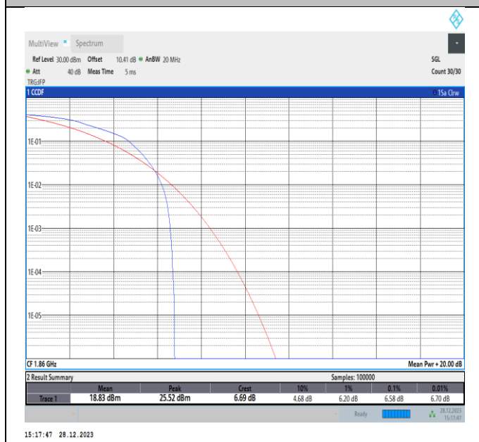
Band2-20MHz-16QAM-18700-PASS
