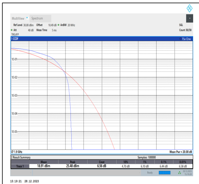
Band2-20MHz-16QAM-19100-PASS
