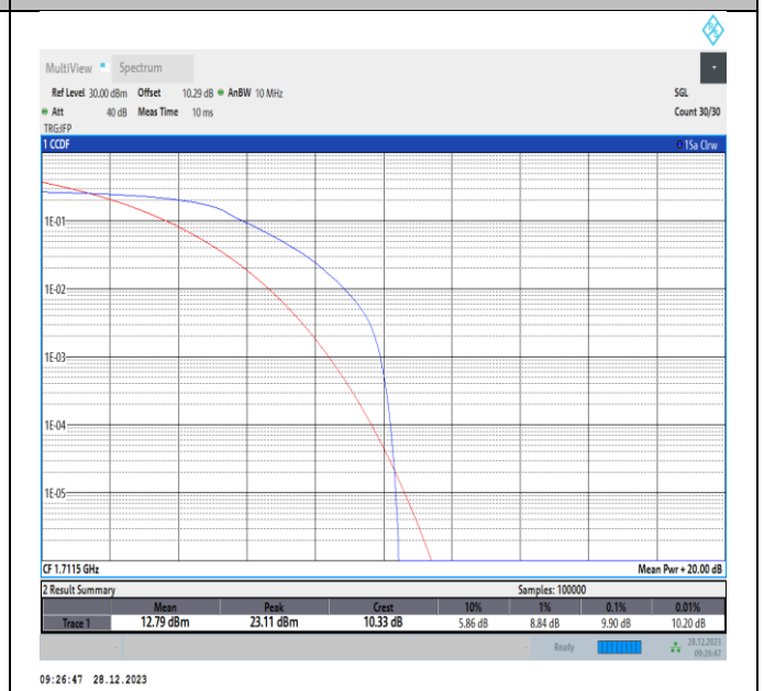
Band4-3MHz-QPSK-19965-PASS
