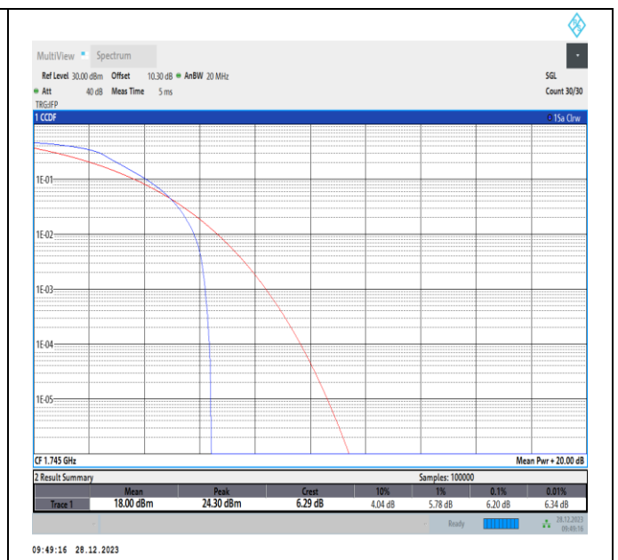
Band4-20MHz-QPSK-20300-PASS
