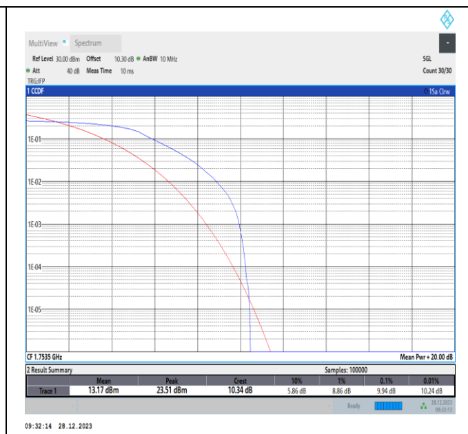
Band4-3MHz-QPSK-20385-PASS
