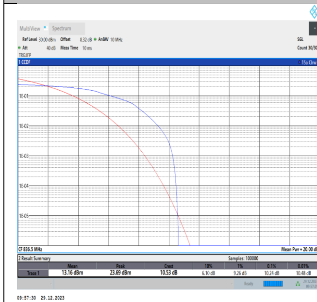
Band5-5MHz-16QAM-20525-PASS
