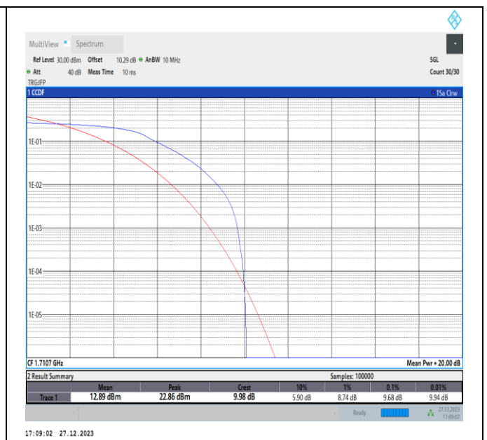
Band4-1.4MHz-QPSK-19957-PASS
