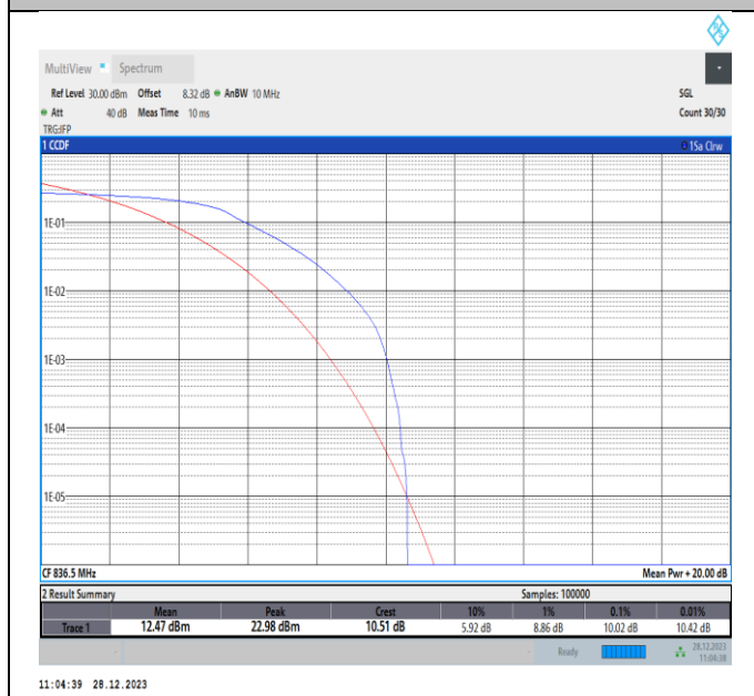
Band5-1.4MHz-QPSK-20525-PASS
