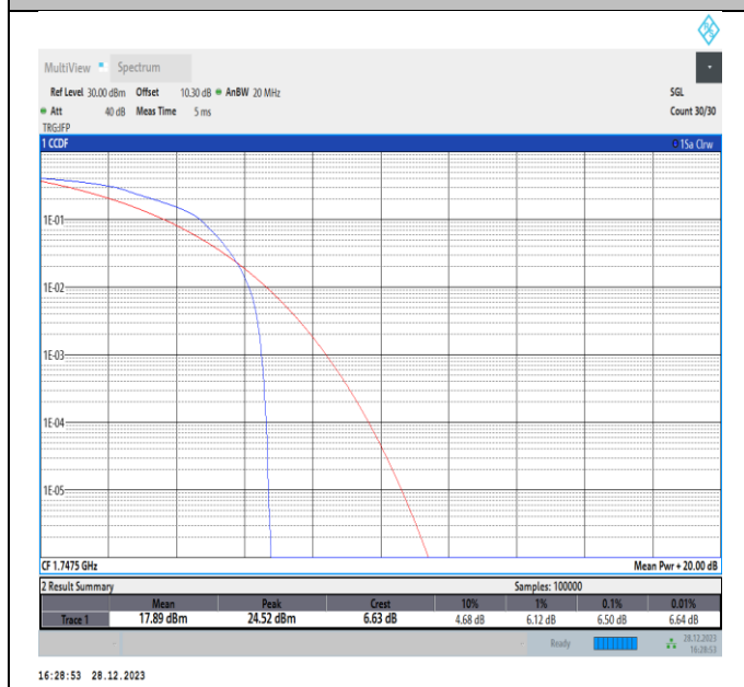
Band4-15MHz-16QAM-20325-PASS
