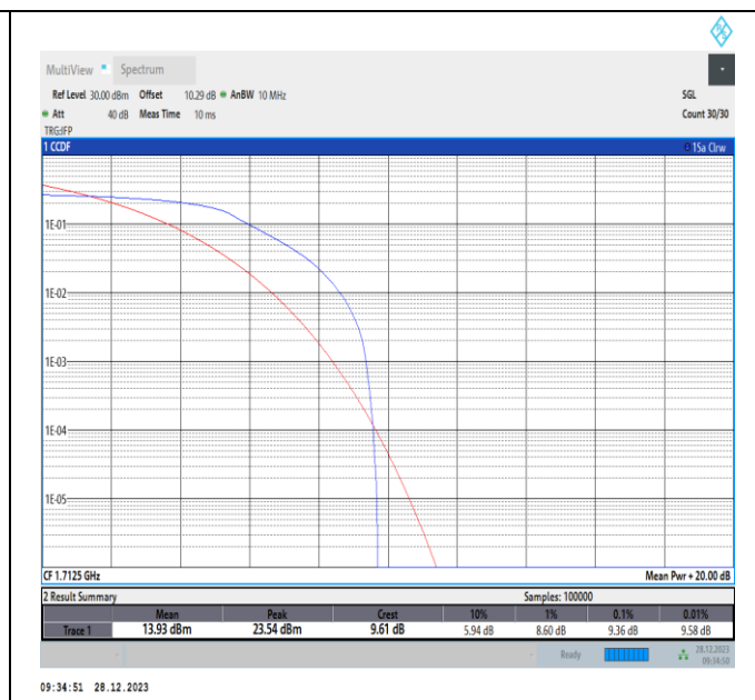
Band4-5MHz-QPSK-19975-PASS
