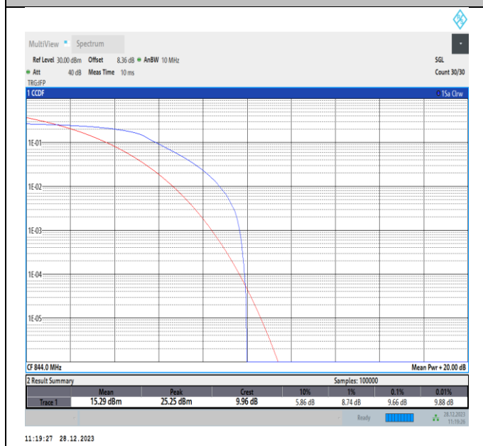
Band5-10MHz-QPSK-20600-PASS
