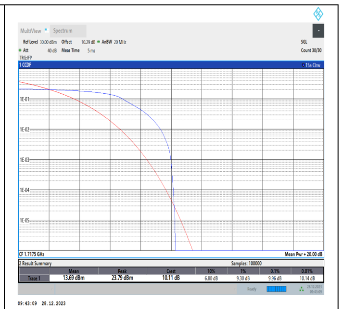
Band4-15MHz-QPSK-20025-PASS
