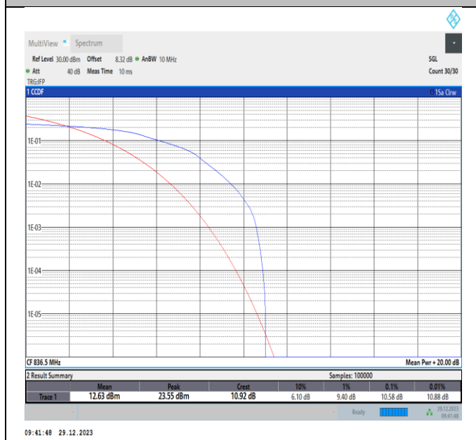
Band5-1.4MHz-16QAM-20525-PASS
