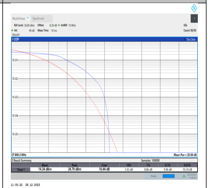
Band5-1.4MHz-QPSK-20643-PASS
