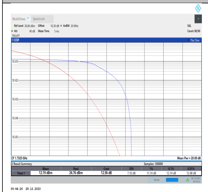
Band4-15MHz-QPSK-20175-PASS
