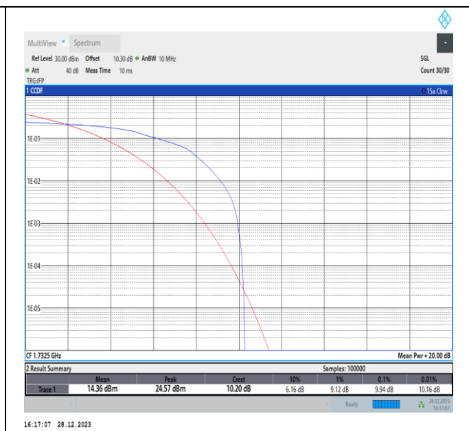
Band4-5MHz-16QAM-20175-PASS
