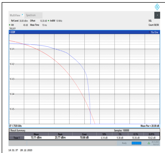
Band4-3MHz-16QAM-20385-PASS
