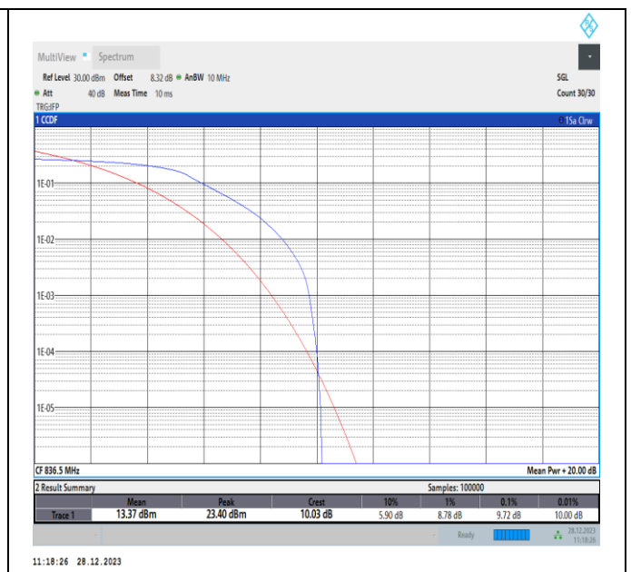
Band5-10MHz-QPSK-20525-PASS
