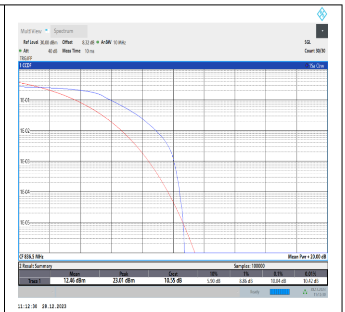
Band5-3MHz-QPSK-20525-PASS
