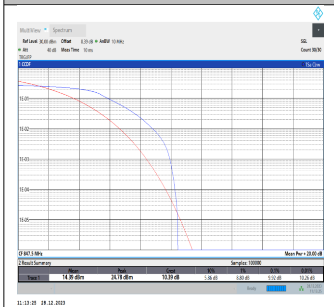
Band5-3MHz-QPSK-20635-PASS
