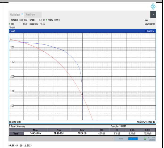
Band5-10MHz-16QAM-20450-PASS
