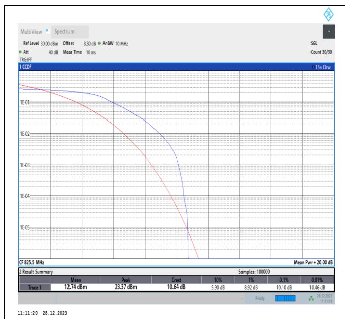
Band5-3MHz-QPSK-20415-PASS
