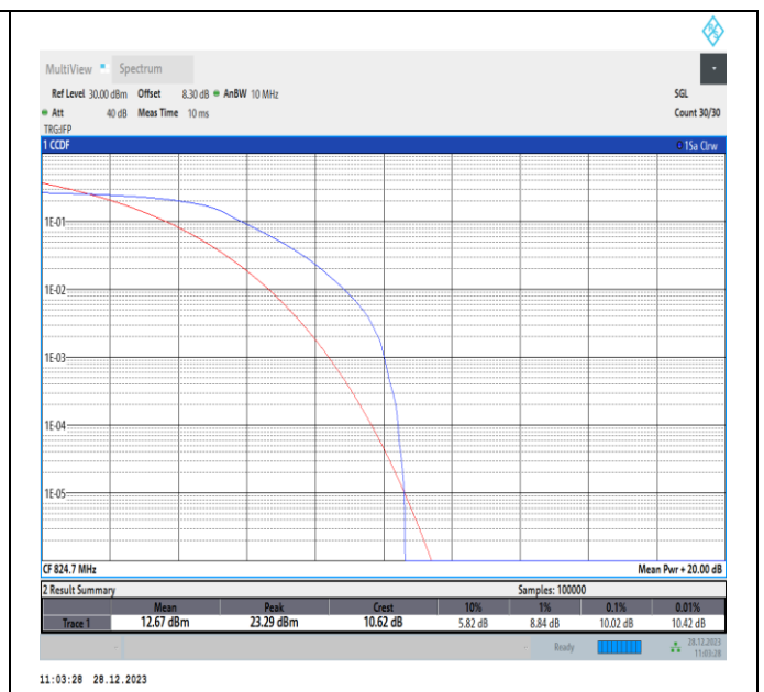
Band5-1.4MHz-QPSK-20407-PASS
