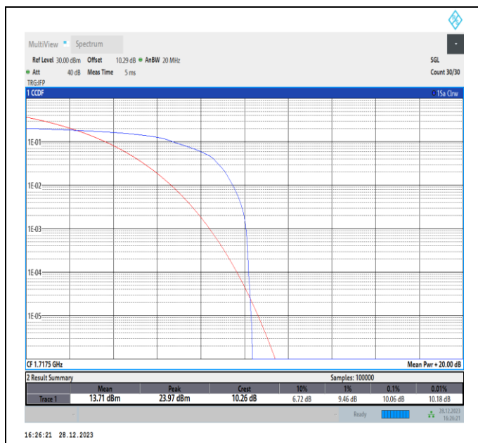
Band4-15MHz-16QAM-20025-PASS
