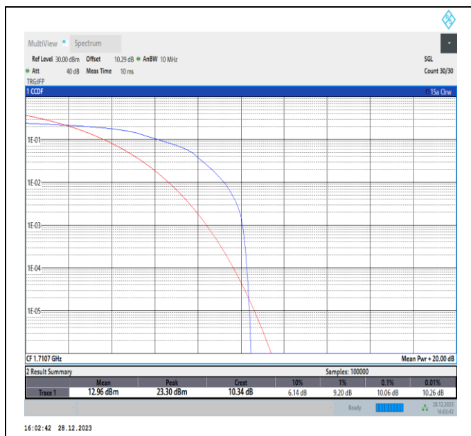
Band4-1.4MHz-16QAM-19957-PASS
