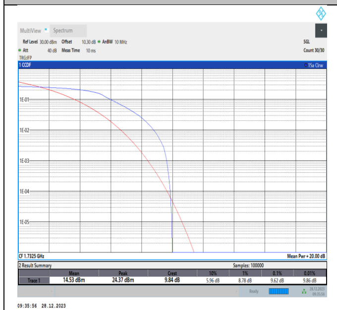
Band4-5MHz-QPSK-20175-PASS
