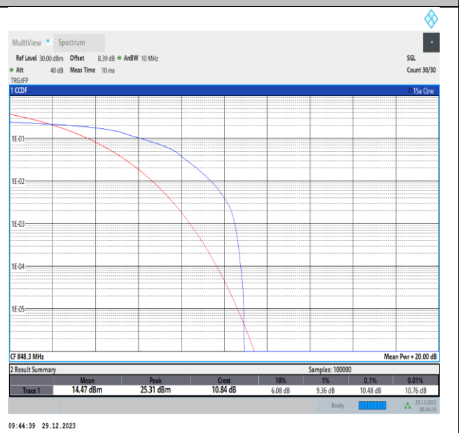
Band5-1.4MHz-16QAM-20643-PASS
