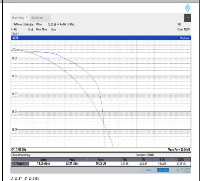
Band4-1.4MHz-QPSK-20393-PASS
