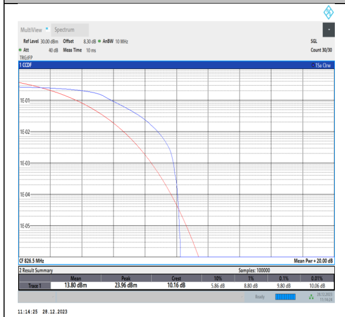
Band5-5MHz-QPSK-20425-PASS
