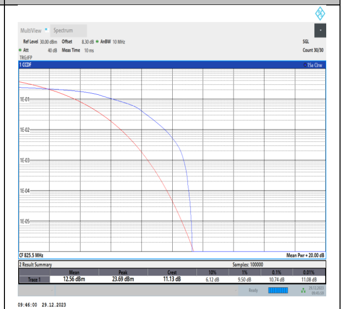
Band5-3MHz-16QAM-20415-PASS
