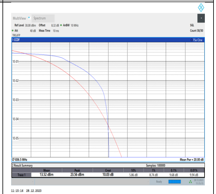
Band5-5MHz-QPSK-20525-PASS
