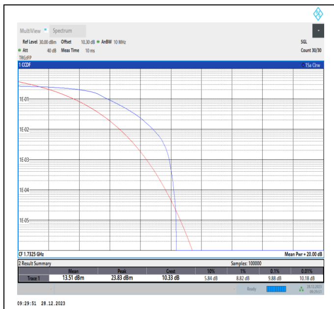
Band4-3MHz-QPSK-20175-PASS
