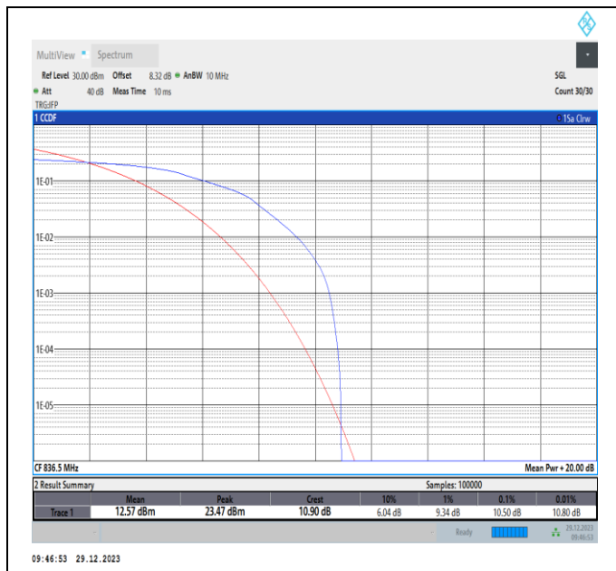
Band5-3MHz-16QAM-20525-PASS
