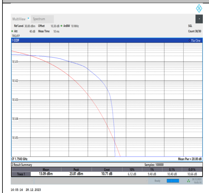
Band4-1.4MHz-16QAM-20393-PASS
