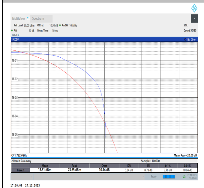
Band4-1.4MHz-QPSK-20175-PASS
