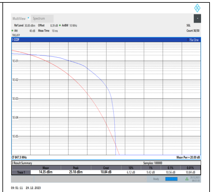
Band5-3MHz-16QAM-20635-PASS
