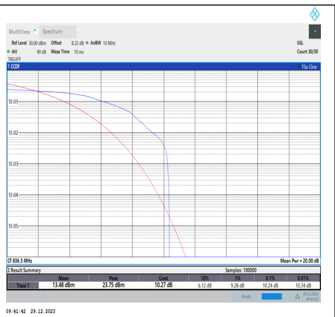
Band5-1.4MHz-16QAM-20525-PASS
