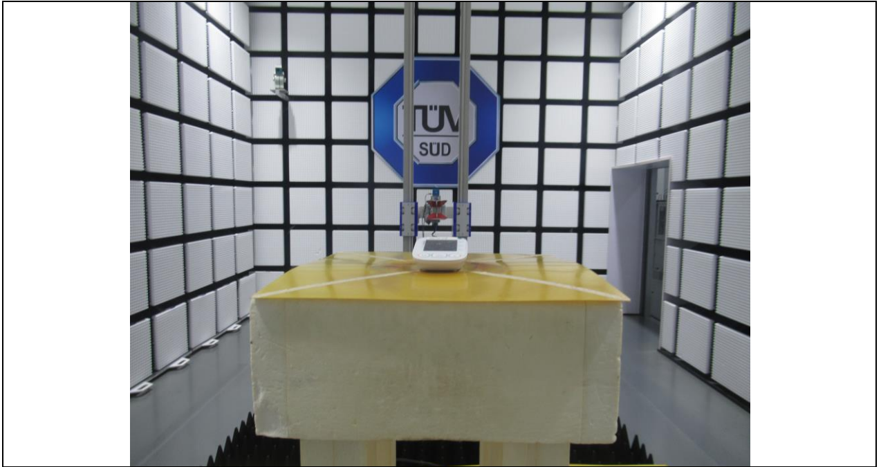
Details of: Radiated Emission test (1-18GHz)
