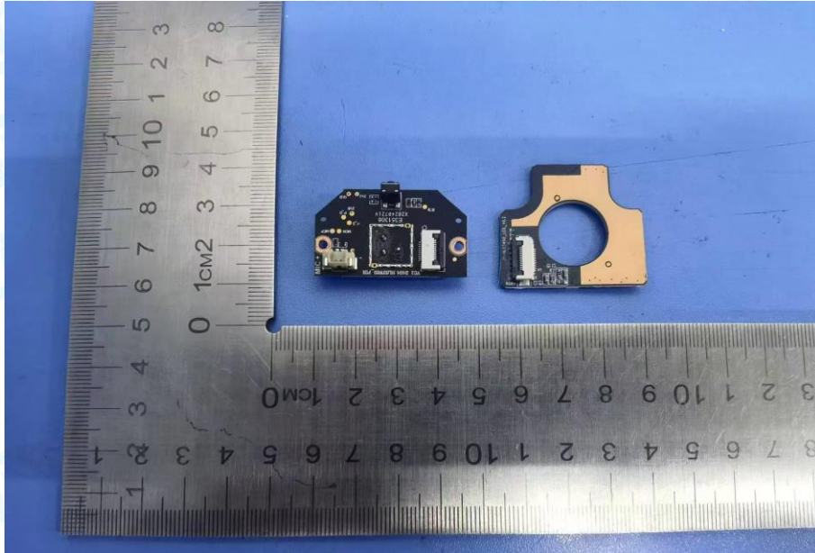
Photo 22 Internal of EUT
