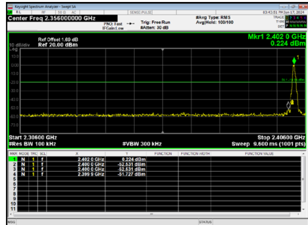
Band-edge Emission
