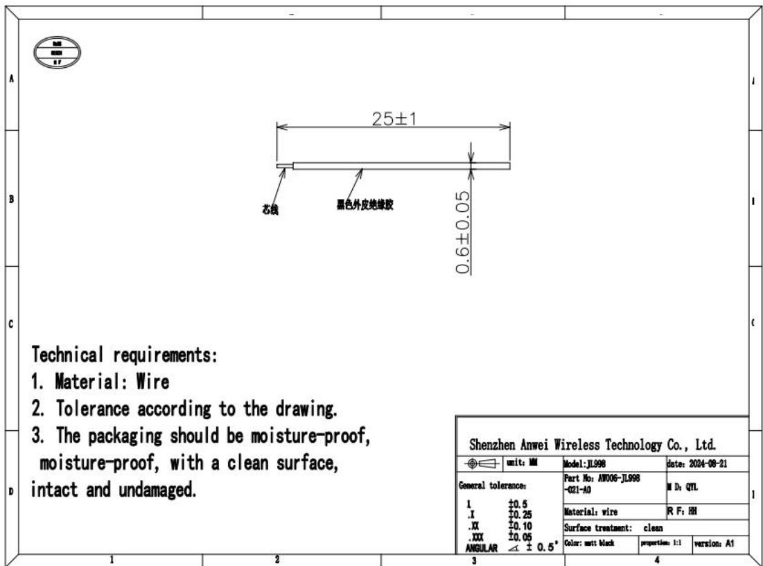
BT Antenna
