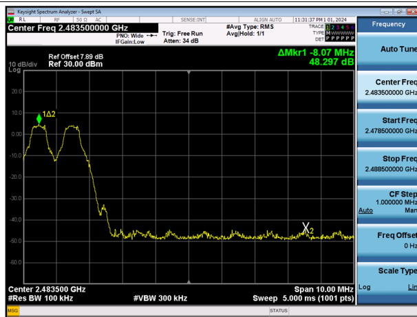
GFSK(with hopping) Band Edge(CH.78)
