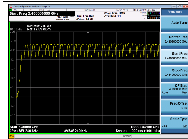
GFSK Number of Channels (2.4 GHz - 2.441 GHz)
