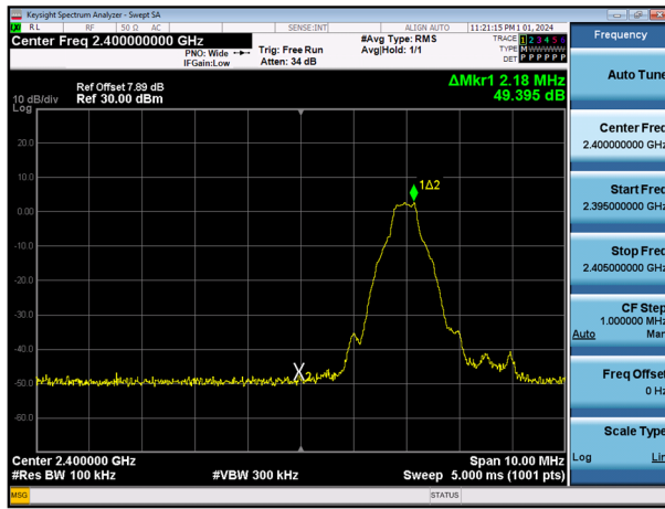
GFSK(with hopping) Band Edge(CH.0)
