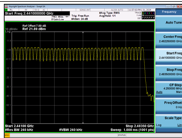
GFSK Number of Channels (2.441 GHz - 2.483.5 GHz)
