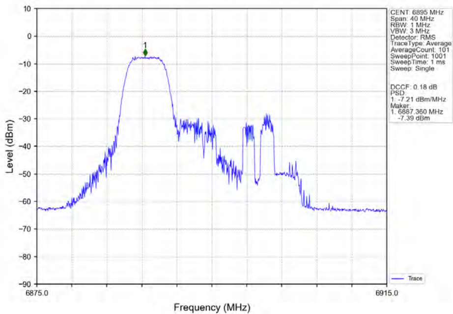
802.11ax(HEW20)_LCH_6895MHz_RU52-Ant5_NTNV
