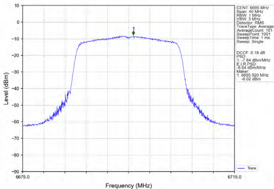
802.11ax(HEW20)_MCH_6695MHz_SU_ / Ant5_NTNV
