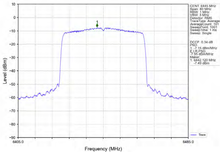
802.11ax(HEW40)_LCH_6445MHz_SU_/_MIMO_NTNV
