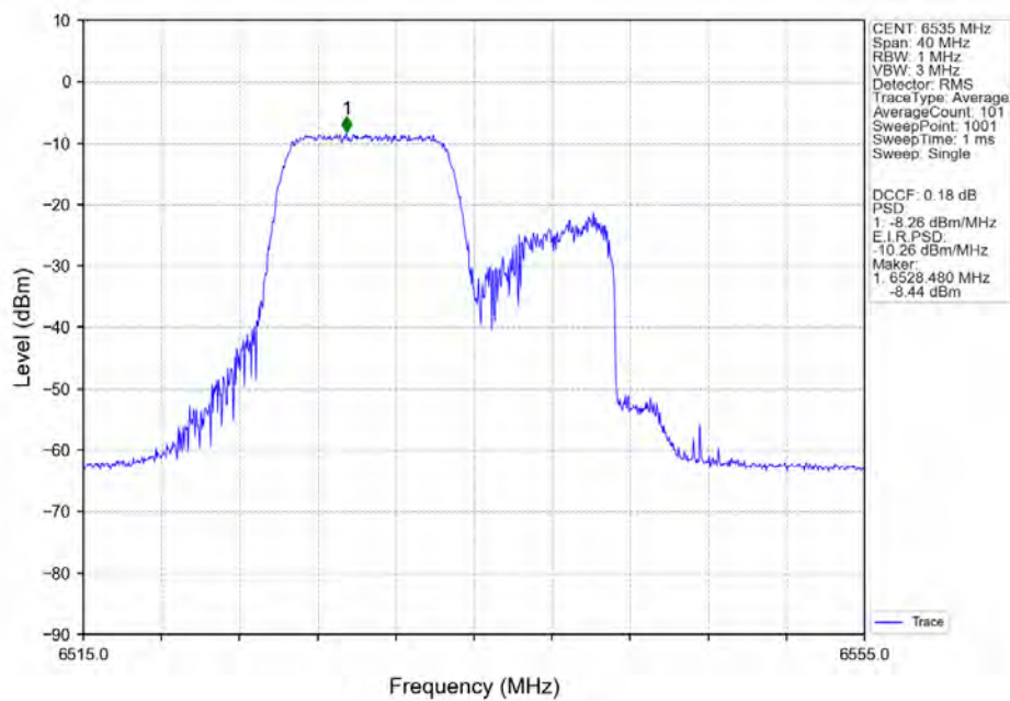
802.11ax(HEW20)_LCH_6535MHz_RU106-Ant4_NTNV
