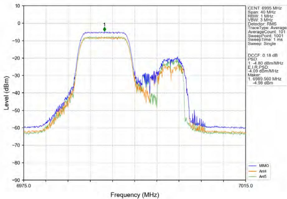
802.11ax(HEW20)_MCH_6995MHz_RU106-MIMO_NTNV
