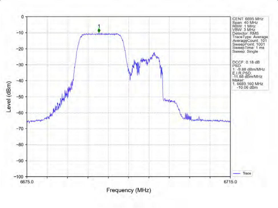
802.11ax(HEW20)_MCH_6695MHz_RU106-Ant4_NTNV
