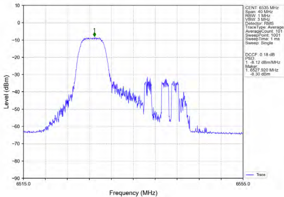
802.11ax(HEW20)_LCH_6535MHz_RU52-Ant5_NTNV
