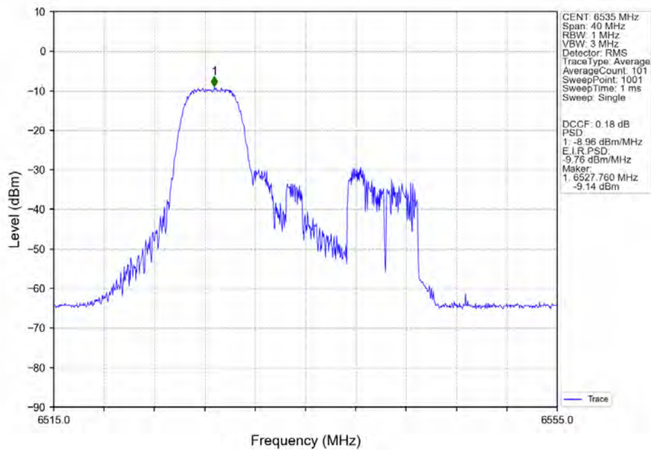
802.11ax(HEW20)_LCH_6535MHz_RU52-Ant5_NTNV
