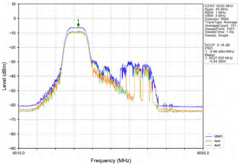
802.11ax(HEW20)_LCH_6535MHz_RU106-Ant4_NTNV
