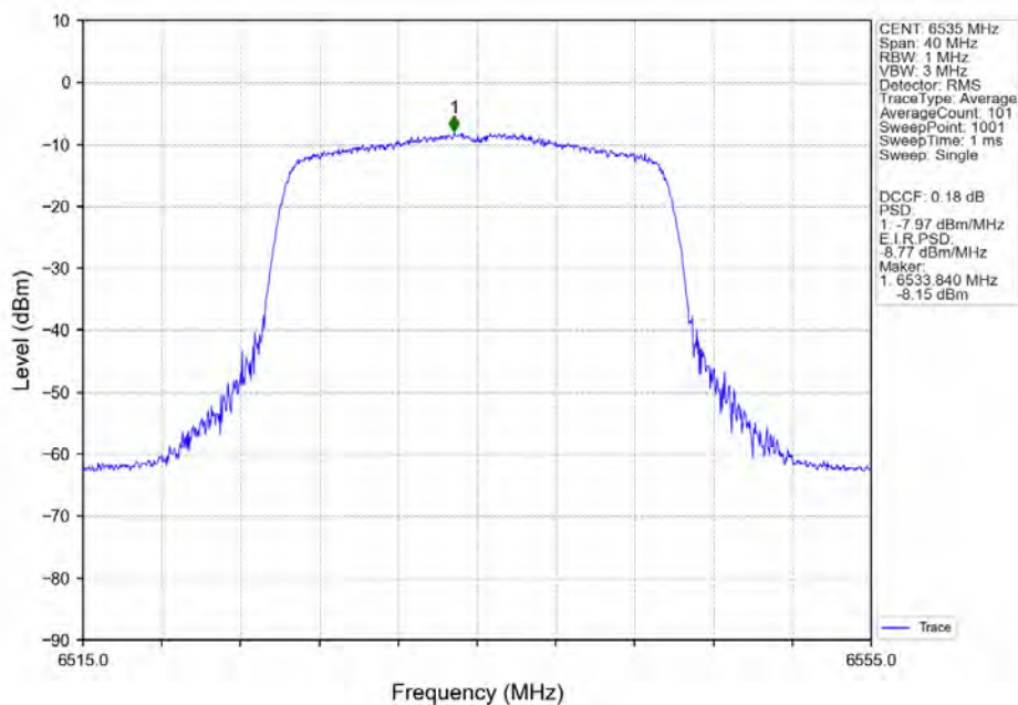
802.11ax(HEW20)_LCH_6535MHz_SU_/_Ant5_NTNV
