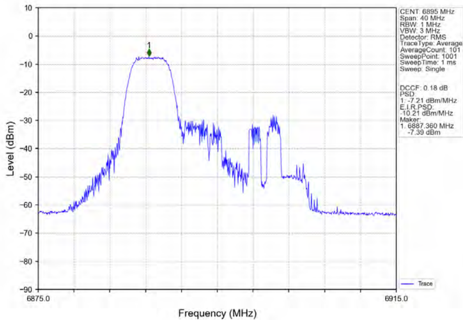
802.11ax(HEW20)_LCH_6895MHz_RU52-Ant5_NTNV
