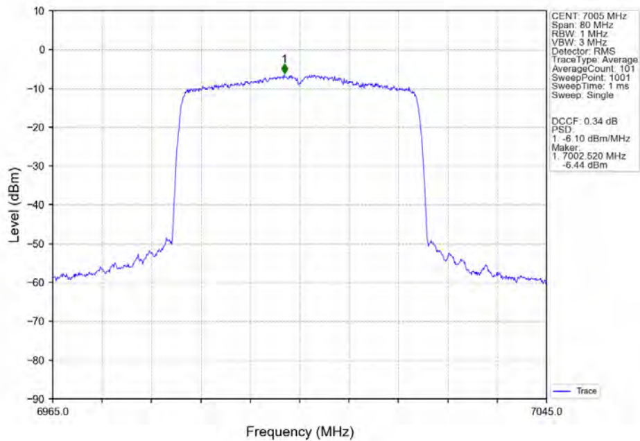
802.11ax(HEW40)_MCH_7005MHz_SU_/_Ant5_NTNV
