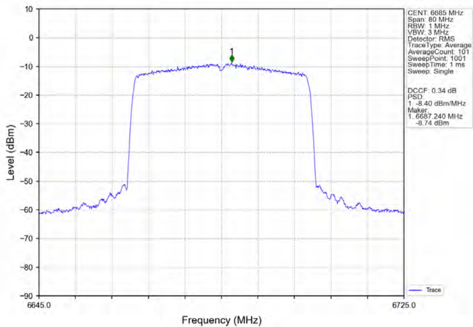
802.11ax(HEW40)_MCH_6685MHz_SU_/_Ant5_NTNV
