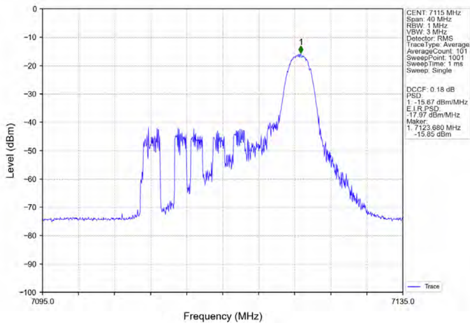
802.11ax(HEW20)_HCH_7115MHz_RU26-MIMO_NTNV
