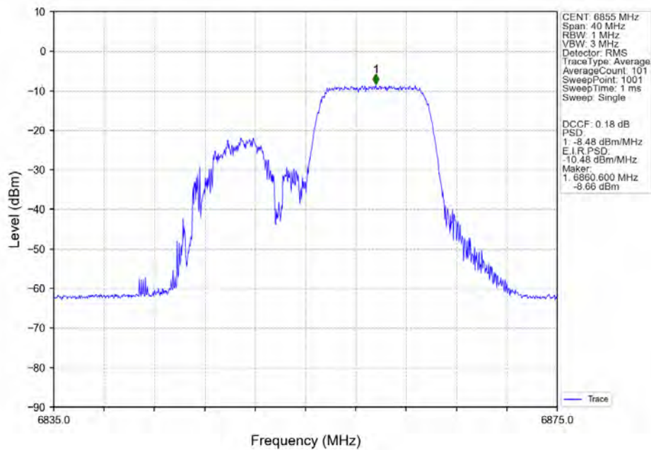
802.11ax(HEW20)_HCH_6855MHz_RU106-Ant4_NTNV
