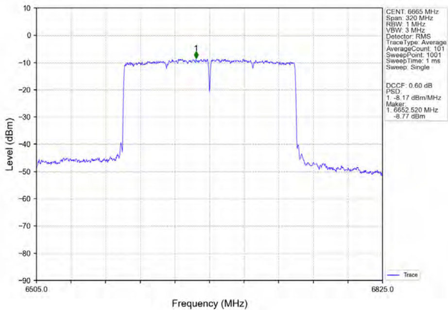
802.11ax(HEW160)_MCH_6665MHz_SU_/_Ant4_NTNV
