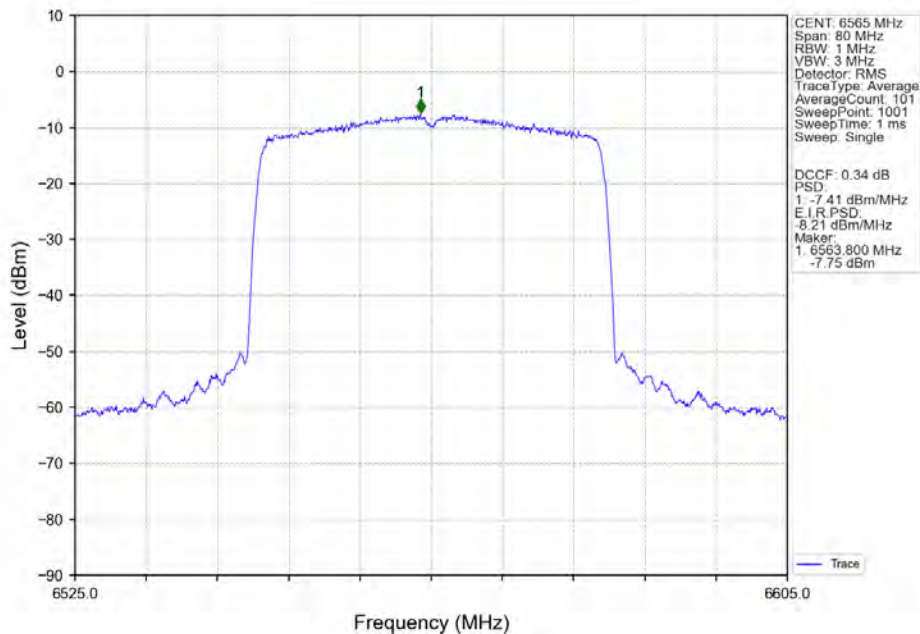
802.11ax(HEW40)_LCH_6565MHz_SU_/_MIMO_NTNV
