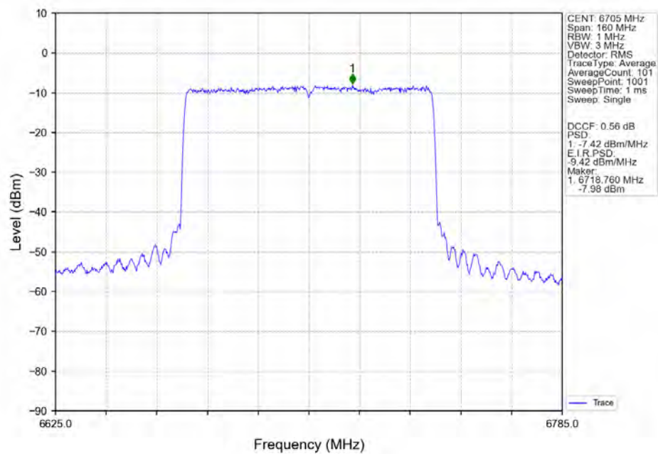
802.11ax(HEW80)_MCH_6705MHz_SU_ / Ant4_NTNV
