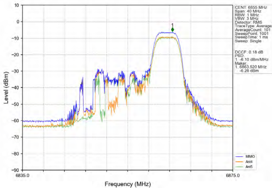
802.11ax(HEW20)_HCH_6855MHz_RU106-Ant4_NTNV
