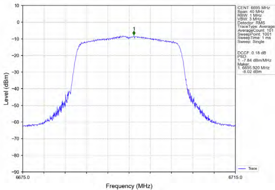
802.11ax(HEW20)_MCH_6695MHz_SU_ / Ant5_NTNV
