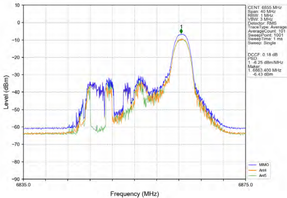
802.11ax(HEW20)_HCH_6855MHz_RU26-MIMO_NTNV
