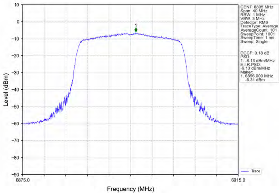
802.11ax(HEW20)_LCH_6895MHz_SU_/_Ant5_NTNV
