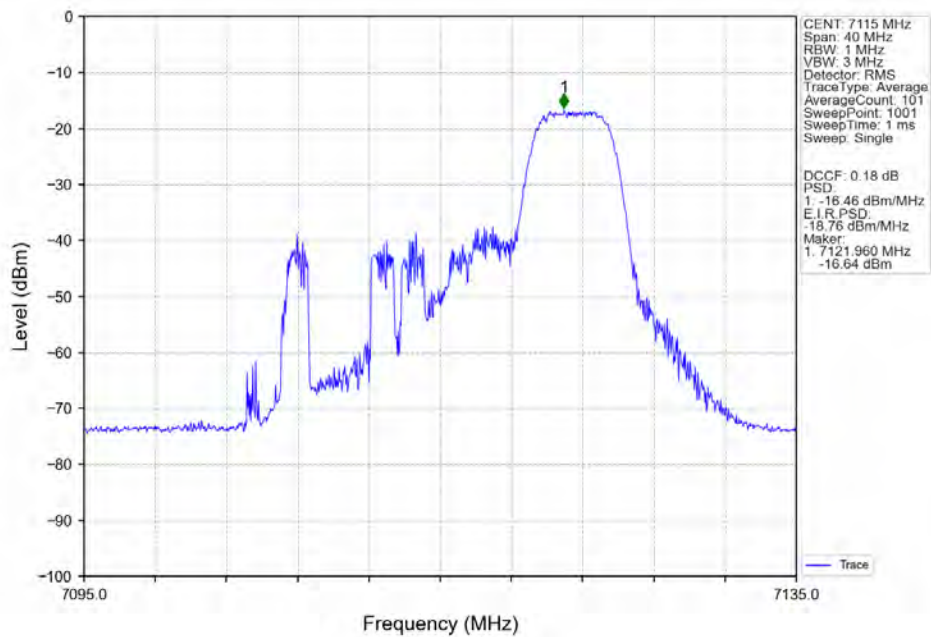
802.11ax(HEW20)_HCH_7115MHz_RU52-Ant5_NTNV
