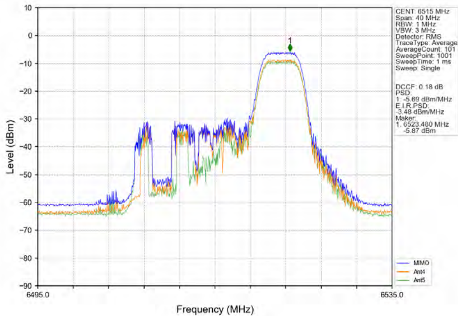
802.11ax(HEW20)_HCH_6515MHz_RU106-Ant4_NTNV
