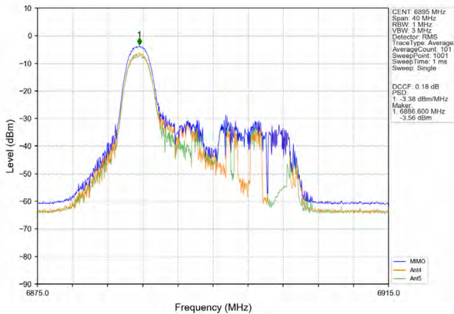
802.11ax(HEW20)_LCH_6895MHz_RU26-MIMO_NTNV
