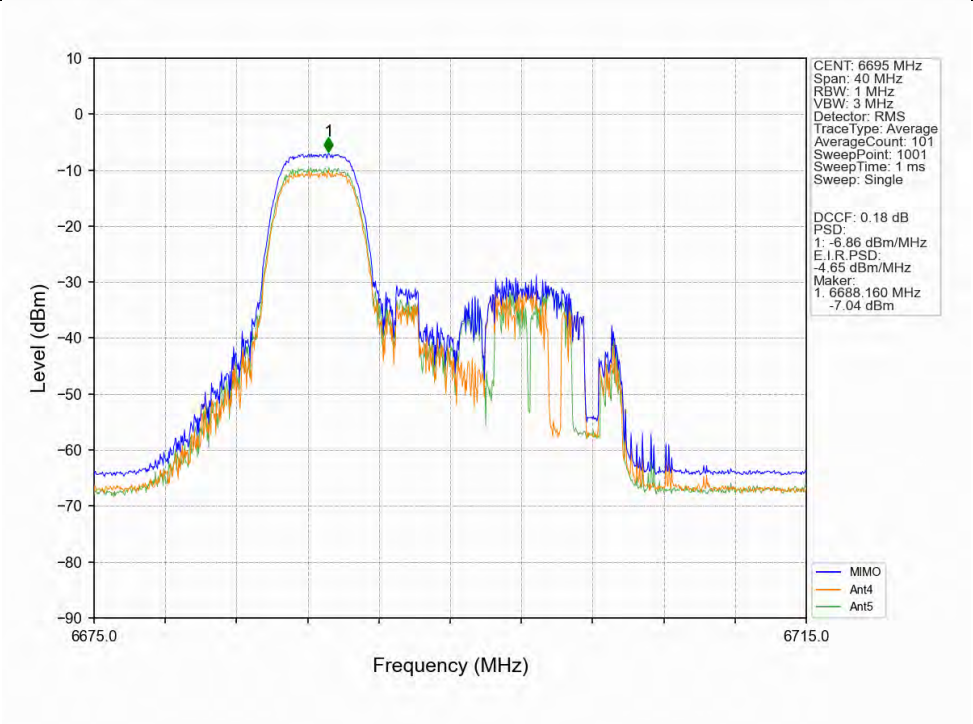
802.11ax(HEW20)_MCH_6695MHz_RU106-Ant4_NTNV
