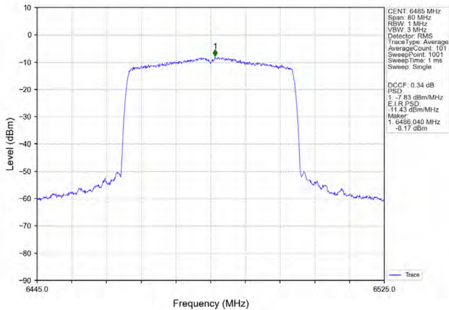
802.11ax(HEW40)_MCH_6485MHz_SU_/_Ant5_NTNV
