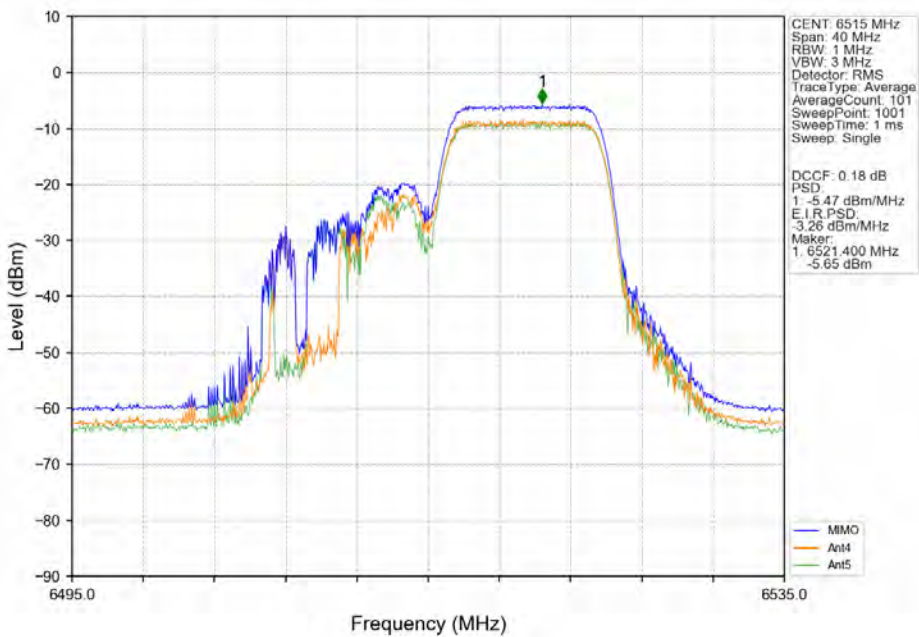
802.11ax(HEW20)_HCH_6515MHz_RU106-MIMO_NTNV
