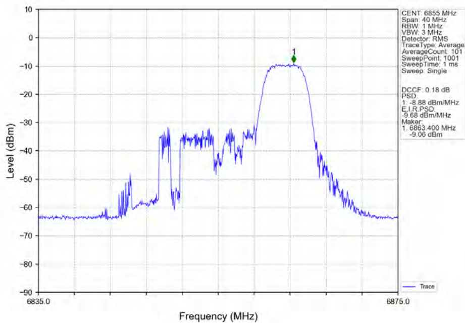
802.11ax(HEW20)_HCH_6855MHz_RU52-Ant5_NTNV
