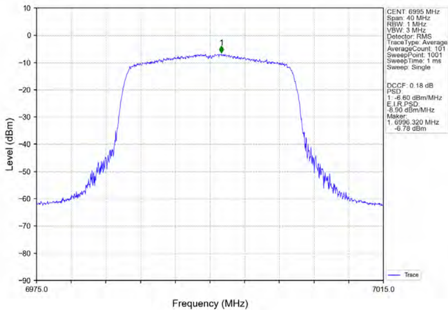
802.11ax(HEW20)_MCH_6995MHz_SU_ / _Ant5_NTNV
