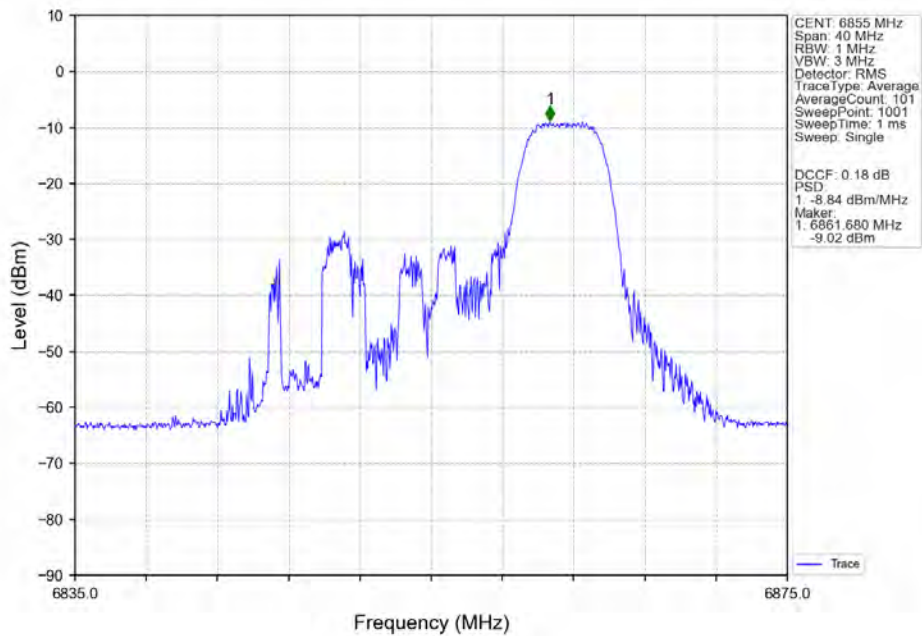
802.11ax(HEW20)_HCH_6855MHz_RU52-Ant5_NTNV
