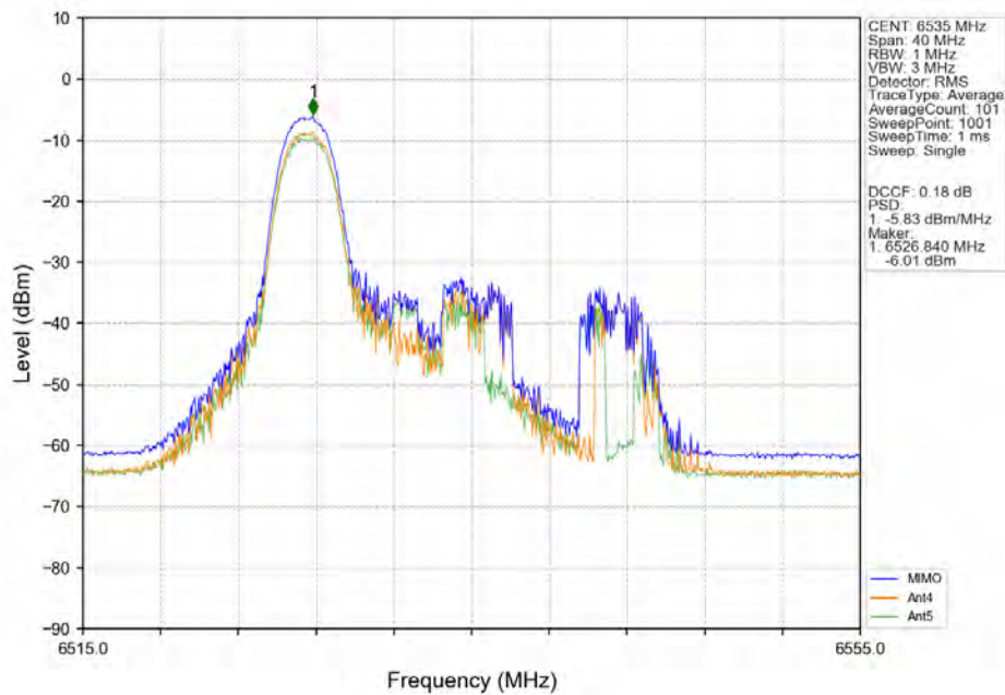
802.11ax(HEW20)_LCH_6535MHz_RU26-MIMO_NTNV
