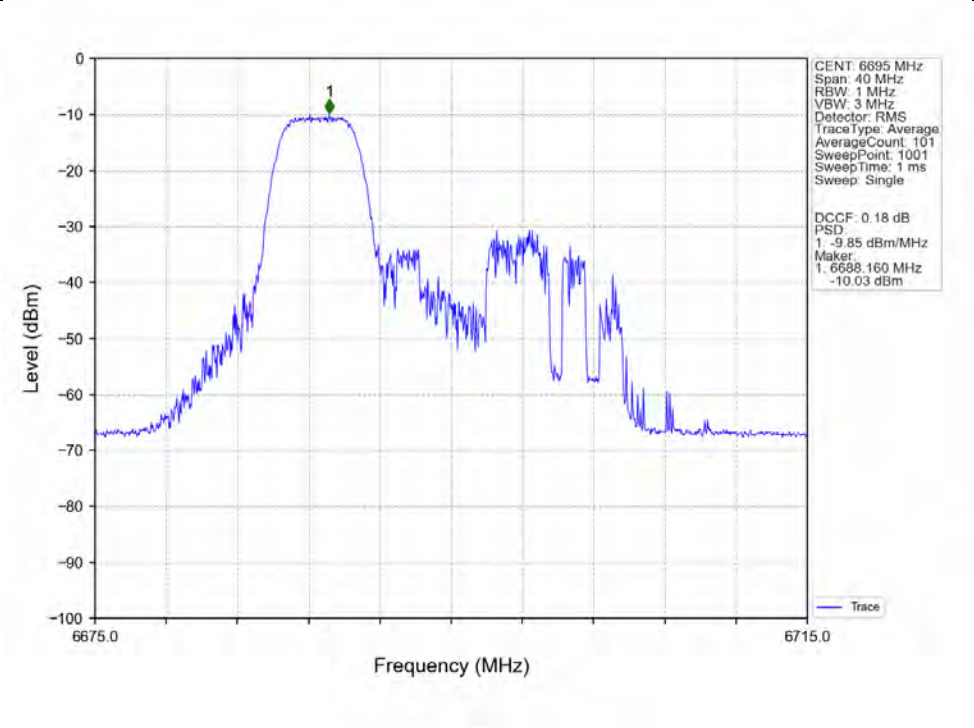
802.11ax(HEW20)_MCH_6695MHz_RU52-Ant5_NTNV
