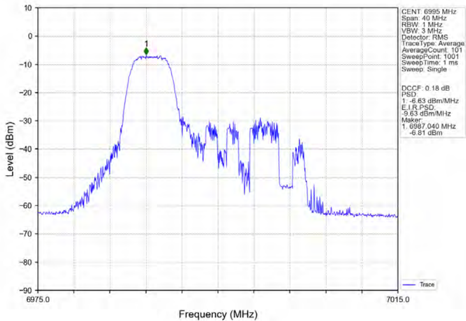
802.11ax(HEW20)_MCH_6995MHz_RU52-Ant5_NTNV
