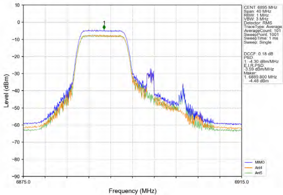
802.11ax(HEW20)_LCH_6895MHz_RU106-MIMO_NTNV
