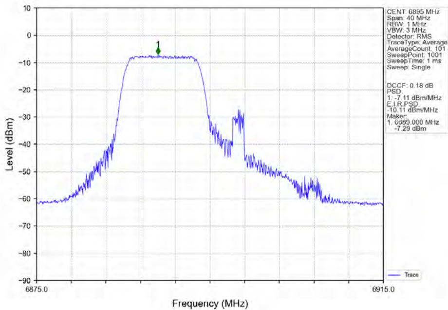
802.11ax(HEW20)_LCH_6895MHz_RU106-Ant4_NTNV
