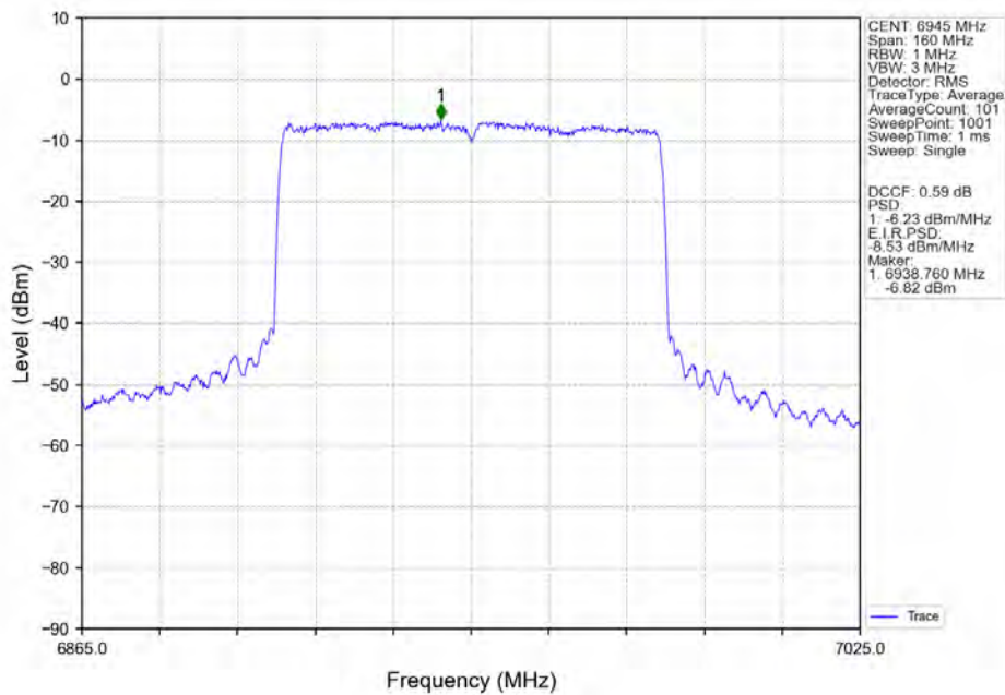
802.11ax(HEW80)_LCH_6945MHz_SU_/_Ant5_NTNV
