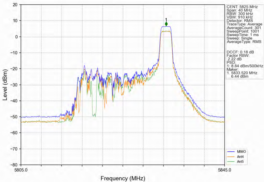
802.11ax(HEW20)_HCH_5825MHz_RU52-Ant4_NTNV
