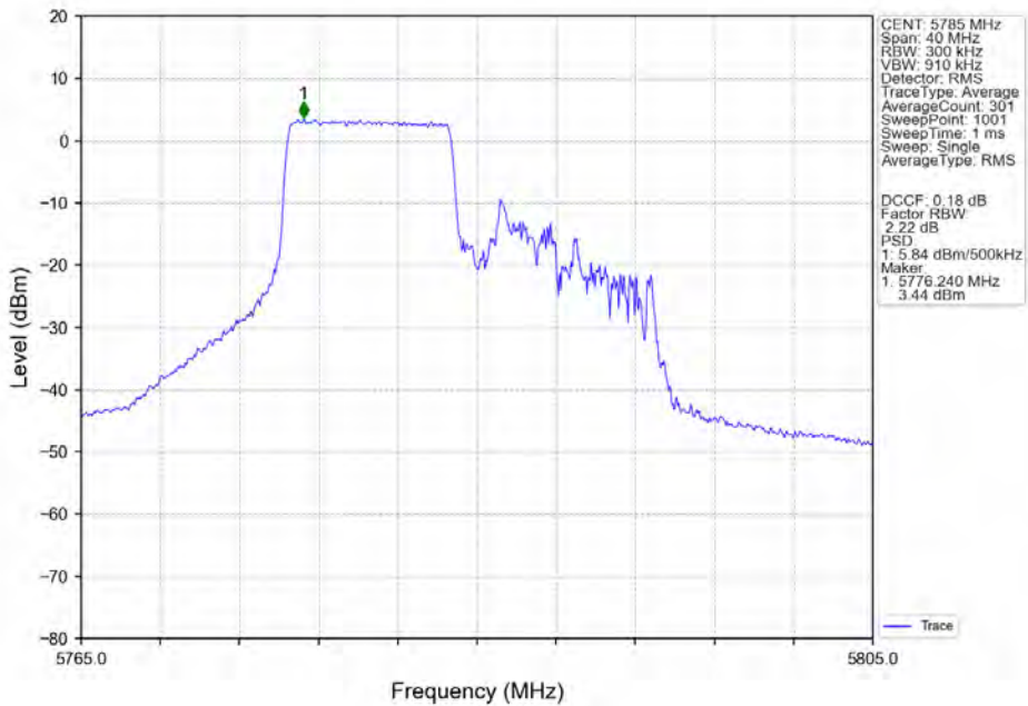
802.11ax(HEW20)_MCH_5785MHz_RU106-Ant5_NTNV
