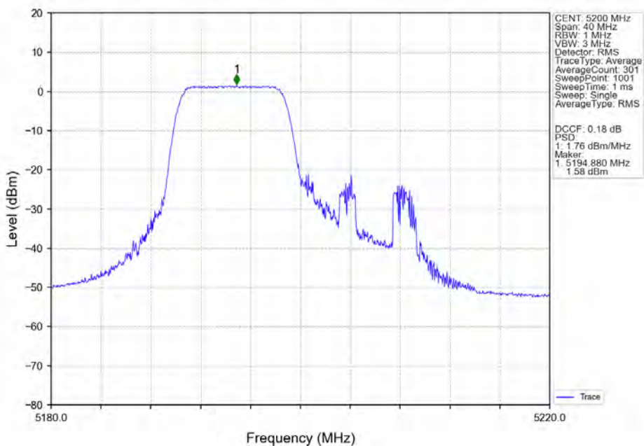
802.11ax(HEW20)_MCH_5200MHz_RU106-Ant5_NTNV
