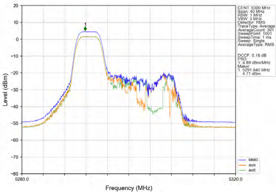
802.11ax(HEW20)_MCH_5300MHz_RU52-MIMO_NTNV
