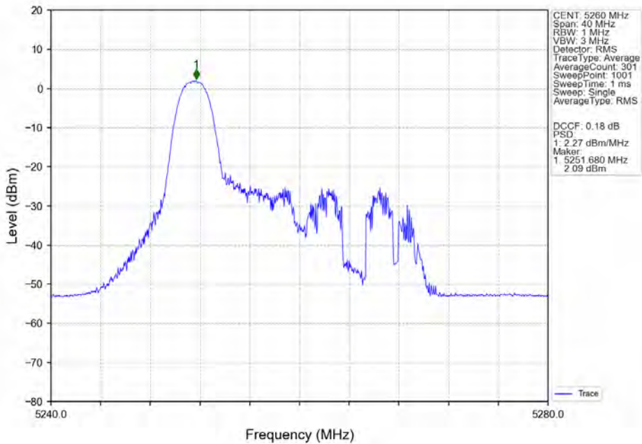
802.11ax(HEW20)_LCH_5260MHz_RU26-Ant5_NTNV
