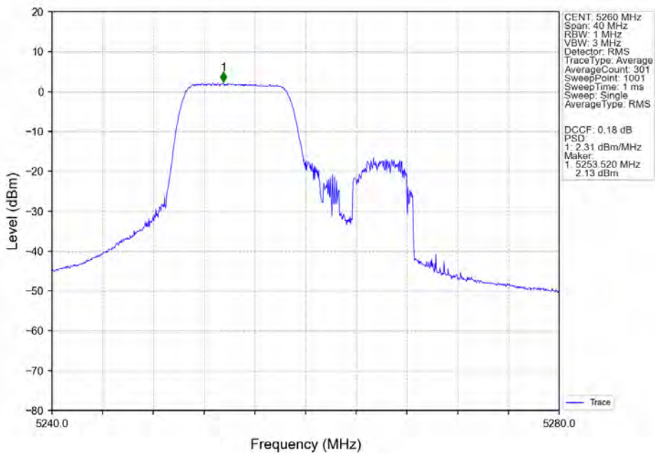
802.11ax(HEW20)_LCH_5260MHz_RU106-Ant5_NTNV
