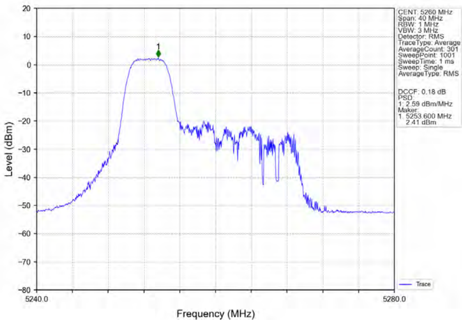
802.11ax(HEW20)_LCH_5260MHz_RU52-MIMO_NTNV
