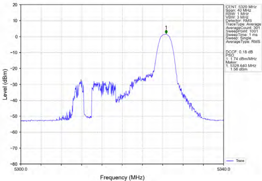
802.11ax(HEW20)_HCH_5320MHz_RU26-Ant5_NTNV
