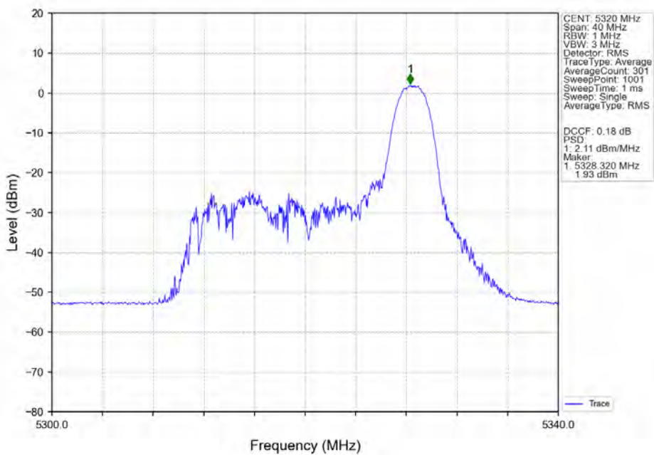
802.11ax(HEW20)_HCH_5320MHz_RU26-Ant5_NTNV
