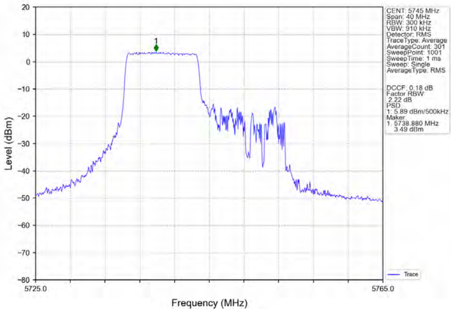
802.11ax(HEW20)_LCH_5745MHz_RU106-Ant5_NTNV
