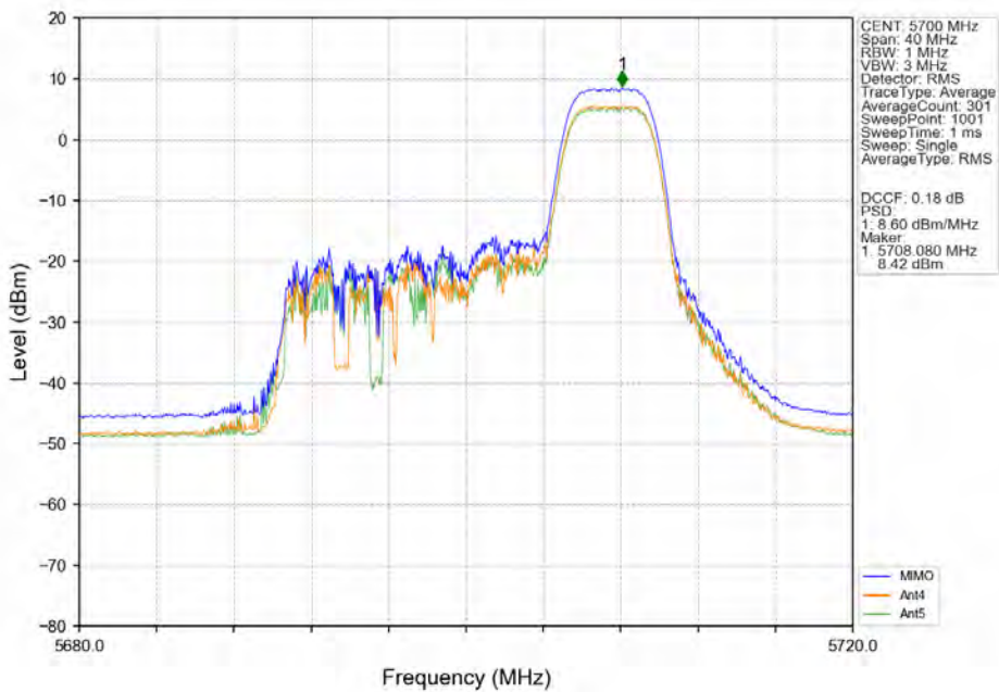
802.11ax(HEW20)_HCH_5700MHz_RU52-MIMO_NTNV
