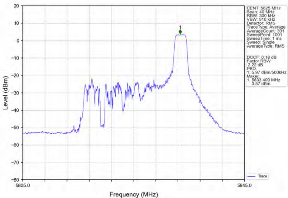
802.11ax(HEW20)_HCH_5825MHz_RU26-Ant5_NTNV
