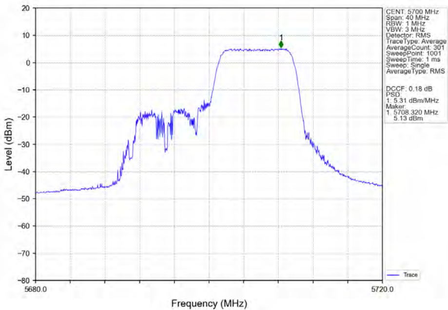
802.11ax(HEW20)_HCH_5700MHz_RU106-Ant5_NTNV
