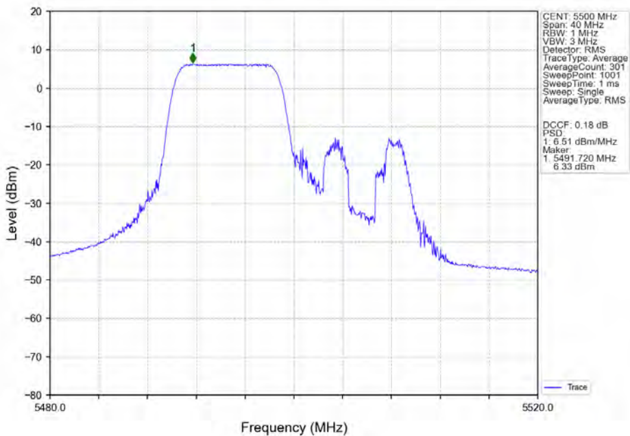
802.11ax(HEW20)_LCH_5500MHz_RU106-Ant5_NTNV
