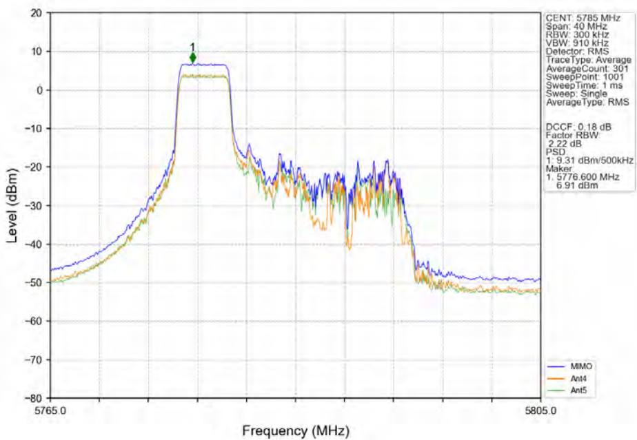
802.11ax(HEW20)_MCH_5785MHz_RU52-MIMO_NTNV
