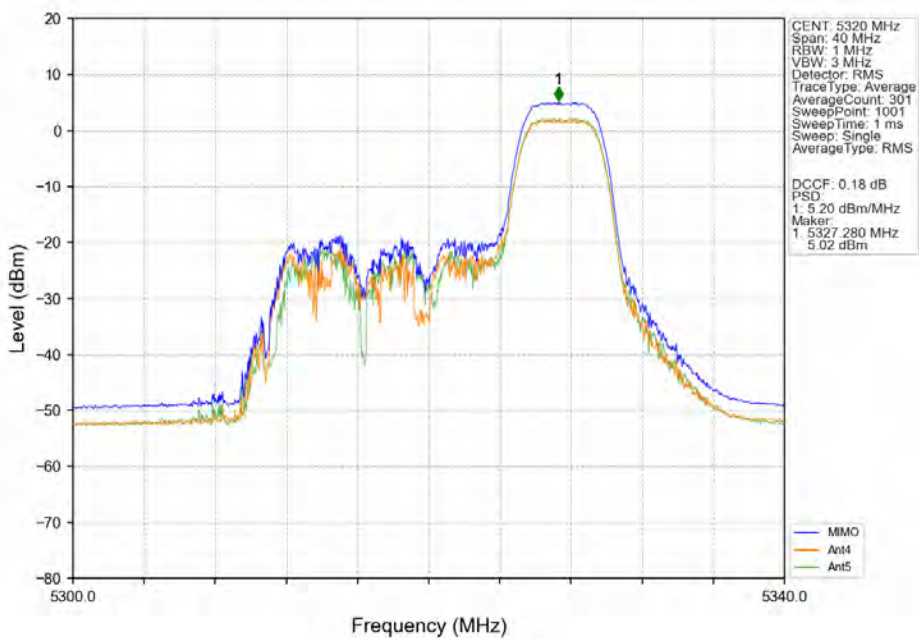
802.11ax(HEW20)_HCH_5320MHz_RU52-MIMO_NTNV
