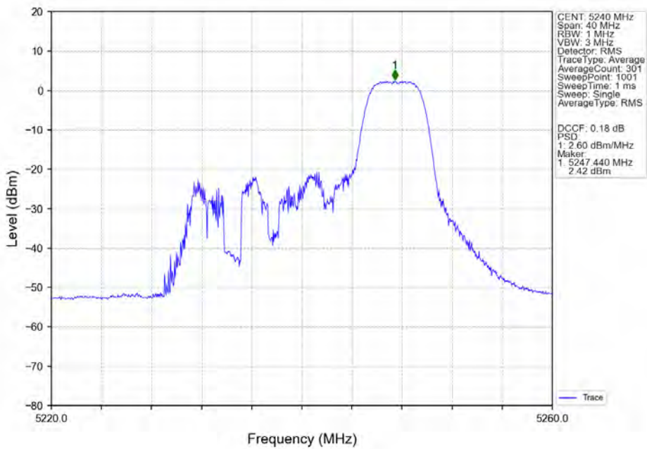
802.11ax(HEW20)_HCH_5240MHz_RU52-MIMO_NTNV
