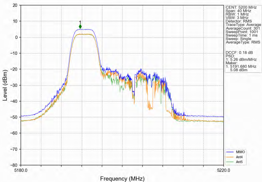
802.11ax(HEW20)_MCH_5200MHz_RU52-MIMO_NTNV
