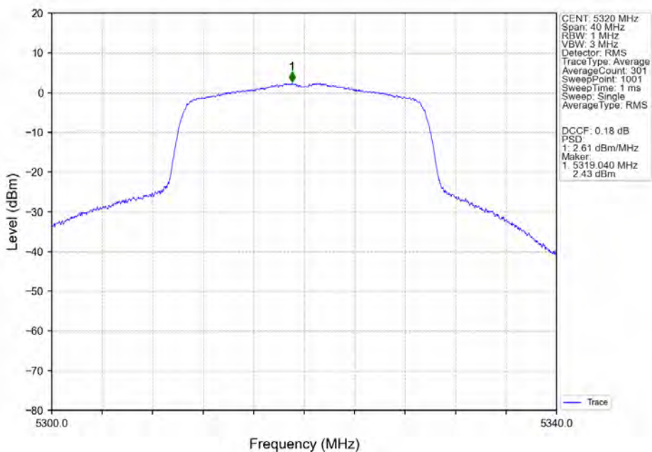
802.11ax(HEW20)_HCH_5320MHz_SU_ / Ant4_NTNV
