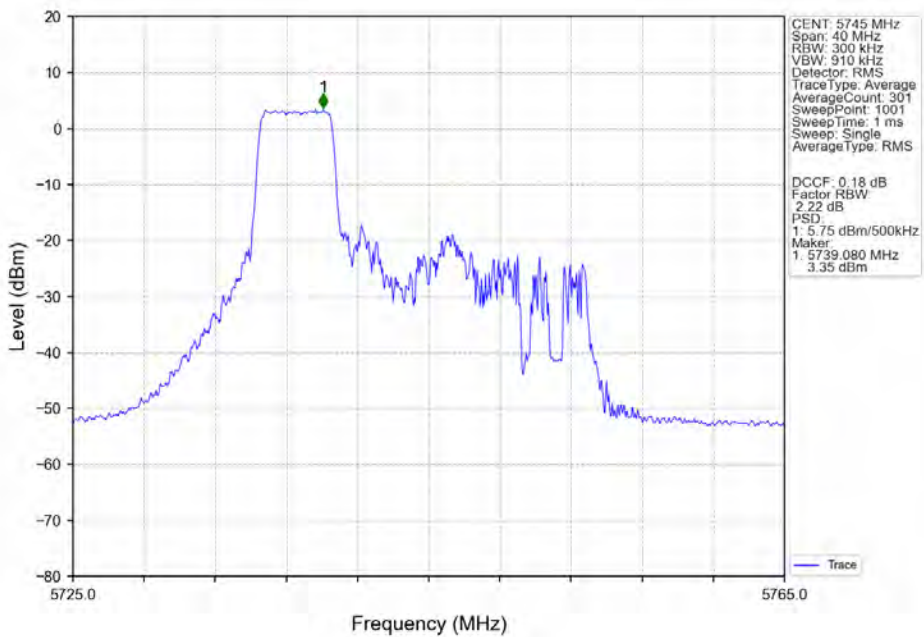
802.11ax(HEW20)_LCH_5745MHz_RU52-Ant4_NTNV
