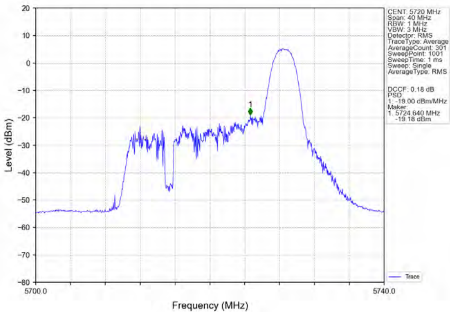
802.11ax(HEW20)_HCH_5720MHz_RU26-Ant5_NTNV
