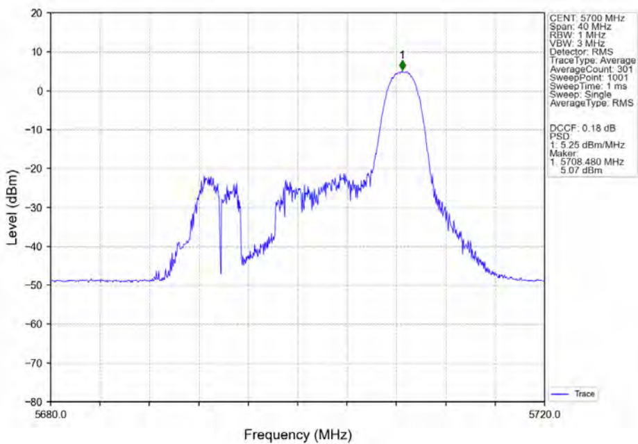
802.11ax(HEW20)_HCH_5700MHz_RU26-Ant5_NTNV
