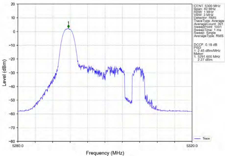
802.11ax(HEW20)_MCH_5300MHz_RU26-Ant5_NTNV
