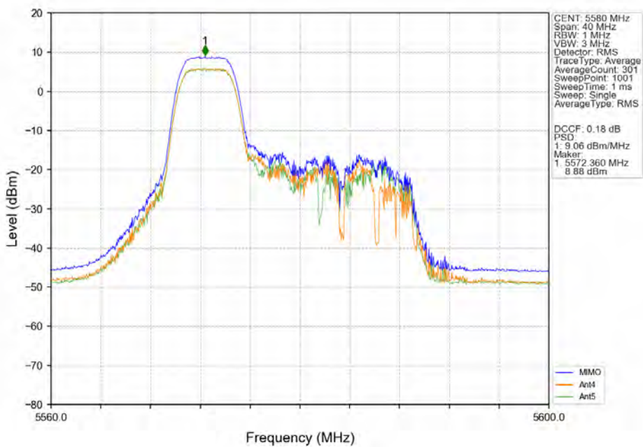
802.11ax(HEW20)_MCH_5580MHz_RU52-MIMO_NTNV
