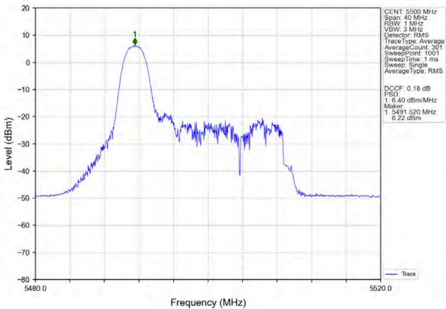
802.11ax(HEW20)_LCH_5500MHz_RU26-Ant5_NTNV
