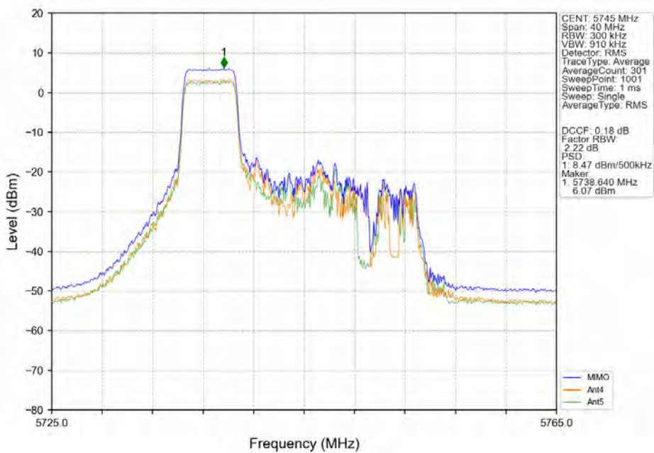
802.11ax(HEW20)_LCH_5745MHz_RU52-MIMO_NTNV
