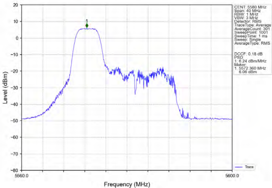
802.11ax(HEW20)_MCH_5580MHz_RU52-MIMO_NTNV
