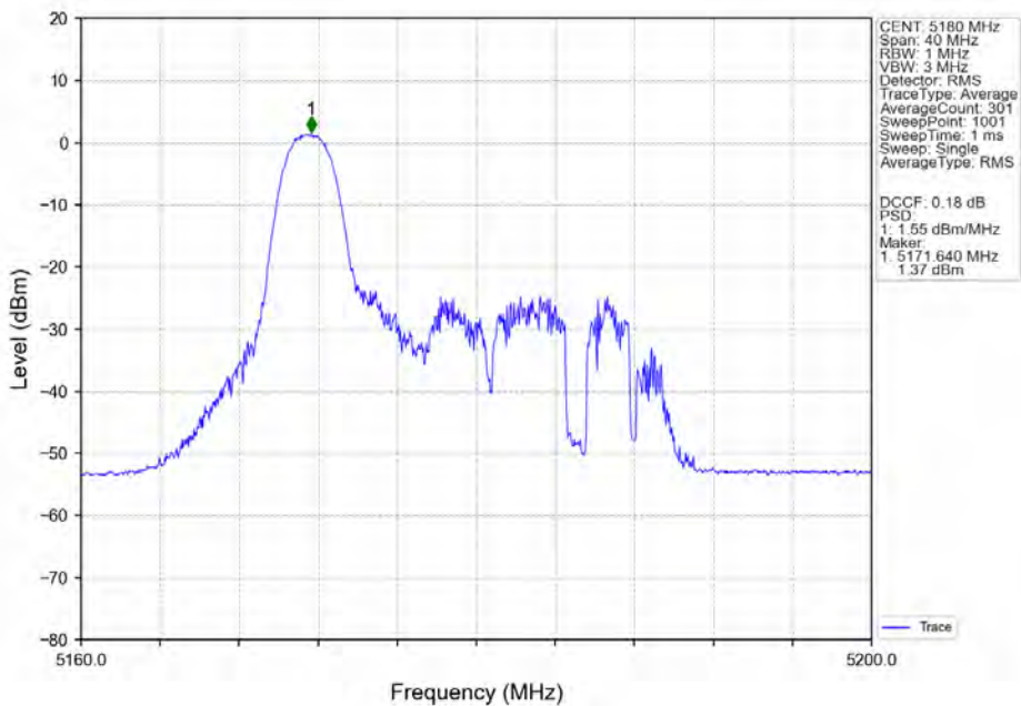
802.11ax(HEW20)_LCH_5180MHz_RU26-Ant5_NTNV
