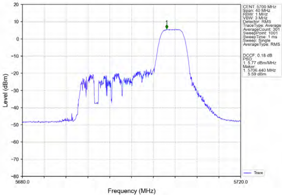
802.11ax(HEW20)_HCH_5700MHz_RU52-Ant4_NTNV
