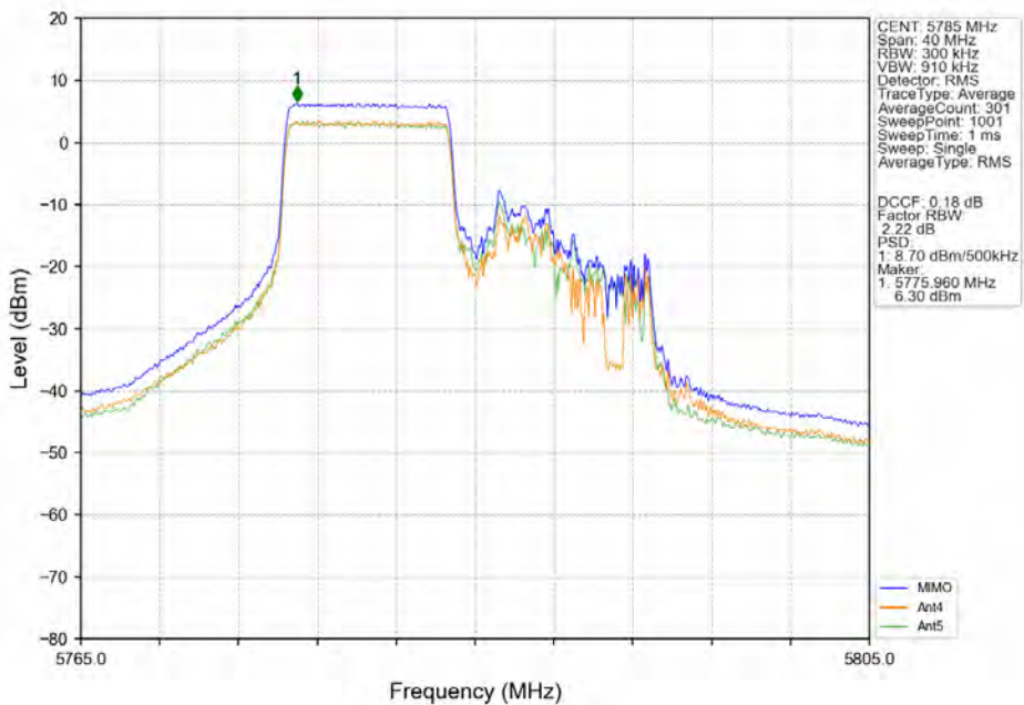
802.11ax(HEW20)_MCH_5785MHz_SU / Ant4_NTNV
