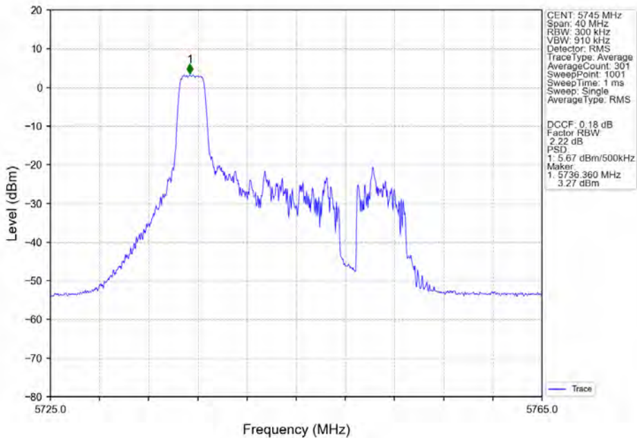
802.11ax(HEW20)_LCH_5745MHz_RU26-Ant5_NTNV
