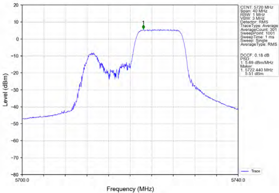
802.11ax(HEW20)_HCH_5720MHz_RU106-Ant5_NTNV
