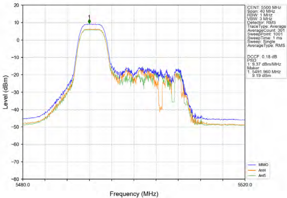
802.11ax(HEW20)_LCH_5500MHz_RU52-MIMO_NTNV
