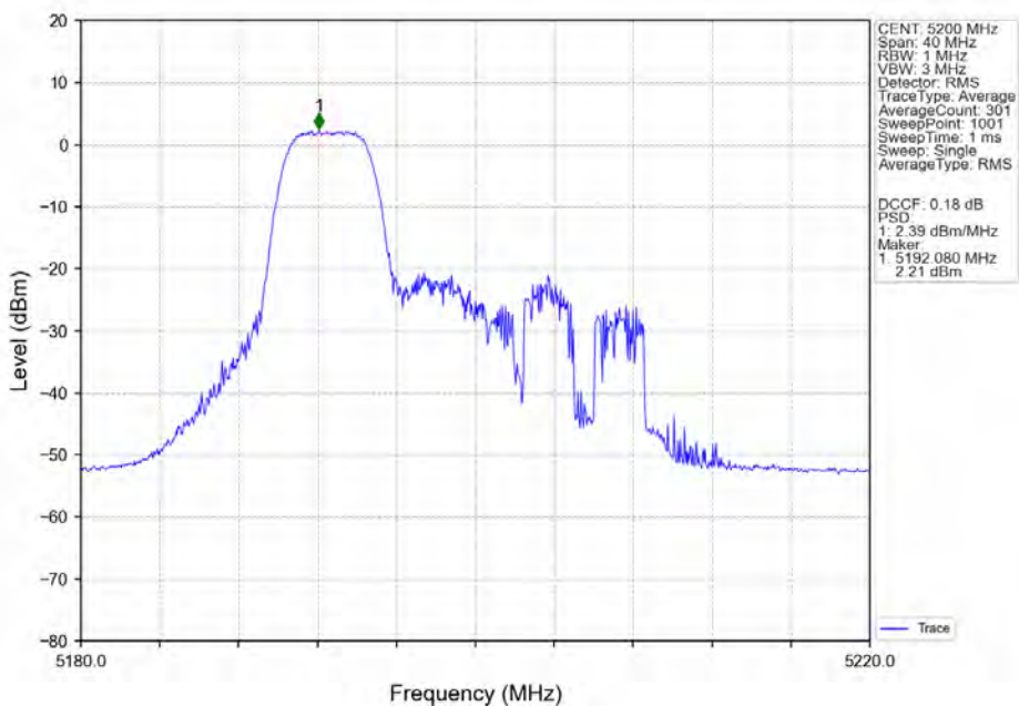
802.11ax(HEW20)_MCH_5200MHz_RU52-Ant4_NTNV
