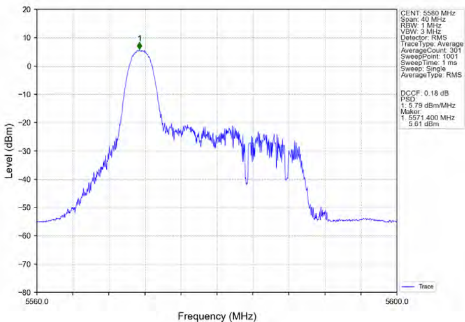
802.11ax(HEW20)_MCH_5580MHz_RU26-Ant5_NTNV
