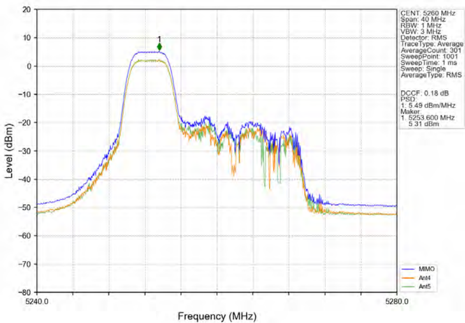
802.11ax(HEW20)_LCH_5260MHz_RU52-MIMO_NTNV
