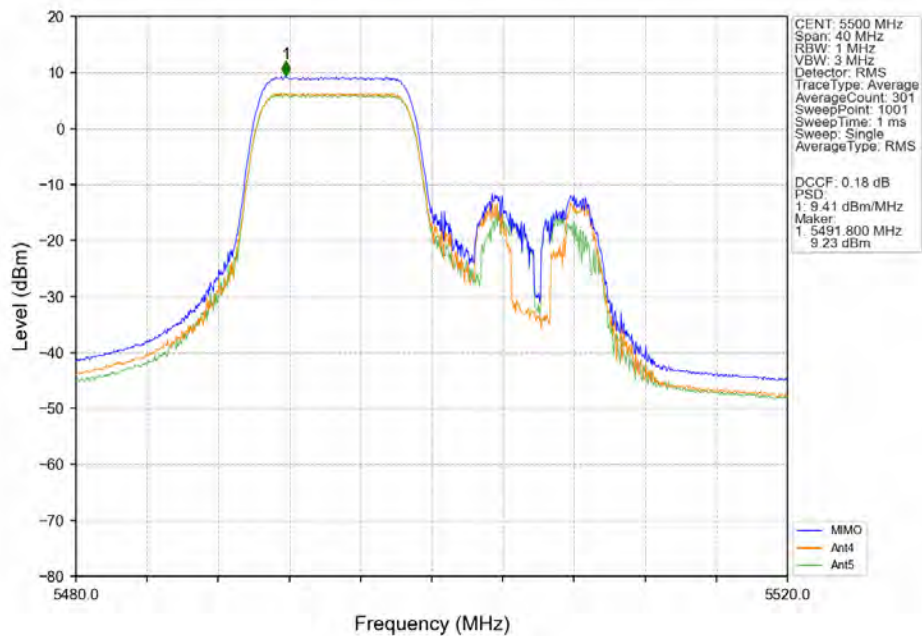
802.11ax(HEW20)_LCH_5500MHz_SU / Ant4_NTNV
