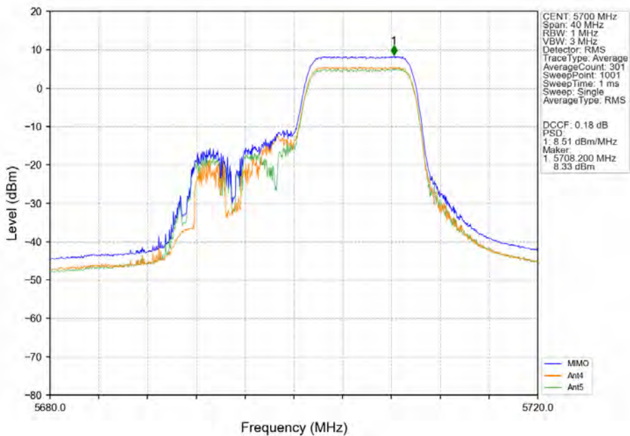
802.11ax(HEW20)_HCH_5700MHz_SU / Ant4_NTNV
