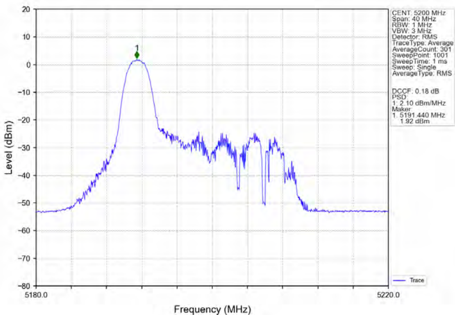
802.11ax(HEW20)_MCH_5200MHz_RU26-Ant5_NTNV
