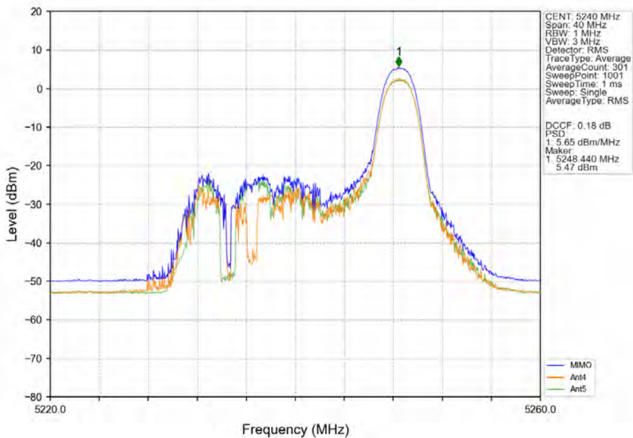
802.11ax(HEW20)_HCH_5240MHz_RU52-Ant4_NTNV
