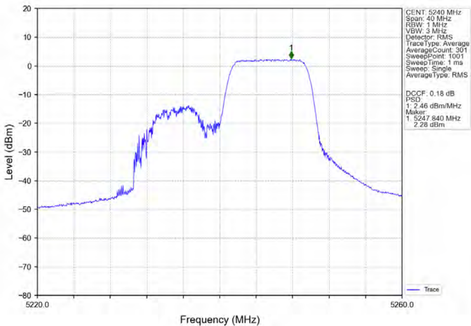
802.11ax(HEW20)_HCH_5240MHz_RU106-Ant5_NTNV
