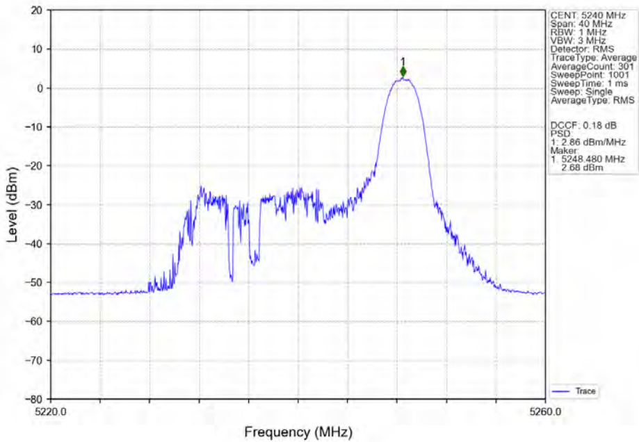
802.11ax(HEW20)_HCH_5240MHz_RU26-Ant5_NTNV
