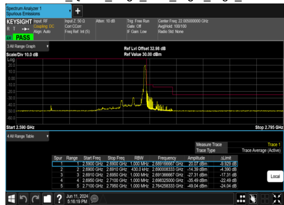
N41(20M)_DFT-s- OFDM_QPSK_Edge_1RB_Right_High_CH
