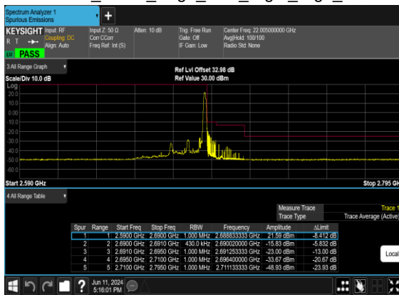
N41(20M)_DFT-s- OFDM_BPSK_Edge_1RB_Right_High_CH
