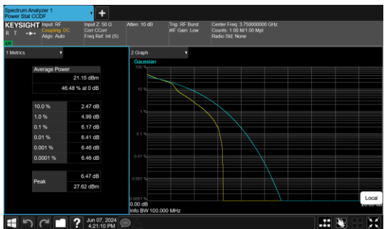
N78(80M)_DFT-s- OFDM_QPSK_Edge_1RB_Left_Mid_CH
