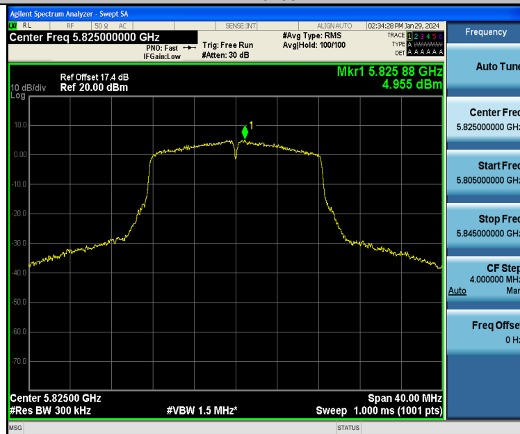
11A-Ant1-5825-PASS
