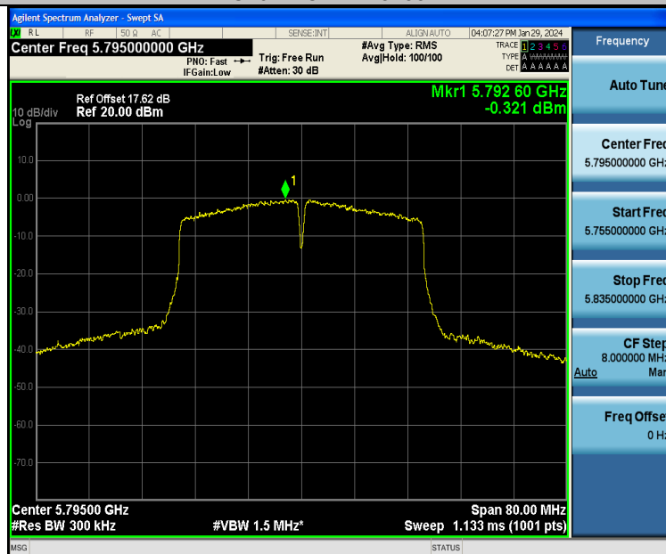
11AC40SISO-Ant1-5795-PASS
