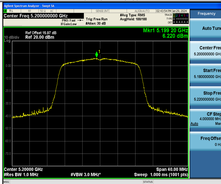
11N20SISO-Ant1-5200-PASS
