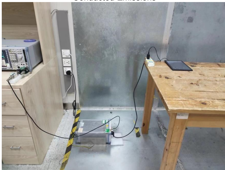
Conducted Emissions
