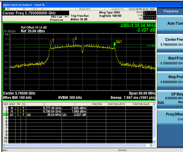
11N40SISO-Ant1-5795-PASS
