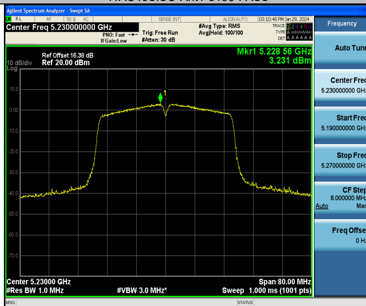
11N40SISO-Ant1-5230-PASS
