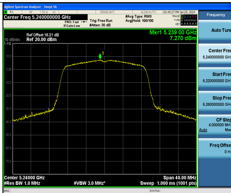
11N20SISO-Ant1-5240-PASS
