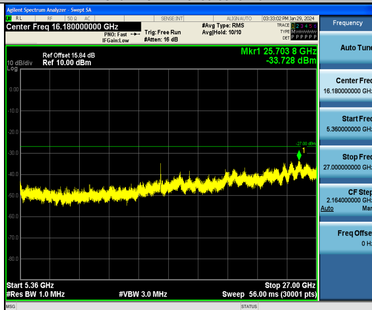
11AC20SISO-Ant1-5200-5360~27000-PASS
