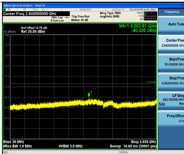
11A-Ant1-5745-30~5650-PASS
