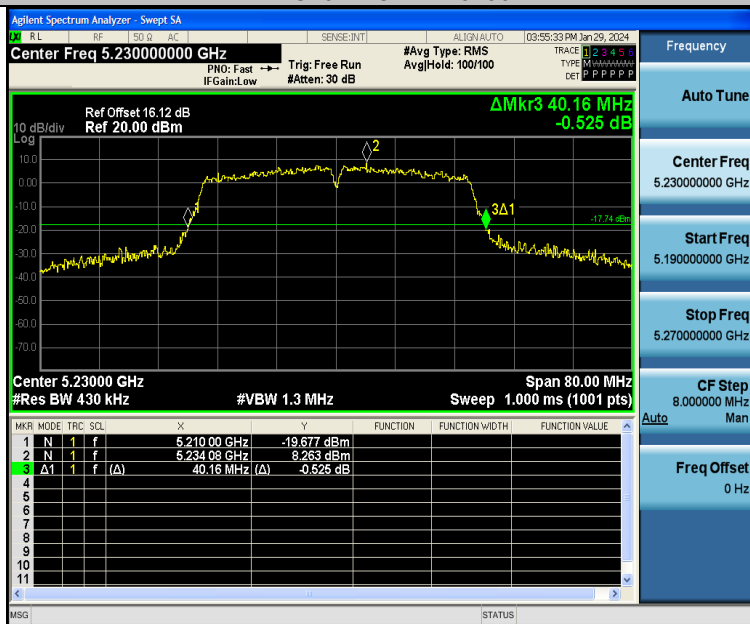
11AC40SISO-Ant1-5230
