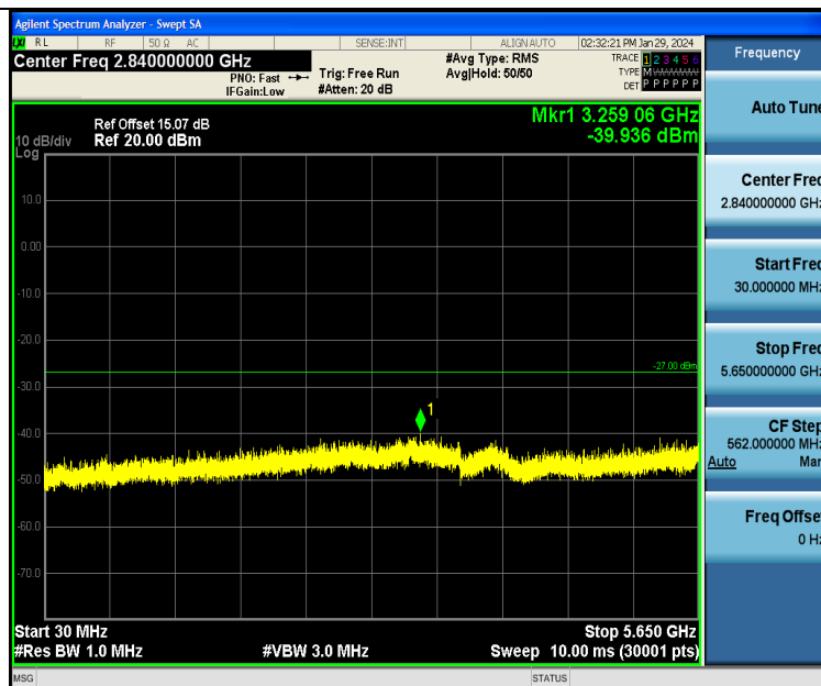
11A-Ant1-5785-30~5650-PASS
