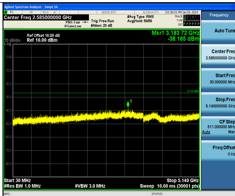
11AC20SISO-Ant1-5240-30~5140-PASS
