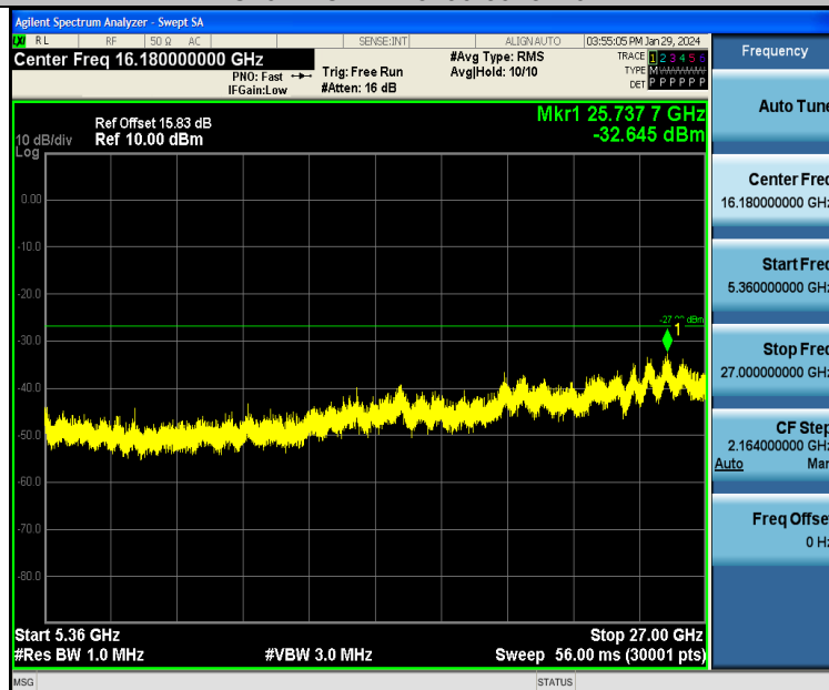
11AC40SISO-Ant1-5190-5360~27000-PASS
