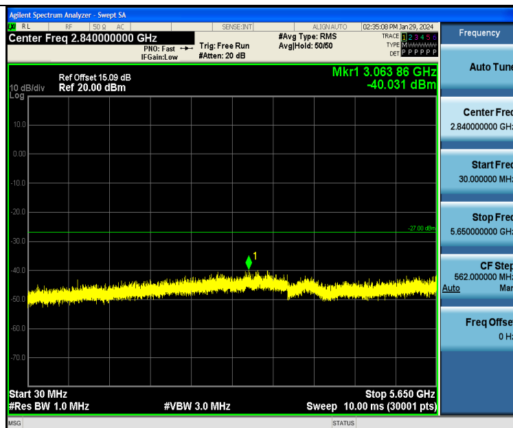
11A-Ant1-5825-30~5650-PASS
