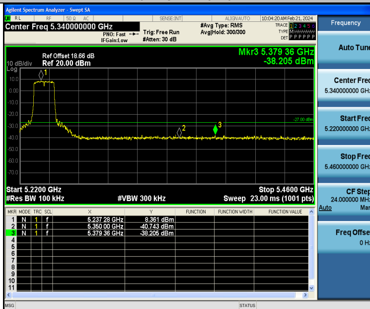
11A20SISO-Ant1-5240-PASS
