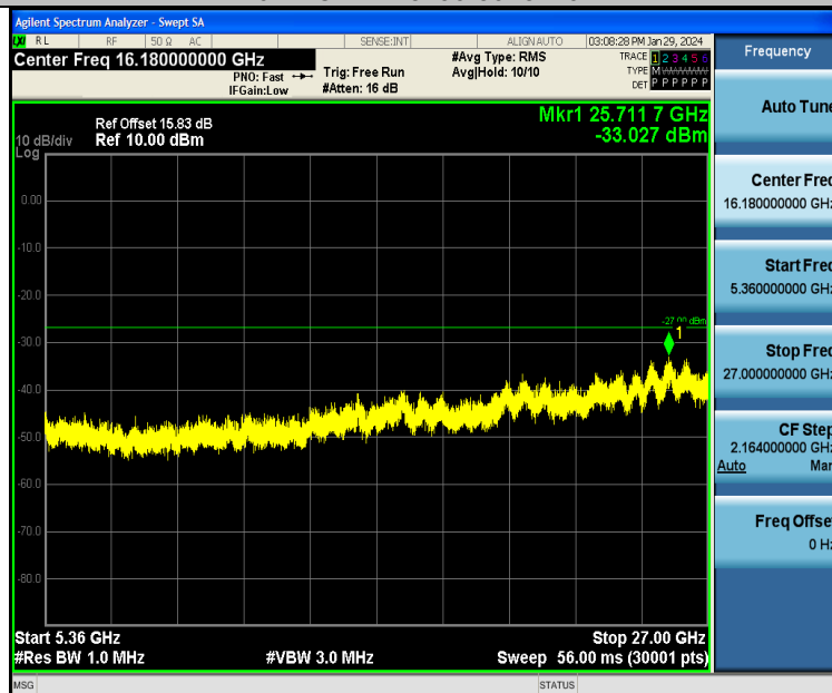
11N40SISO-Ant1-5190-5360~27000-PASS
