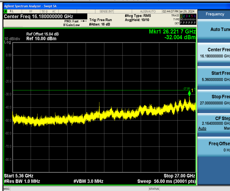
11N20SISO-Ant1-5200-5360~27000-PASS
