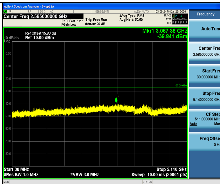
11N40SISO-Ant1-5190-30~5140-PASS
