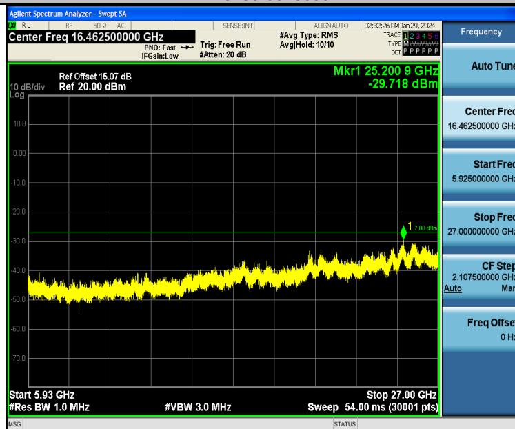
11A-Ant1-5785-5925~27000-PASS
