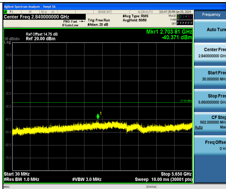
11AC20SISO-Ant1-5745-30~5650-PASS
