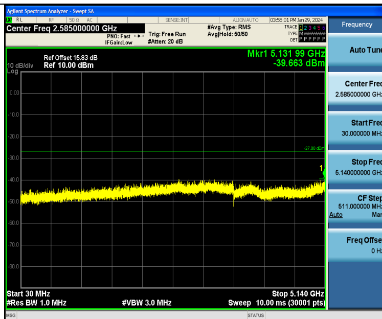
11AC40SISO-Ant1-5190-30~5140-PASS
