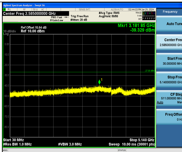
11N20SISO-Ant1-5200-30~5140-PASS
