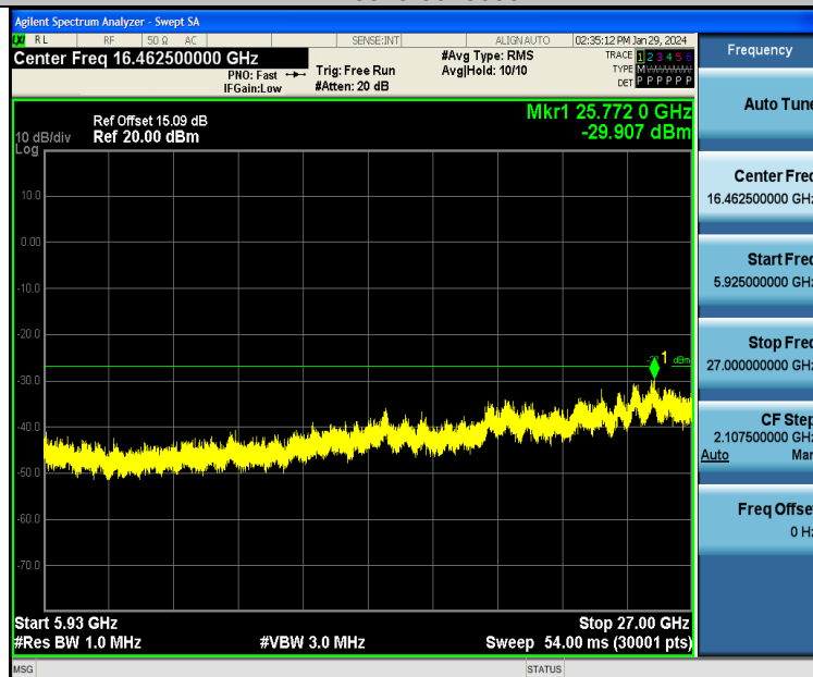
11A-Ant1-5825-5925~27000-PASS
