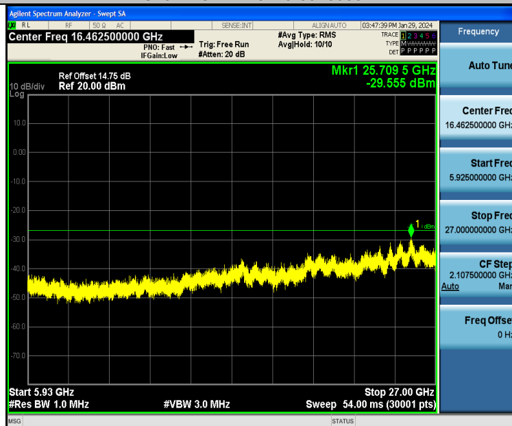
11AC20SISO-Ant1-5745-5925~27000-PASS
