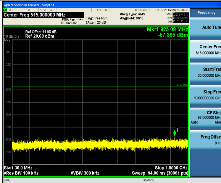
11N20SISO-Ant1-2462-30~1000-PASS
