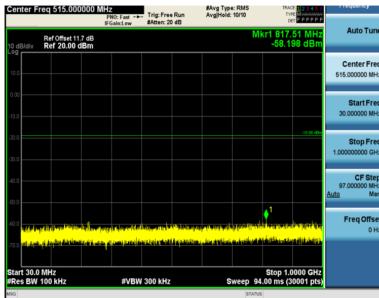
BLE_1M-Ant1-2480-30~1000-PASS
