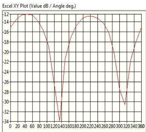
2.485GHz@Theta 0.0 Horizontal
