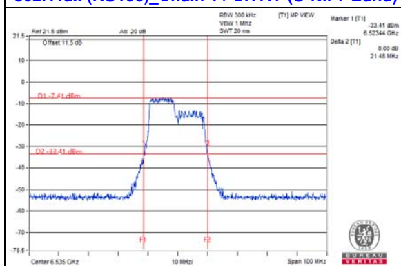
802.11ax (RU106)_Chain 1 / CH117 (U-NII-7 Band)
