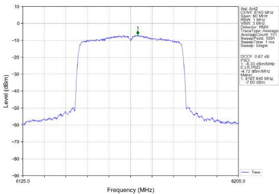
802.11ax(HEW40)_MCH_6165MHz_SU_Ant2_NTNV
