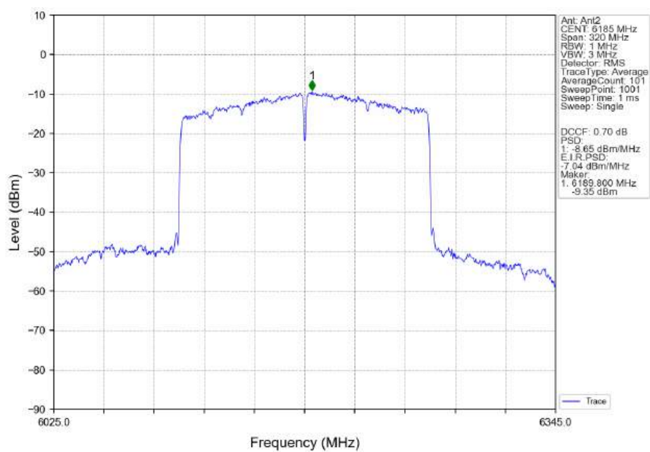
802.11ax(HEW160)_MCH_6185MHz_SU_Ant2_NTNV
