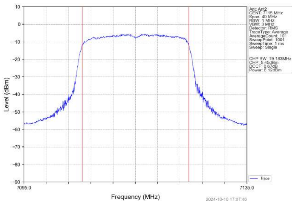
802.11ax(HEW20)_HCH_7115MHz_SU_Ant2_NTNV
