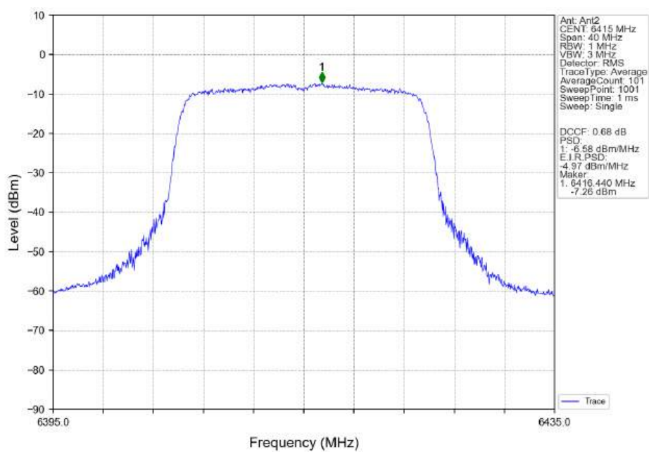
802.11ax(HEW20)_HCH_6415MHz_SU_Ant2_NTNV
