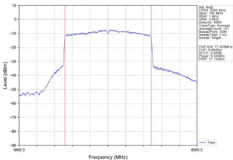
802.11ax(HEW80) LCH_5985MHz_SU_Ant2_NTNV
