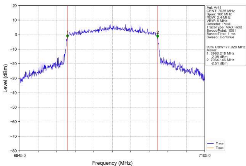
802.11ax(HEW80) HCH_7025MHz_SU_Ant1_NTNV
