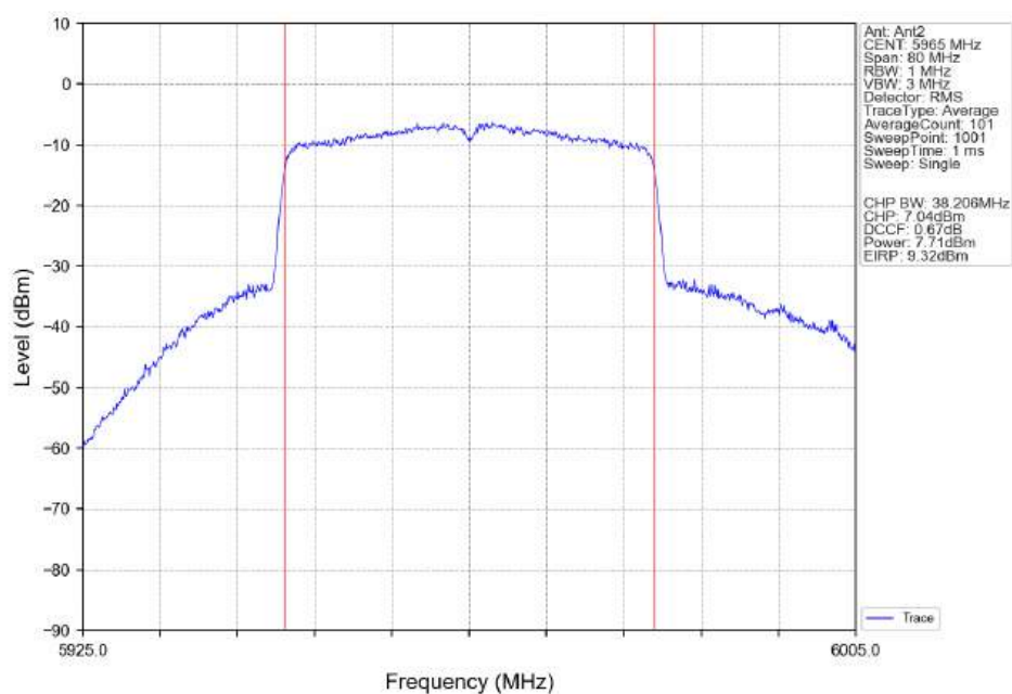
802.11ax(HEW40) LCH_5965MHz_SU_Ant2_NTNV
