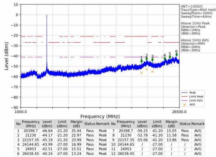
802.11a_LCH_5180MHz_Ant1_NTNV
