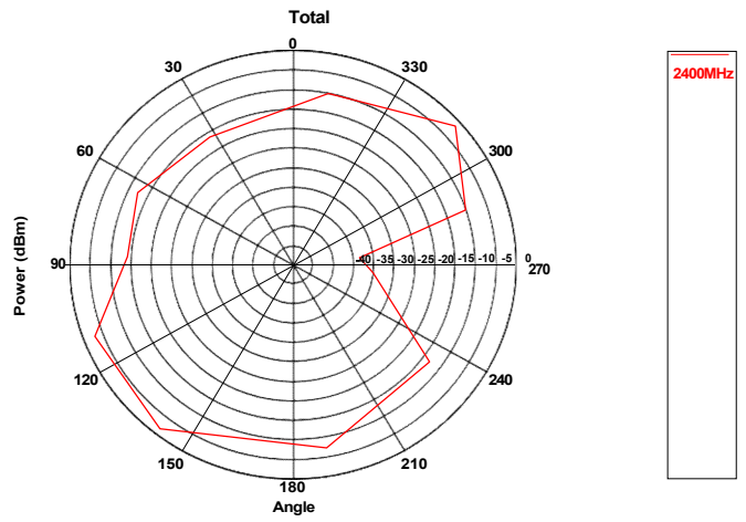
XY Plane at f = 2.400GHz
