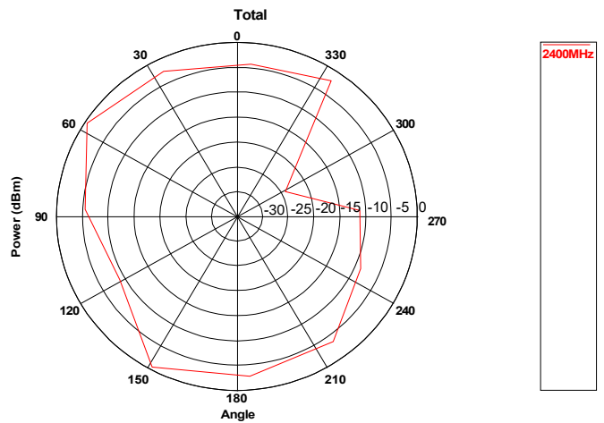
XZ Plane at f = 2.400GHz
