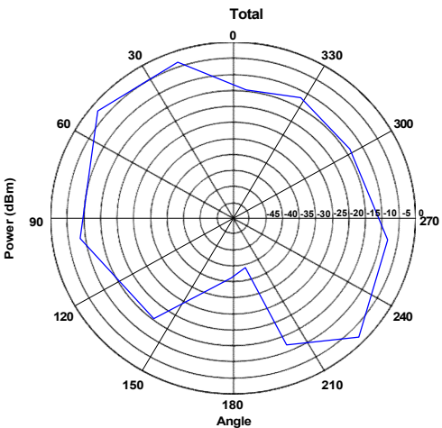
XY Plane at F = 2.500GHz
