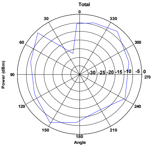
YZ Plane at Freq = 2.500GHz
